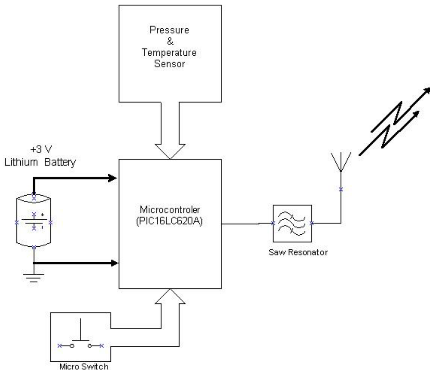
Transmitter(Sensor Module) Block Diagram
