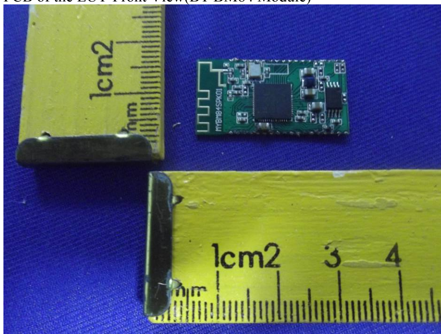
Figure 7 PCB of the EUT-Front View(BT BM84 Module)
