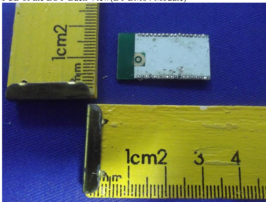
Figure 8 PCB of the EUT-Back View(BT BM84 Module)
