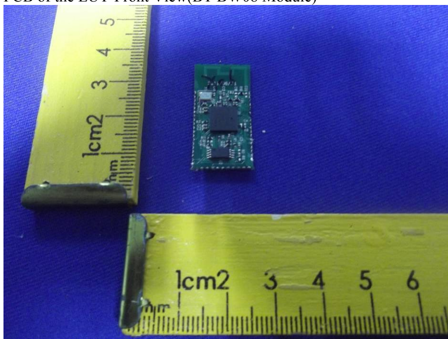
Figure 9 PCB of the EUT-Front View(BT BW08 Module)
