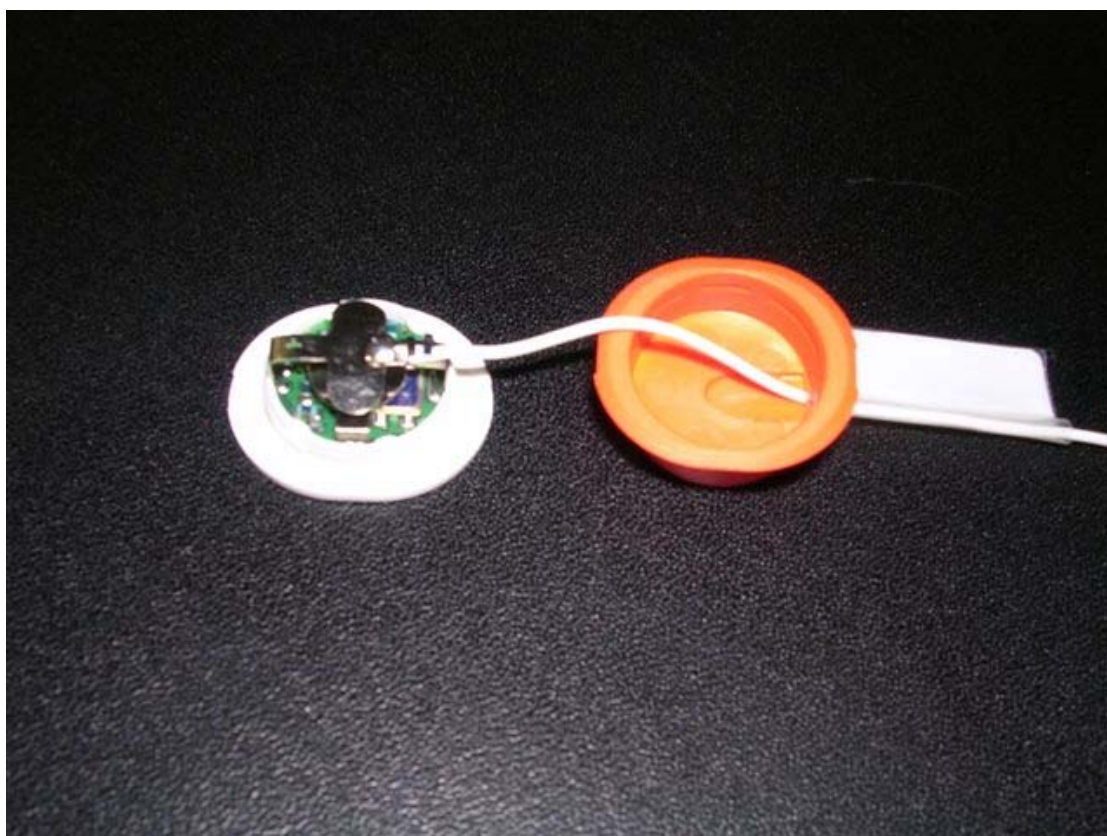
MICRA-G Showing Antenna Soldered to Battery Clip
