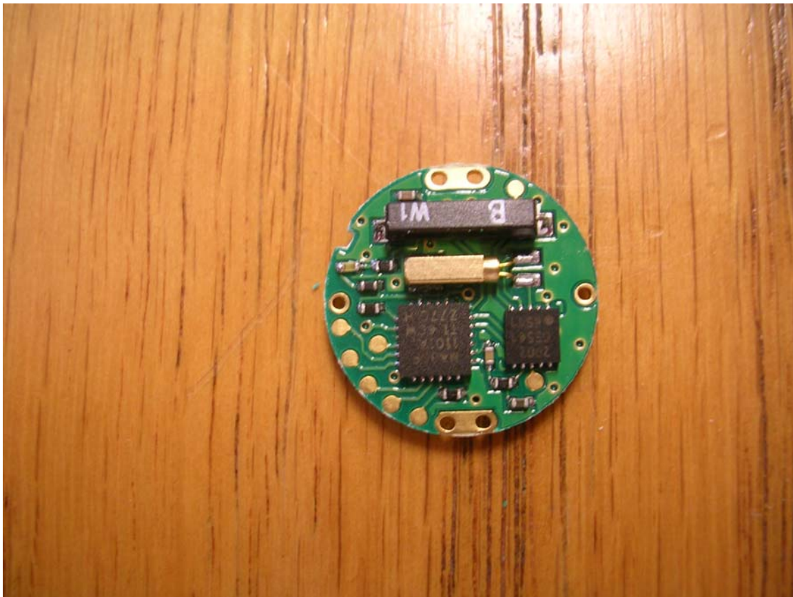
MICRA-G PCB Assembly Top Side
