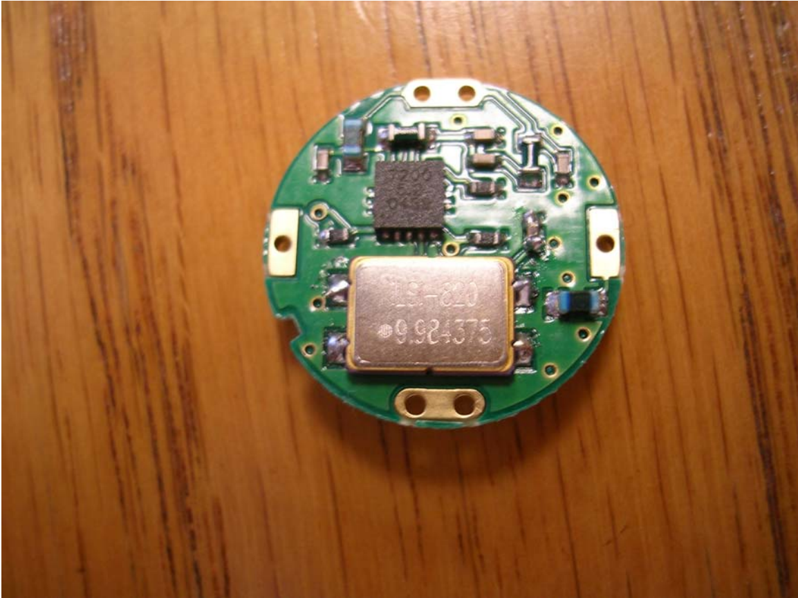
MICRA-G PCB Assembly Bottom Side
