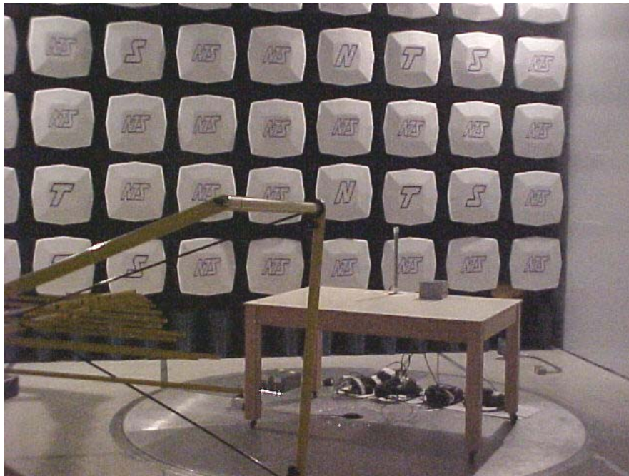
Radiated Emissions 30Mhz-1Ghz With one antenna and three 75 ohms terminations inside anechoic chamber at FM radio frequencies range
