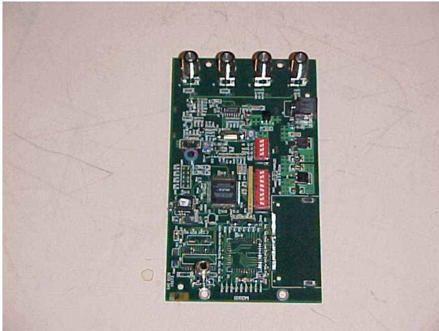
Close Look at the front IMI-3000L Transmit card
