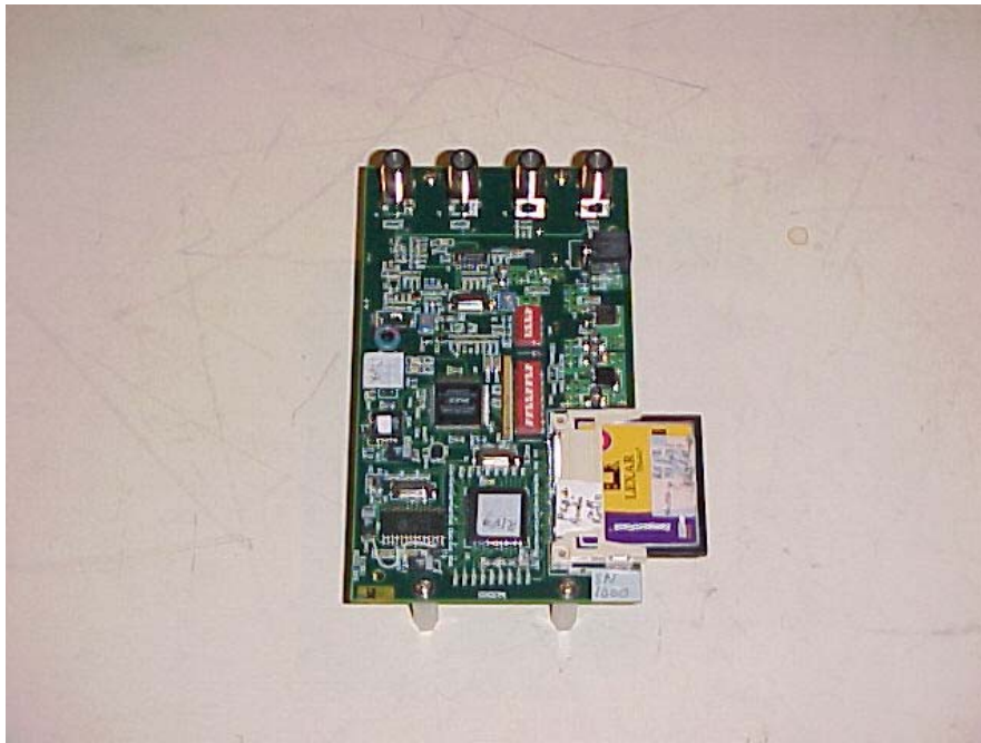
Close Look at the front IMI-3000 Transmit card.
