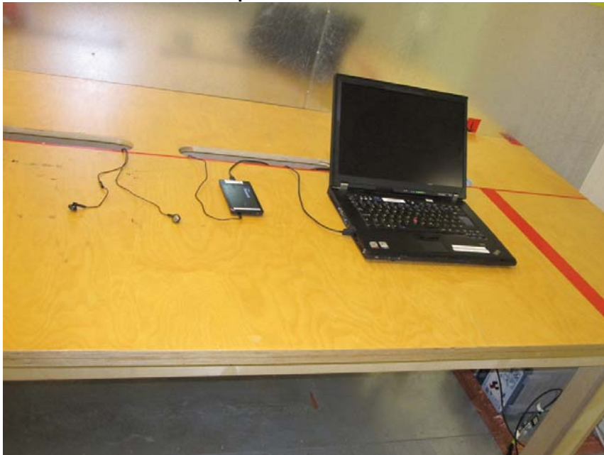
Picture 5. FCC Part 15B AC powerline conducted emissions
