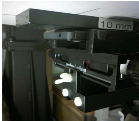
Photo of the device positioned for WR mode measurement –back facing phantom. The spacer was removed before the start of the measurements.
