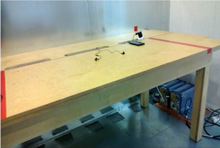
Picture 5. FCC Part 15B AC powerline conducted emissions
