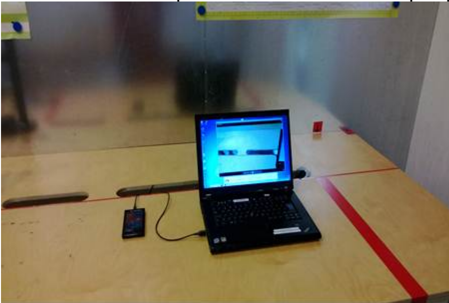
Picture 4. FCC Part 15C AC powerline conducted emissions computer peripherals
