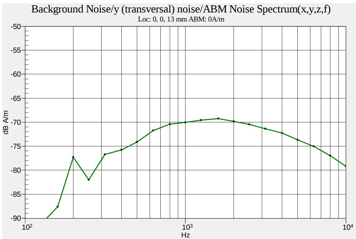
Figure 21: Ambient Background Noise Spectrum Plot – Radial Y Orientation
