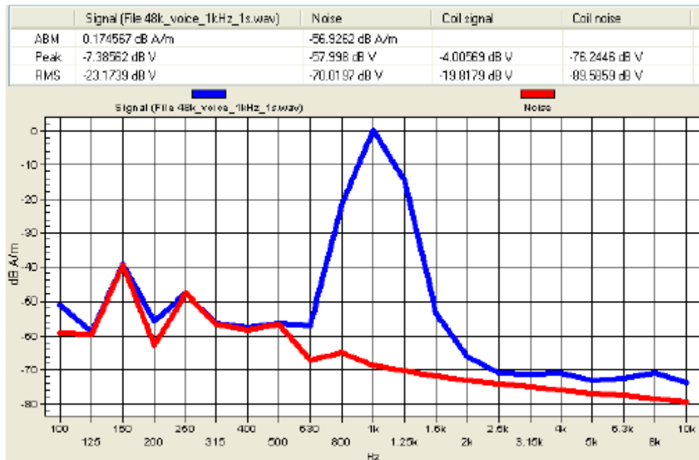
Figure 7: Audio Signal Spectrum of the Narrowband Signal
