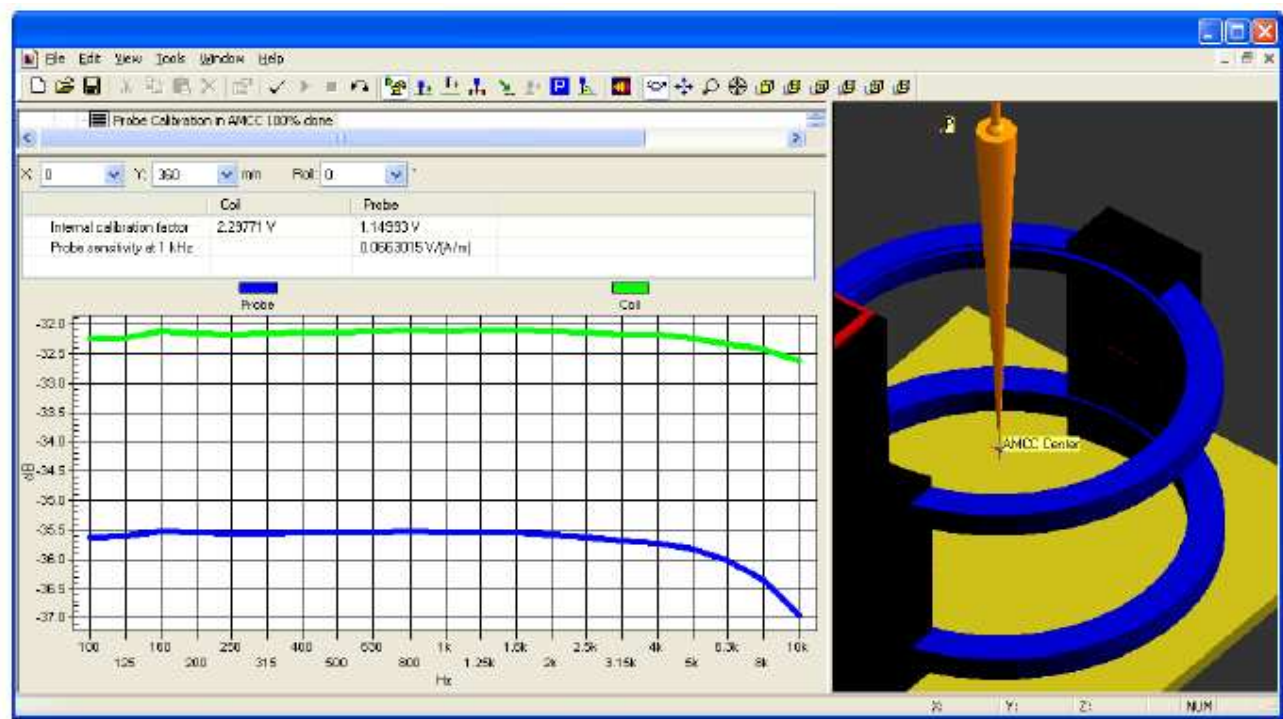
Figure 6: Frequency Response and Sensitivity measured in AMCC
