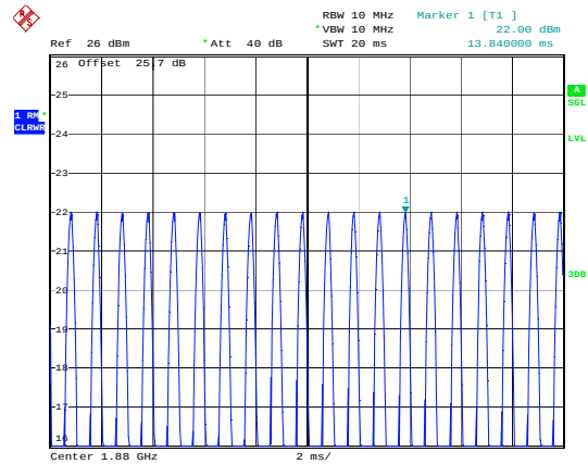
Figure 16: AM – 1880MHz
