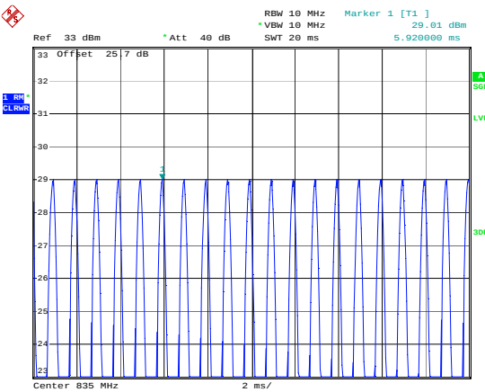
Figure 10: AM – 835MHz
