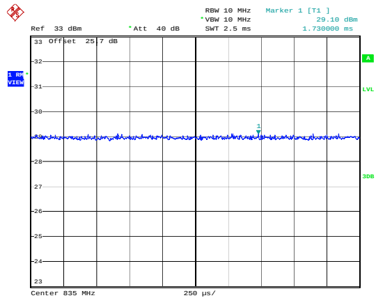
Figure 12: WCDMA – 835MHz
