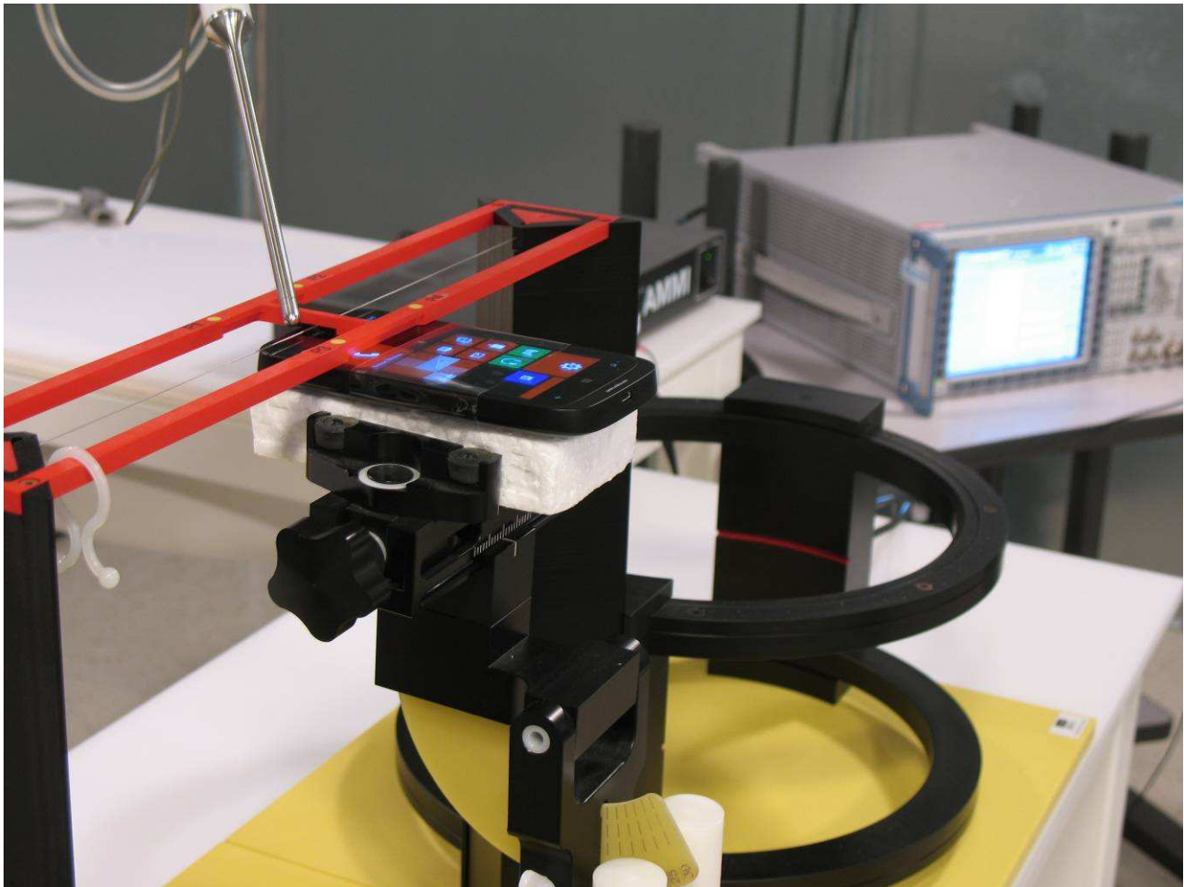
Figure 7: T-Coil Test Setup Photograph
