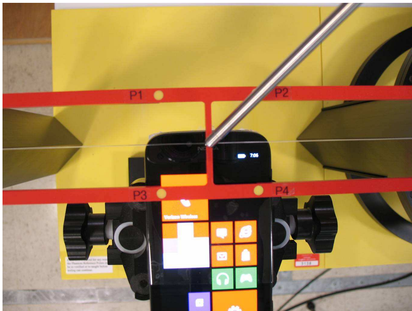
Figure 6: T-Coil Setup Photograph Showing EUT Centered on Test Arch
