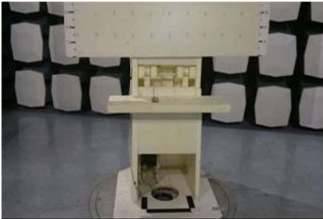
Picture 2. FCC Part 15B Radiated emissions
