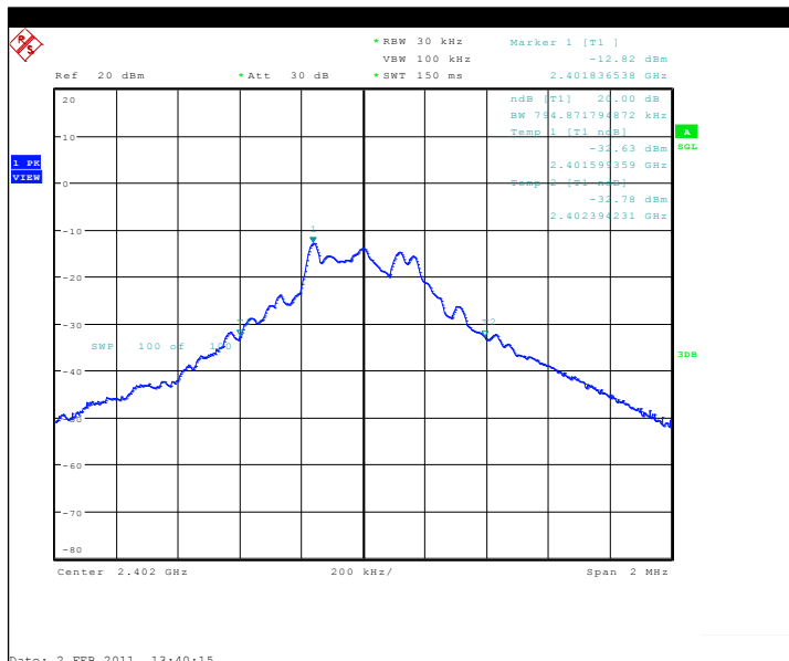
Channel 0 / 2402 MHz
