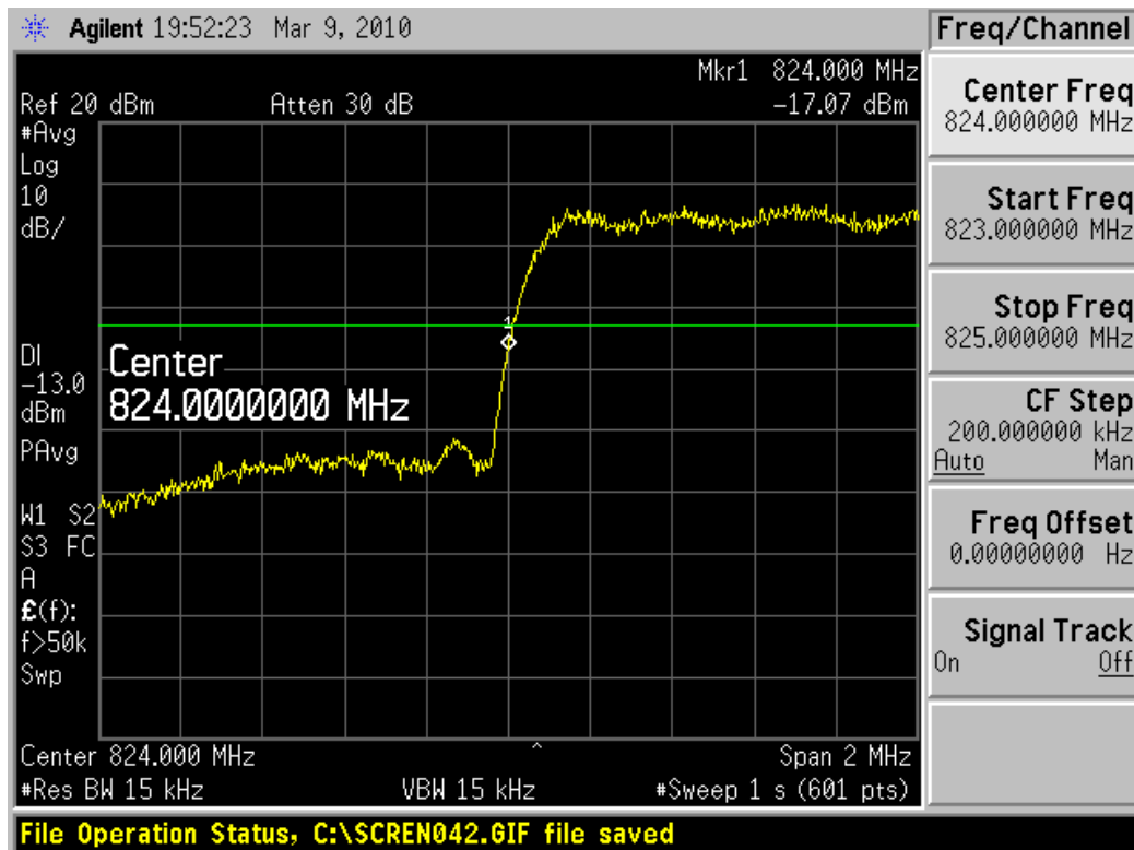
CDMA Cellular 1013 Channel
