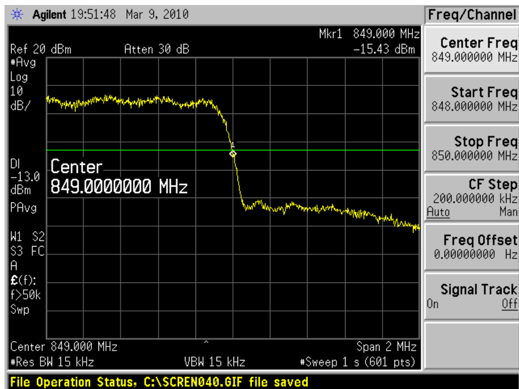
CDMA Cellular 777 Channel
