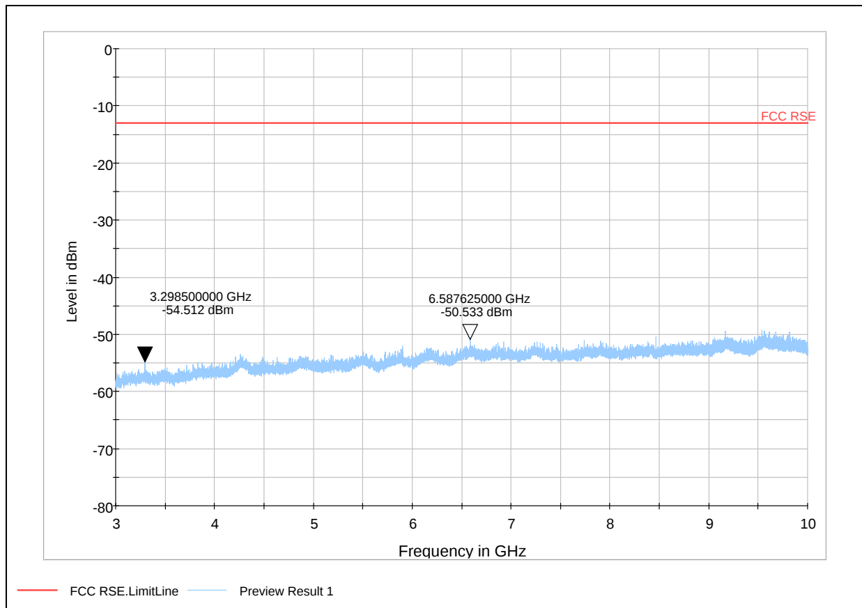
CDMA Cellular Channel1013 3GHz ~10GHz
