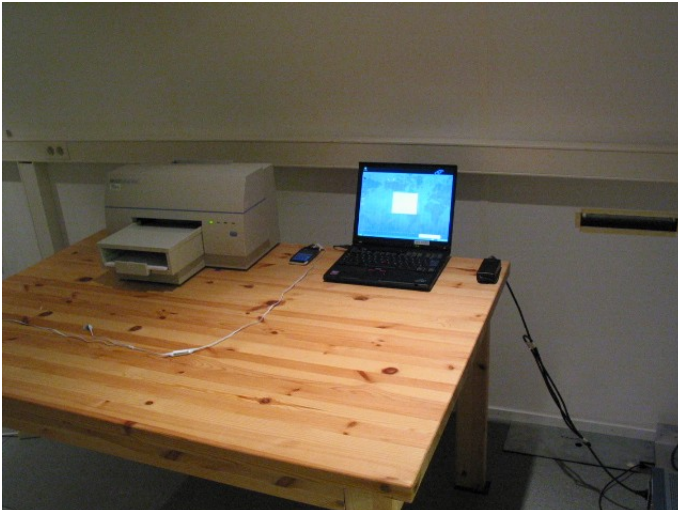
Picture 4. FCC Part 15B AC powerline conducted emissions
