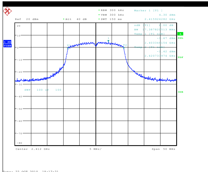
Channel 1 / 2412 MHz
