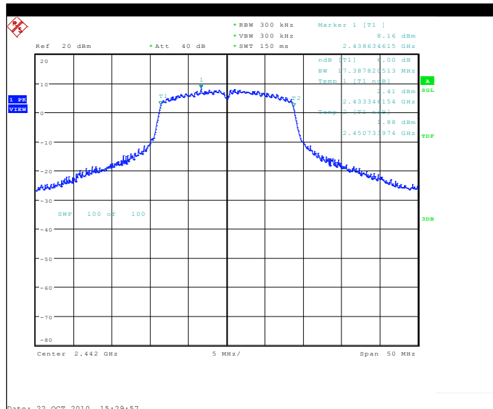
Channel 7 / 2442 MHz
