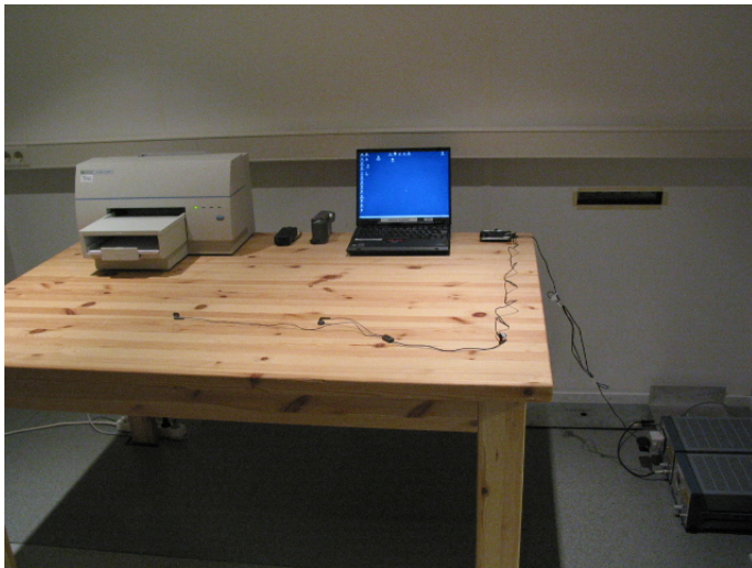
Picture 3 AC powerline conducted emission measurement 15B
