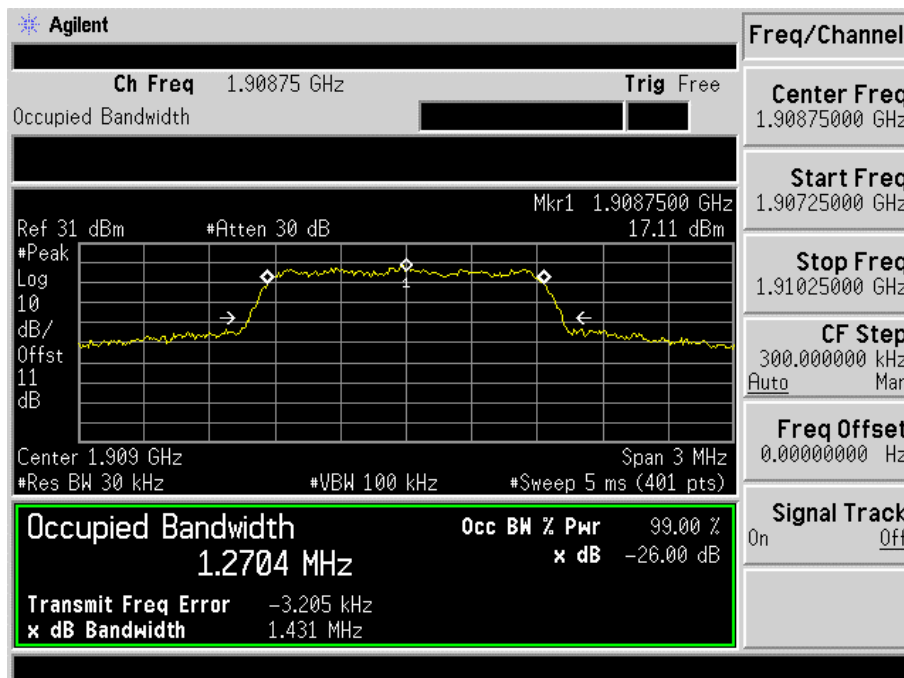
Fig. 3-19 Occupied Bandwidth for mode 6(Ch. 1175).
