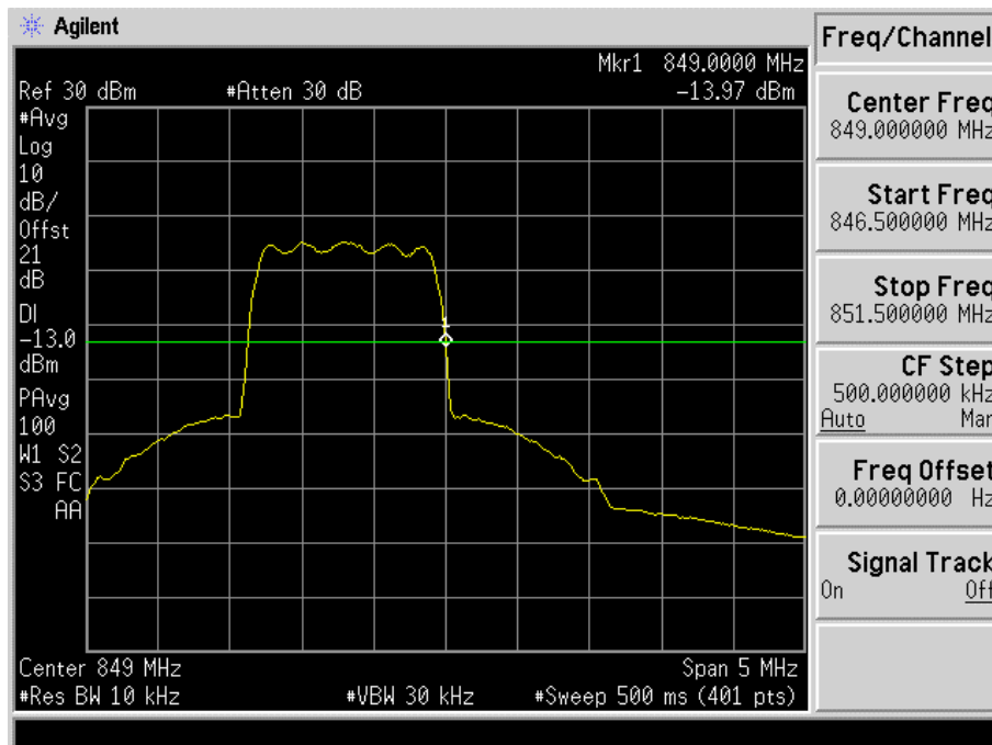
Fig. 4-11 Band edge measurements for mode 5(Ch. 777).
