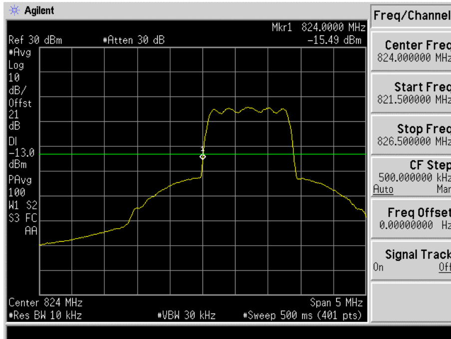
Fig. 4-10 Band edge measurements for mode 5(Ch. 1013).
