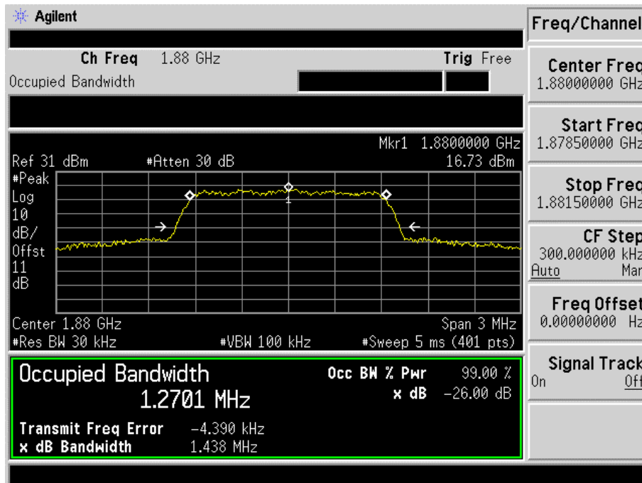
Fig. 3-18 Occupied Bandwidth for mode 6(Ch. 600).
