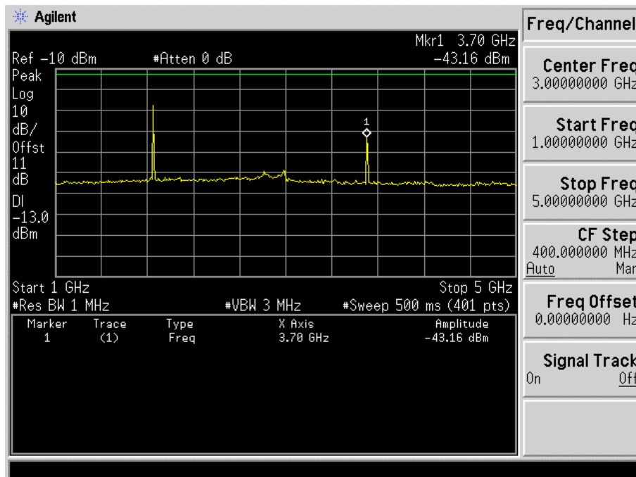
Fig. 5-28(b) Conducted spurious emission for mode 6(Ch. 25).
