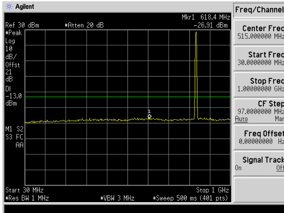
Fig. 5-19(a) Conducted spurious emission for mode 5(Ch. 384).
