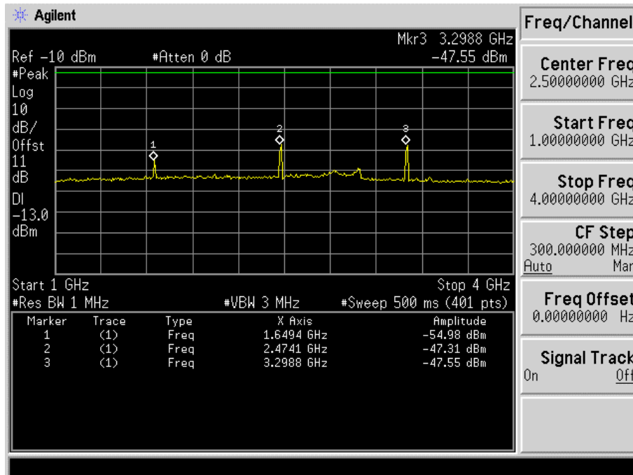
Fig. 5-16(b) Conducted spurious emission for mode 5(Ch. 1013).
