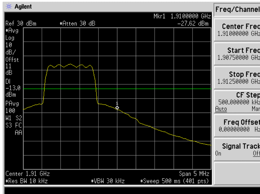
Fig. 4-13 Band edge measurements for mode 6(Ch. 1175).
