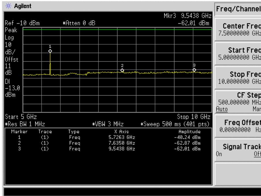
Fig. 5-39(c) Conducted spurious emission for mode 6(Ch. 1175).
