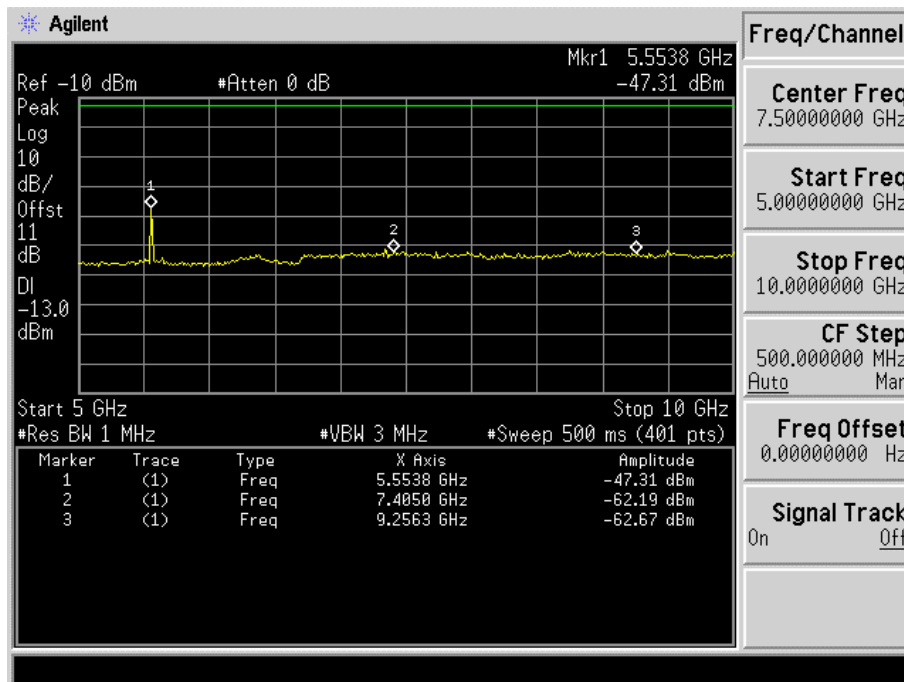
Fig. 5-29(c) Conducted spurious emission for mode 6(Ch. 25).
