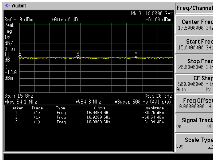
Fig. 5-36(e) Conducted spurious emission for mode 6(Ch. 600).
