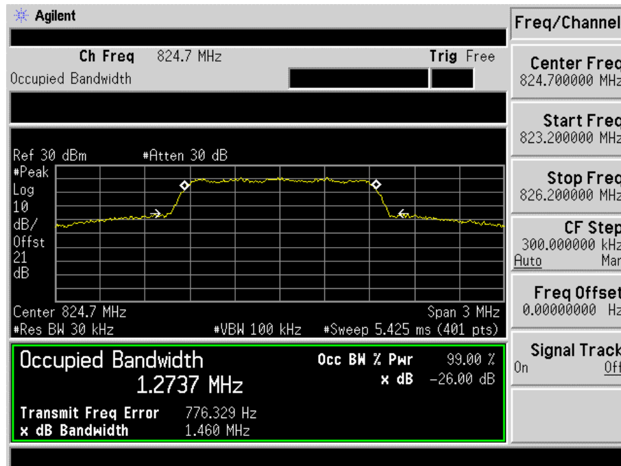
Fig. 3-14 Occupied Bandwidth for mode 5(Ch. 1013).
