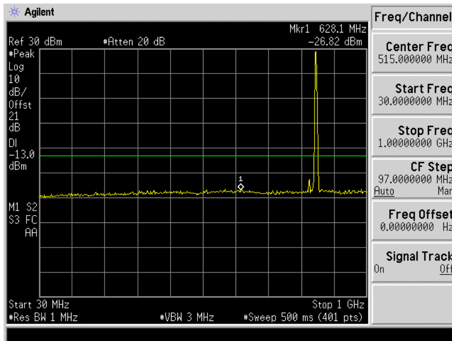
Fig. 5-23(a) Conducted spurious emission for mode 5(Ch. 777).
