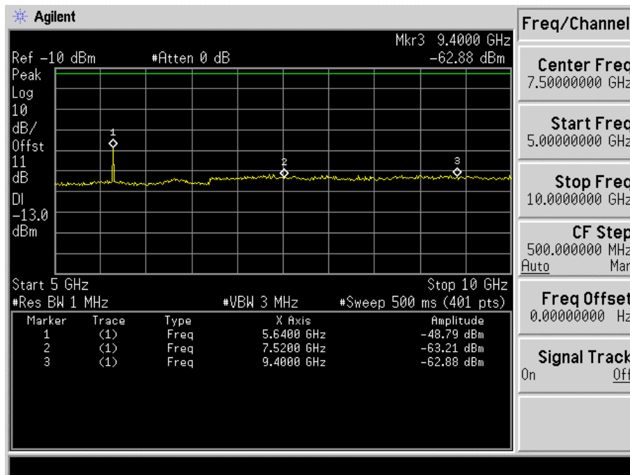
Fig. 5-34(c) Conducted spurious emission for mode 6(Ch. 600).
