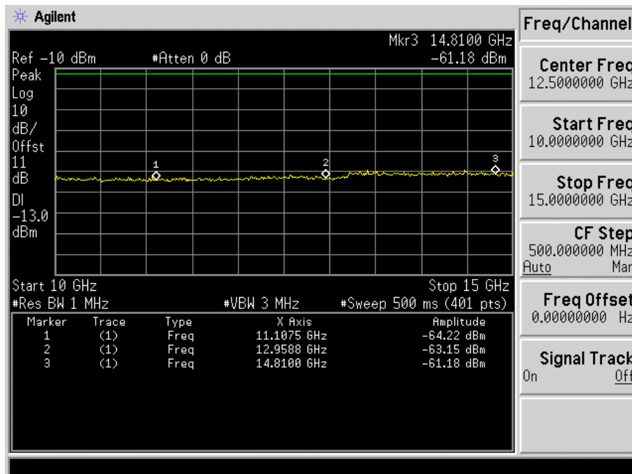
Fig. 5-30(d) Conducted spurious emission for mode 6(Ch. 25).
