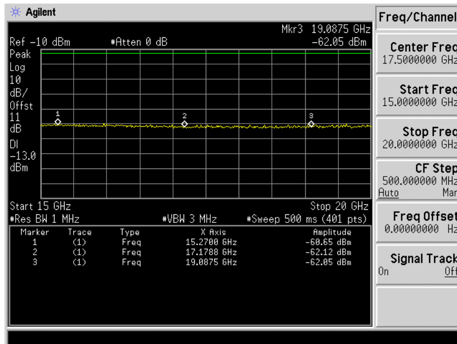
Fig. 5-41(e) Conducted spurious emission for mode 6(Ch. 1175).
