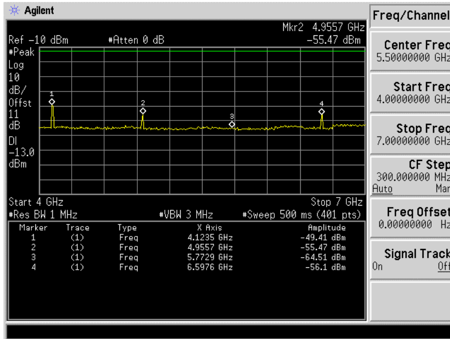
Fig. 5-17(c) Conducted spurious emission for mode 5(Ch. 1013).
