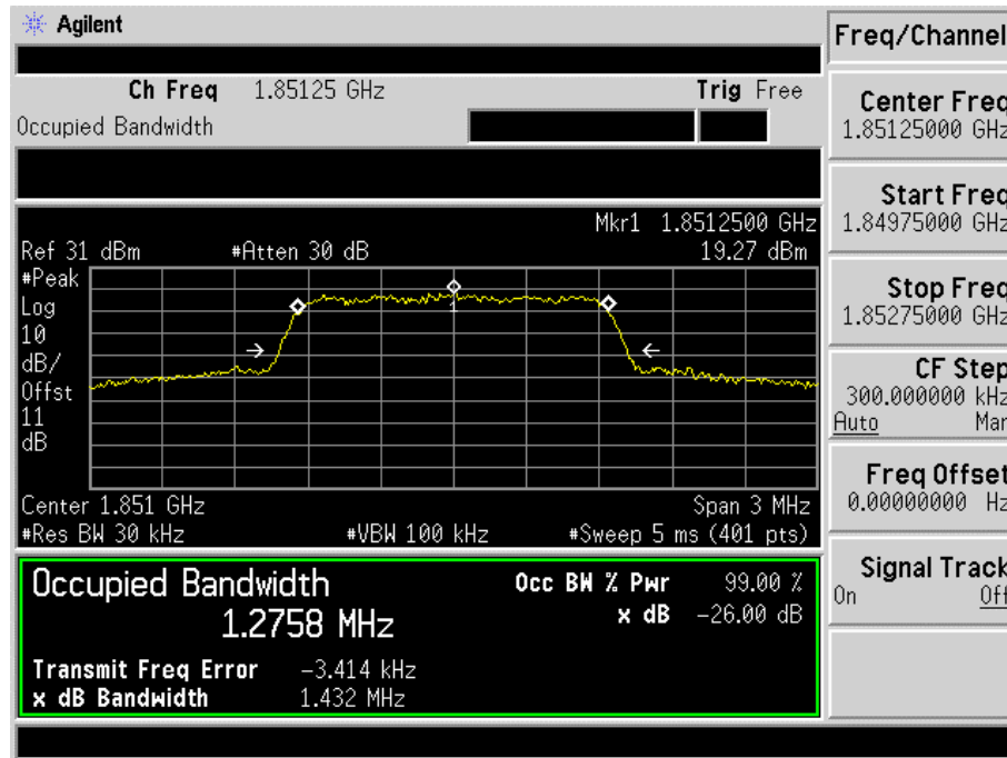
Fig. 3-17 Occupied Bandwidth for mode 6(Ch. 25).
