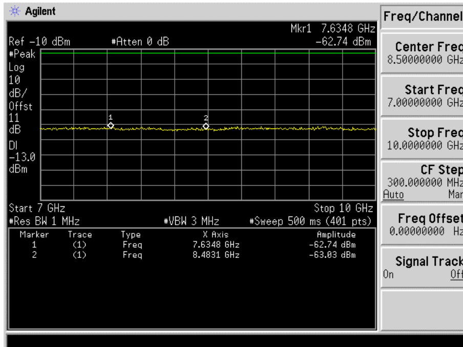
Fig. 5-26(d) Conducted spurious emission for mode 5(Ch. 777).
