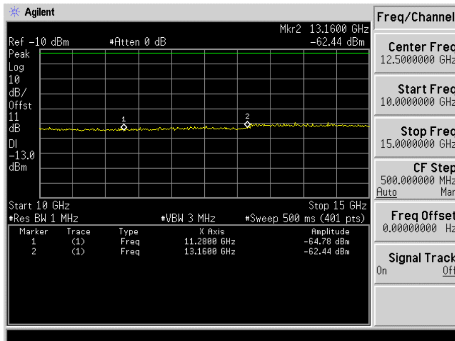
Fig. 5-35(d) Conducted spurious emission for mode 6(Ch. 600).
