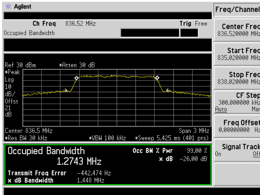
Fig. 3-15 Occupied Bandwidth for mode 5(Ch. 384).
