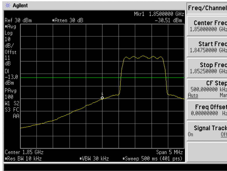
Fig. 4-12 Band edge measurements for mode 6(Ch. 25).
