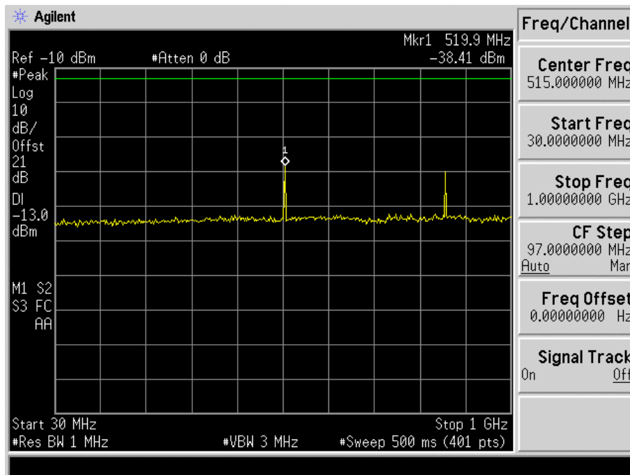
Fig. 5-32(a) Conducted spurious emission for mode 6(Ch. 600).
