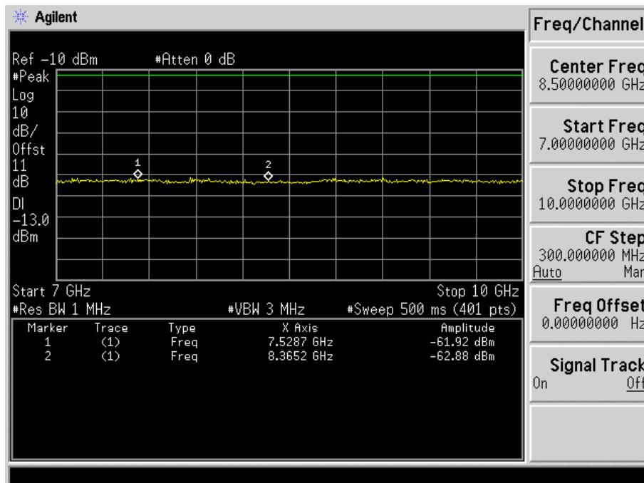
Fig. 5-22(d) Conducted spurious emission for mode 5(Ch. 384).
