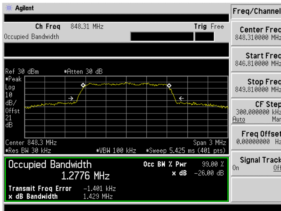
Fig. 3-16 Occupied Bandwidth for mode 5(Ch. 777).
