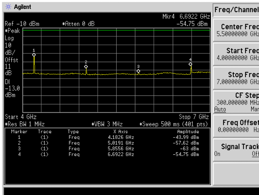
Fig. 5-21(c) Conducted spurious emission for mode 5(Ch. 384).
