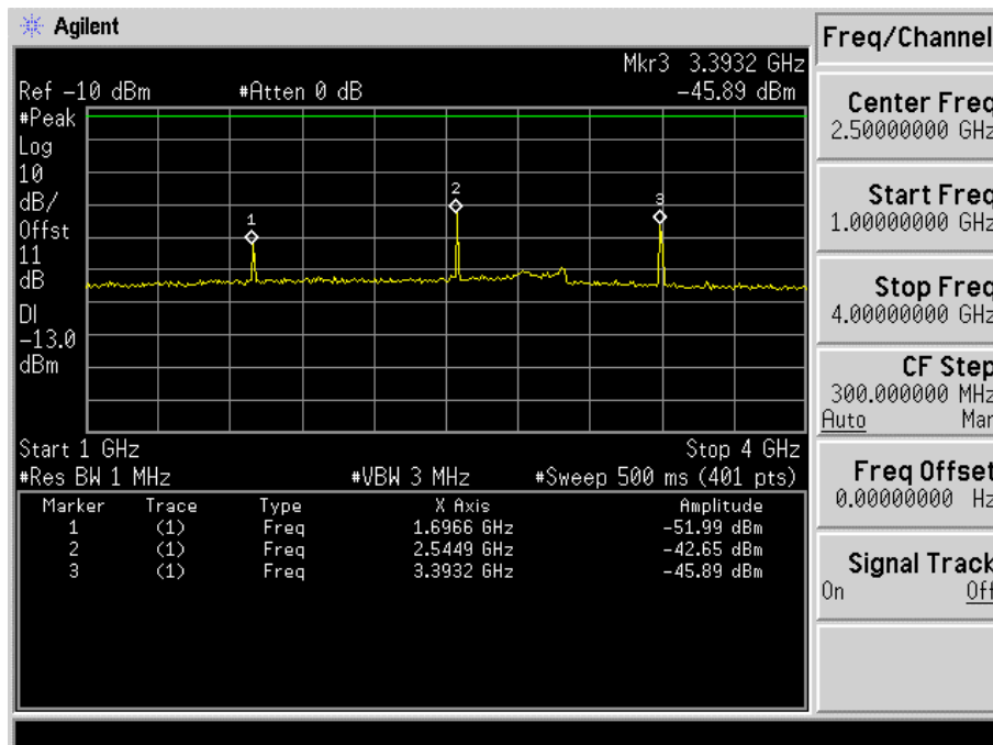
Fig. 5-24(b) Conducted spurious emission for mode 5(Ch. 777).
