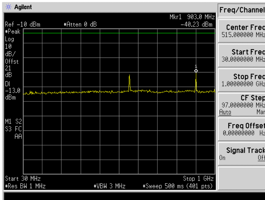
Fig. 5-37(a) Conducted spurious emission for mode 6(Ch. 1175).
