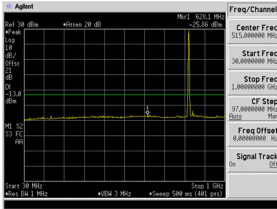
Fig. 5-15(a) Conducted spurious emission for mode 5(Ch. 1013).
