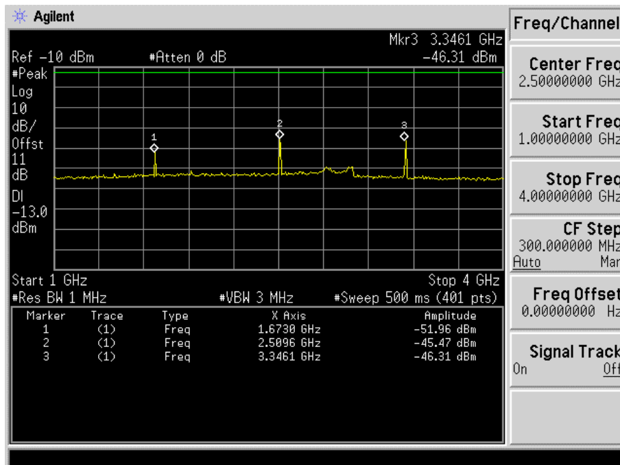
Fig. 5-20(b) Conducted spurious emission for mode 5(Ch. 384).
