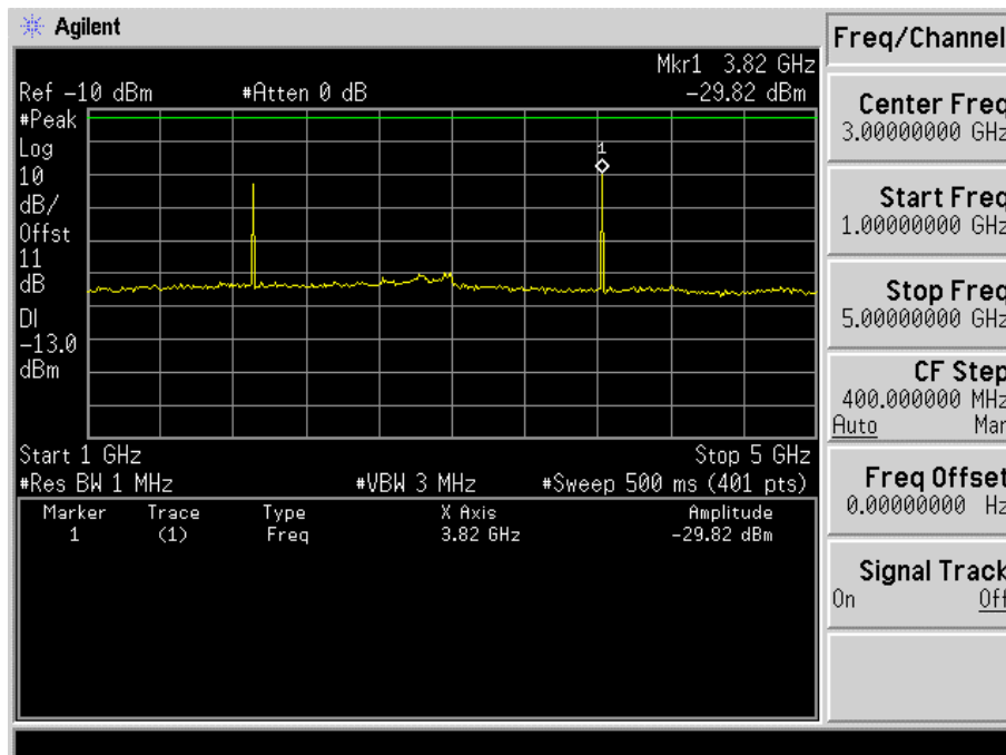
Fig. 5-38(b) Conducted spurious emission for mode 6(Ch. 1175).
