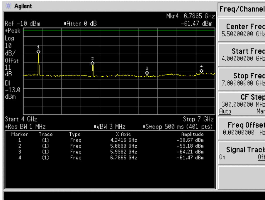
Fig. 5-25(c) Conducted spurious emission for mode 5(Ch. 777).
