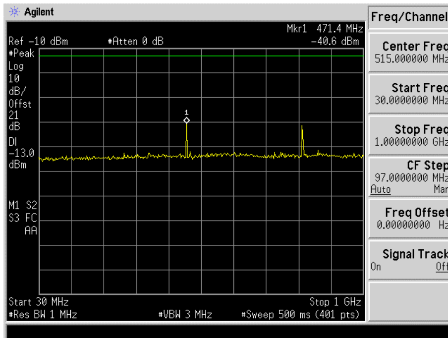
Fig. 5-27(a) Conducted spurious emission for mode 6(Ch. 25).
