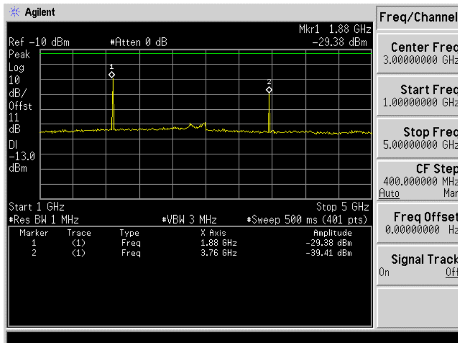
Fig. 5-33(b) Conducted spurious emission for mode 6(Ch. 600).
