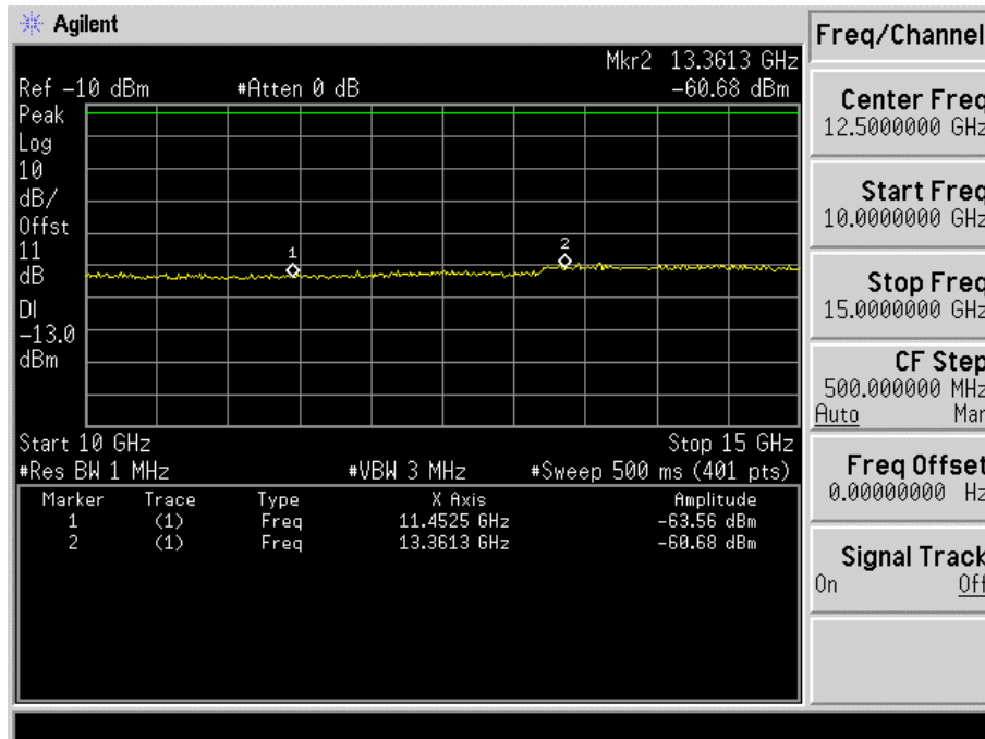
Fig. 5-40(d) Conducted spurious emission for mode 6(Ch. 1175).
