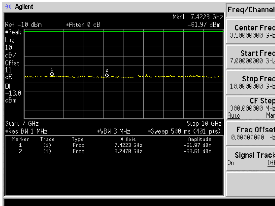
Fig. 5-18(d) Conducted spurious emission for mode 5(Ch. 1013).
