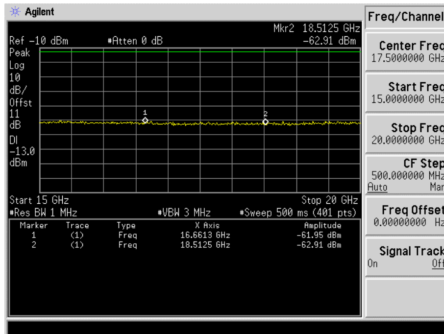
Fig. 5-31(e) Conducted spurious emission for mode 6(Ch. 25).
