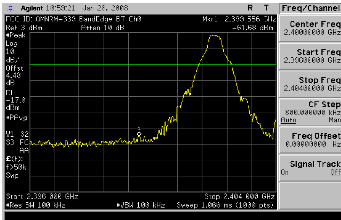
Plot 6-7. Band Edge Plot (Bluetooth (GFSK) – Ch. 0)
