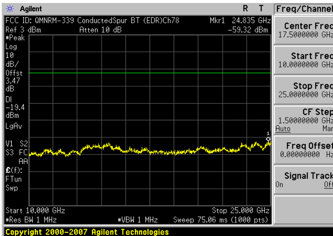
Plot 6-30. Conducted Spurious Plot (Bluetooth 2.0 with Enhanced Data Rate – Ch. 78)
