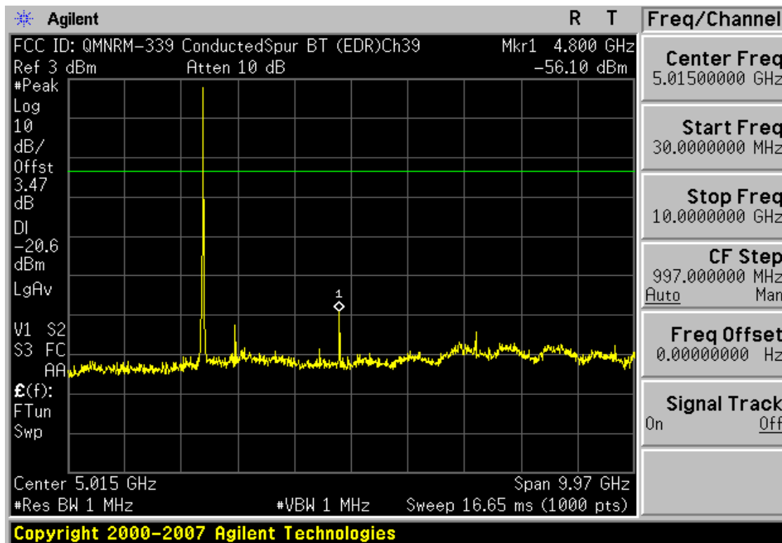
Plot 6-27. Conducted Spurious Plot (Bluetooth 2.0 with Enhanced Data Rate – Ch. 39)
