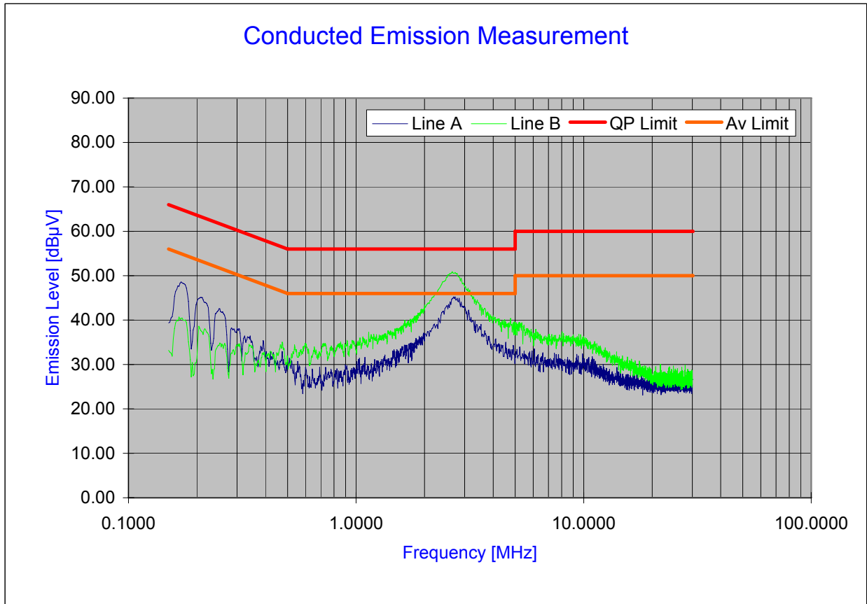
Plot 6-32. Line Conducted Plot with Bluetooth 2.0 with Enhanced Data Rate
