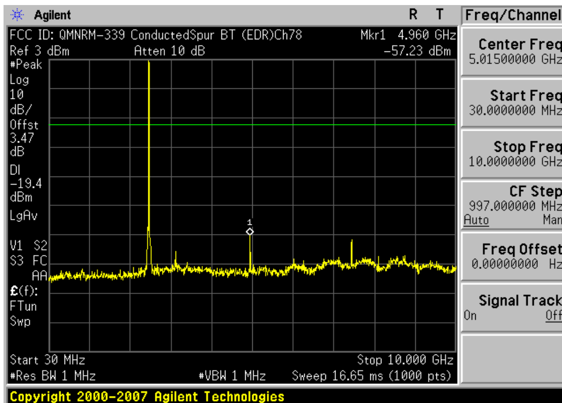
Plot 6-29. Conducted Spurious Plot (Bluetooth 2.0 with Enhanced Data Rate – Ch. 78)
