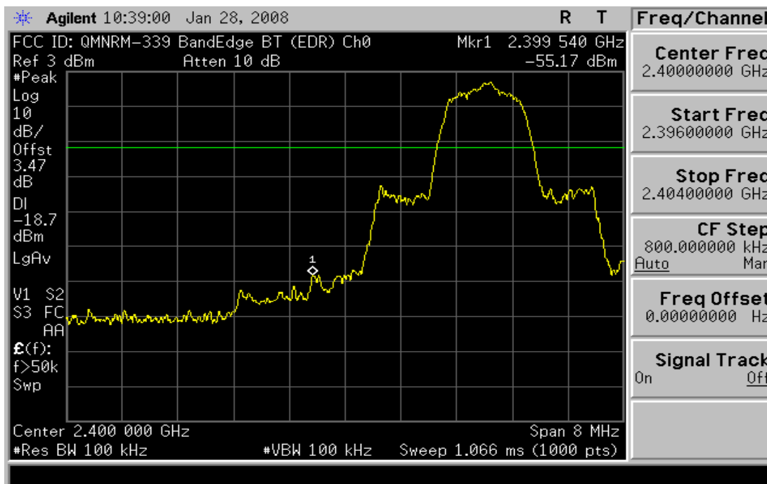
Plot 6-9. Band Edge Plot (Bluetooth 2.0 with Enhanced Data Rate – Ch. 0)
