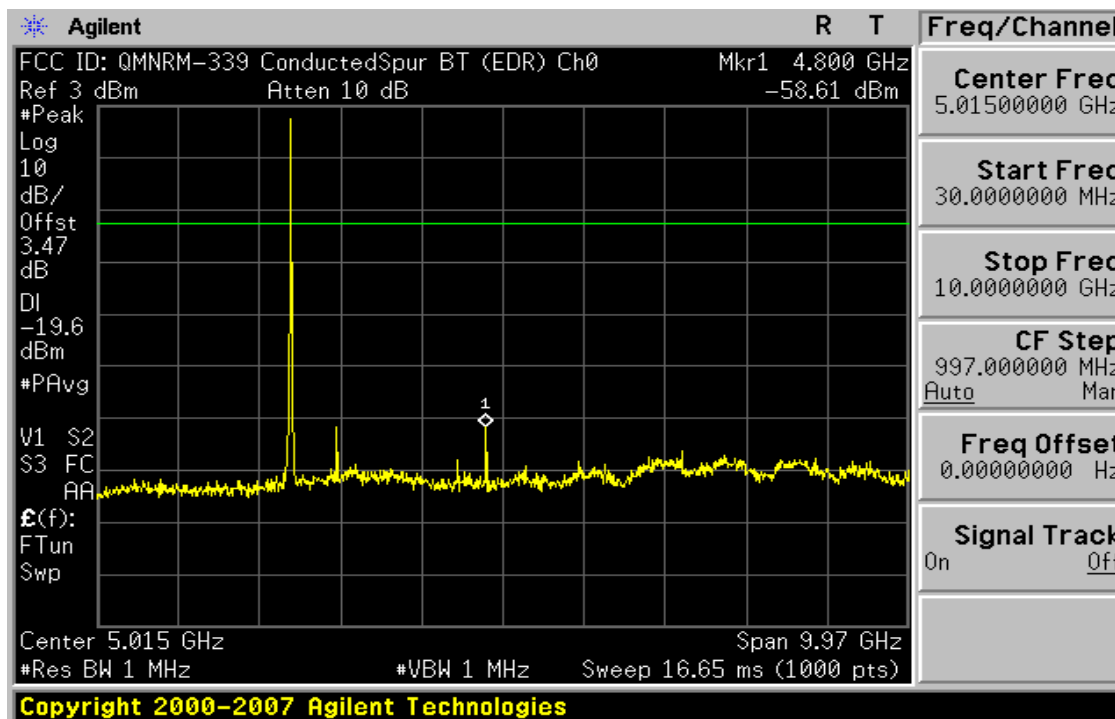
Plot 6-25. Conducted Spurious Plot (Bluetooth 2.0 with Enhanced Data Rate – Ch. 0)
