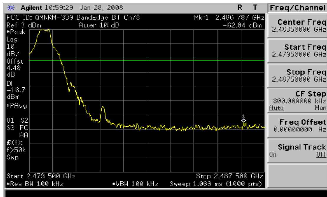
Plot 6-8. Band Edge Plot (Bluetooth (GFSK) – Ch. 78)
