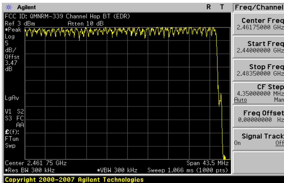
Plot 6-18. High End Spectrum Channel Hopping Plot (Bluetooth 2.0 with Enhanced Data Rate)
