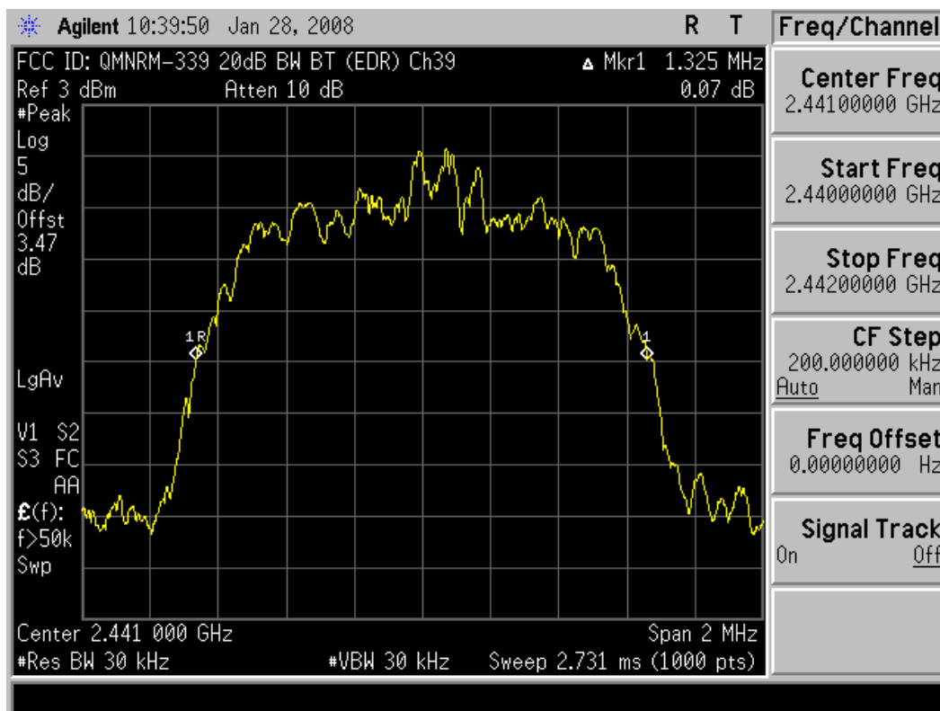
Plot 6-5. 20dB Bandwidth Plot (Bluetooth 2.0 with Enhanced Data Rate – Ch. 39)
