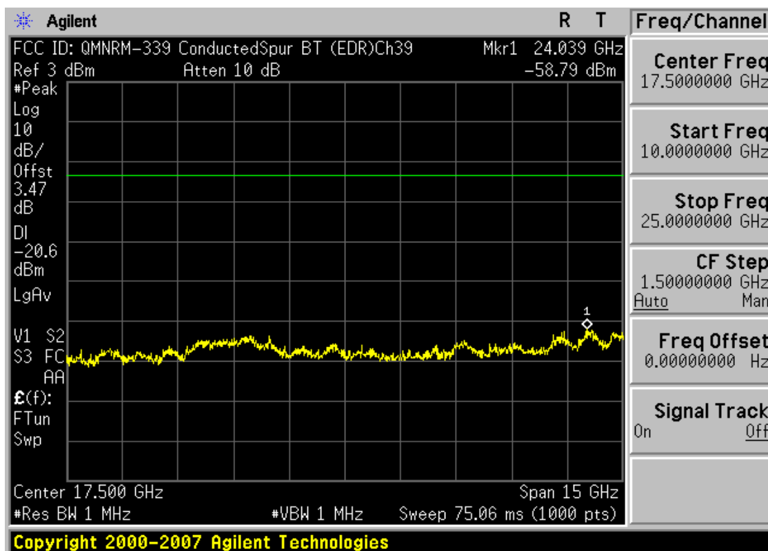
Plot 6-28. Conducted Spurious Plot (Bluetooth 2.0 with Enhanced Data Rate – Ch. 39)
