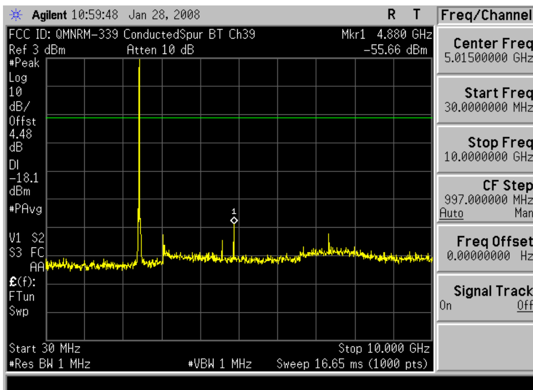
Plot 6-21. Conducted Spurious Plot (Bluetooth (GFSK)– Ch. 39)
