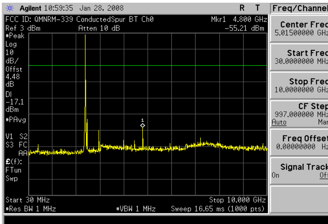
Plot 6-19. Conducted Spurious Plot (Bluetooth (GFSK)– Ch. 0)
