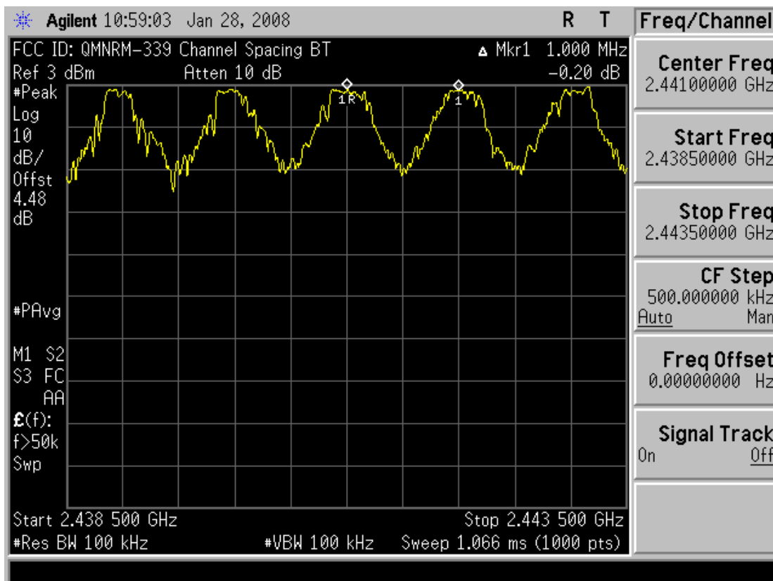
Plot 6-11. Channel Spacing Plot (Bluetooth (GFSK))
