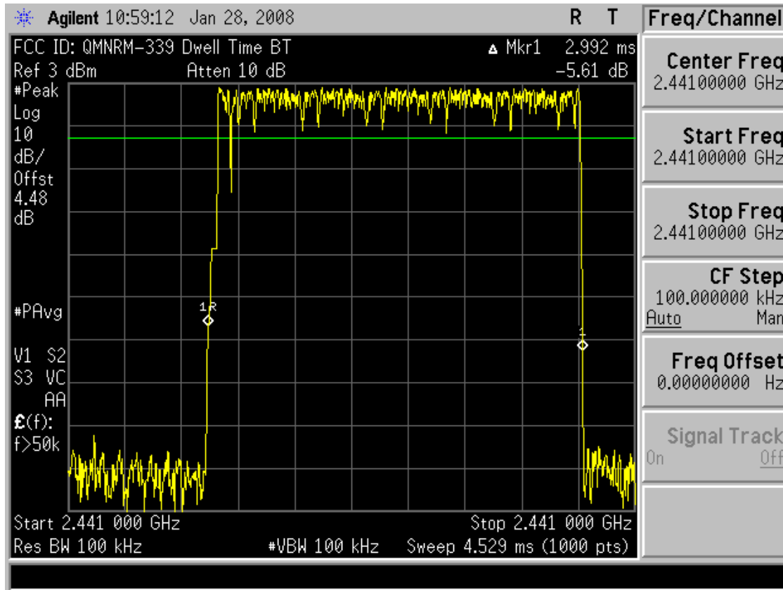
Plot 6-13. Time of Occupancy Plot (Bluetooth (GFSK))
