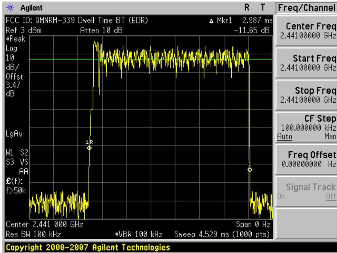
Plot 6-14. Time of Occupancy Plot (Bluetooth 2.0 with Enhanced Data Rate)
