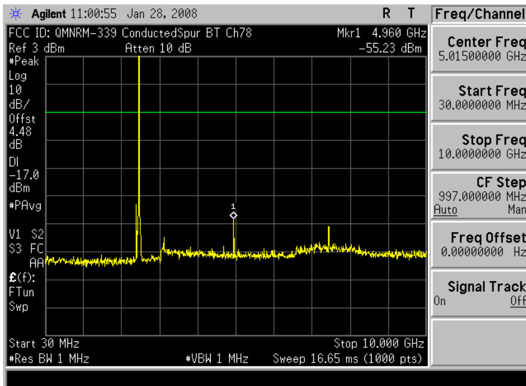
Plot 6-23. Conducted Spurious Plot (Bluetooth (GFSK)– Ch. 78)
