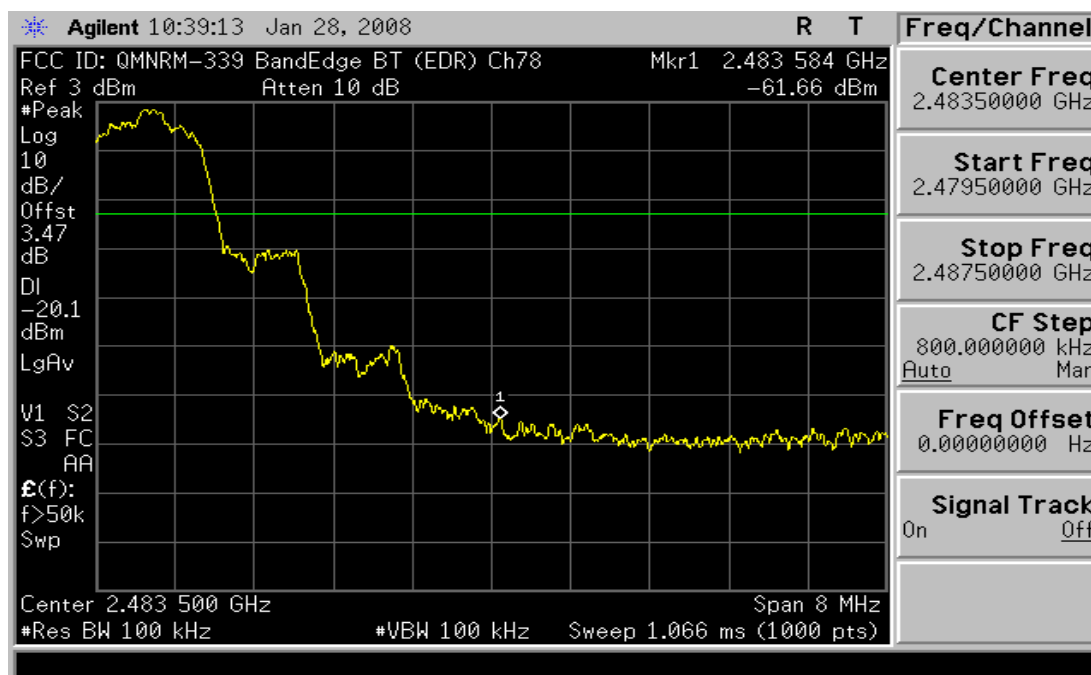
Plot 6-10. Band Edge Plot (Bluetooth 2.0 with Enhanced Data Rate – Ch. 78)
