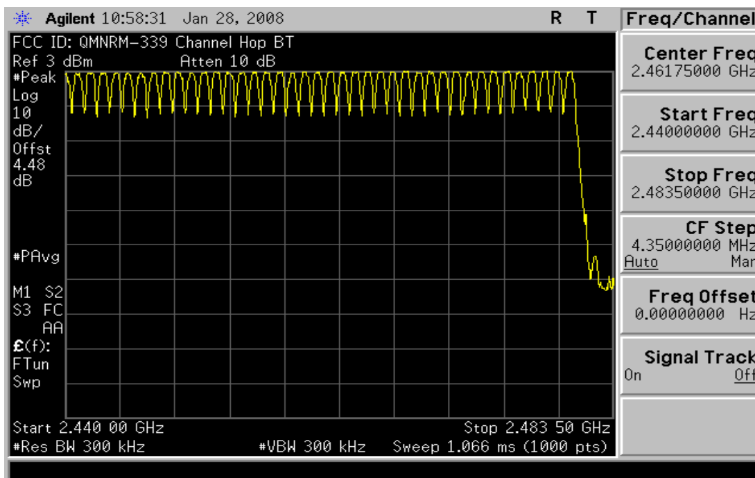
Plot 6-16. High End Spectrum Channel Hopping Plot (Bluetooth (GFSK))
