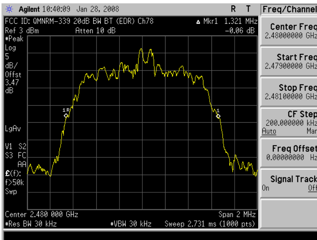
Plot 6-6. 20dB Bandwidth Plot (Bluetooth 2.0 with Enhanced Data Rate – Ch. 78)
