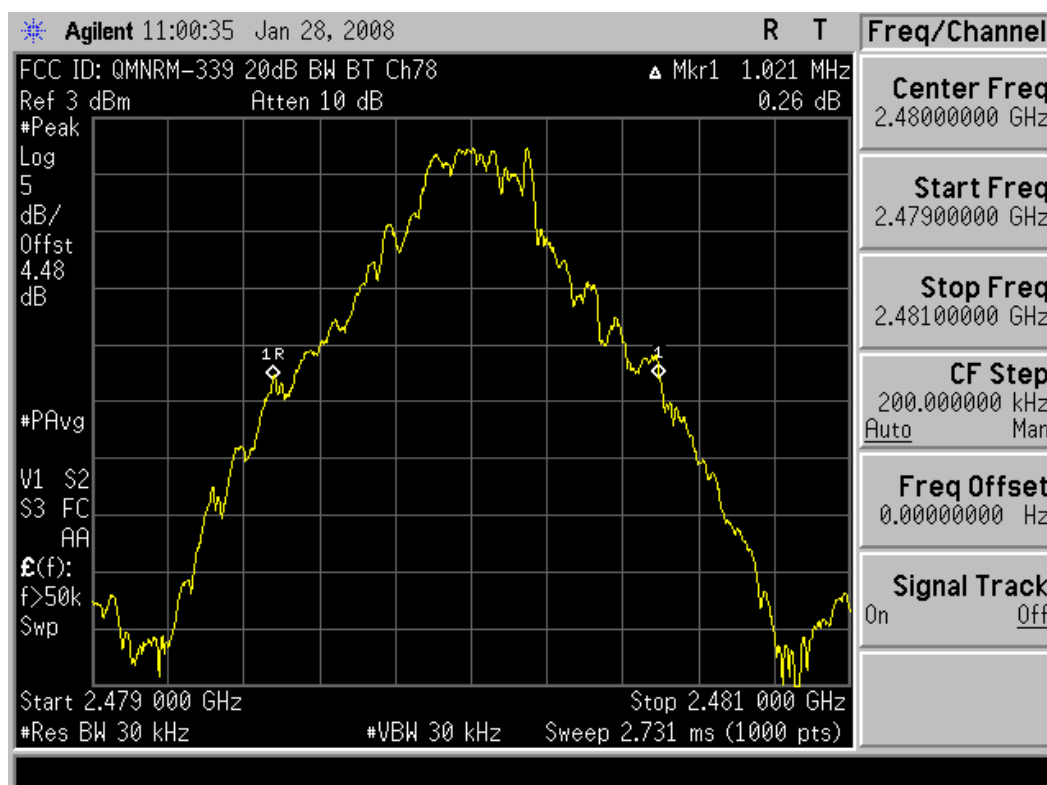
Plot 6-3. 20dB Bandwidth Plot (Bluetooth (GFSK) – Ch. 78)
