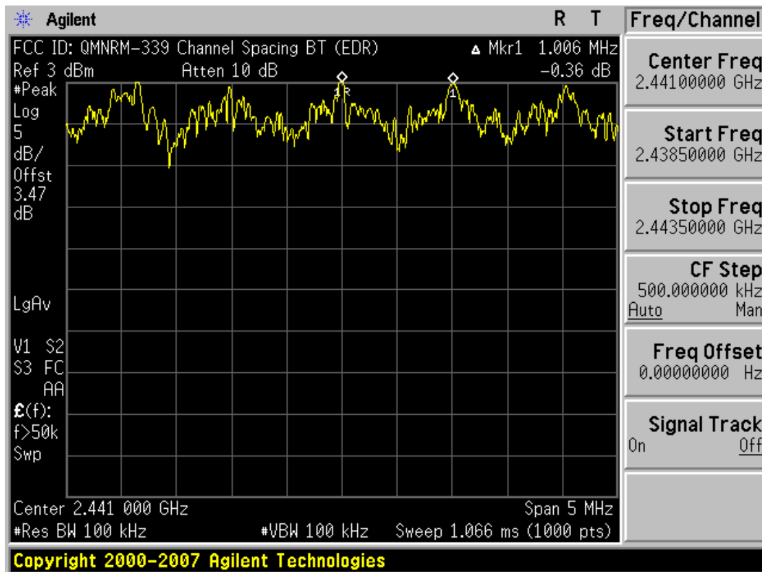
Plot 6-12. Channel Spacing Plot (Bluetooth 2.0 with Enhanced Data Rate)
