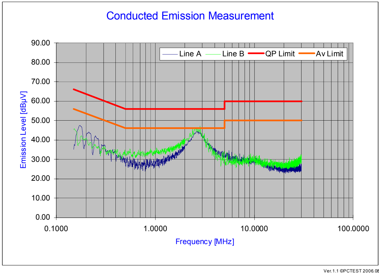
Plot 6-31. Line Conducted Plot with Bluetooth (GFSK)
