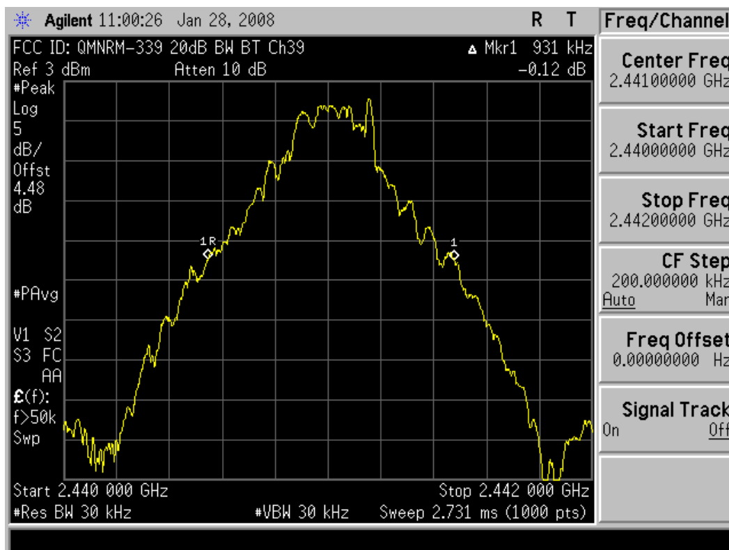
Plot 6-2. 20dB Bandwidth Plot (Bluetooth (GFSK) – Ch. 39)
