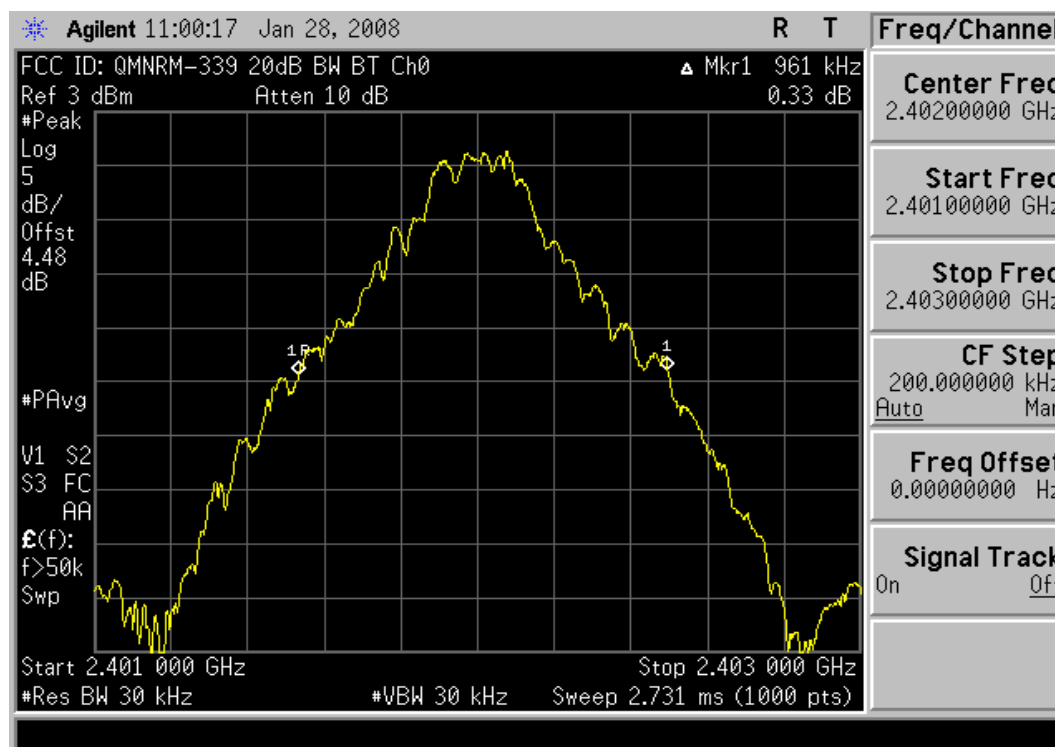
Plot 6-1. 20dB Bandwidth Plot (Bluetooth (GFSK) – Ch. 0)
