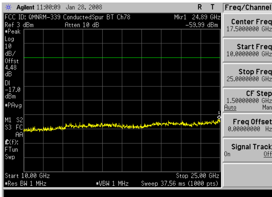
Plot 6-24. Conducted Spurious Plot (Bluetooth (GFSK)– Ch. 78)
