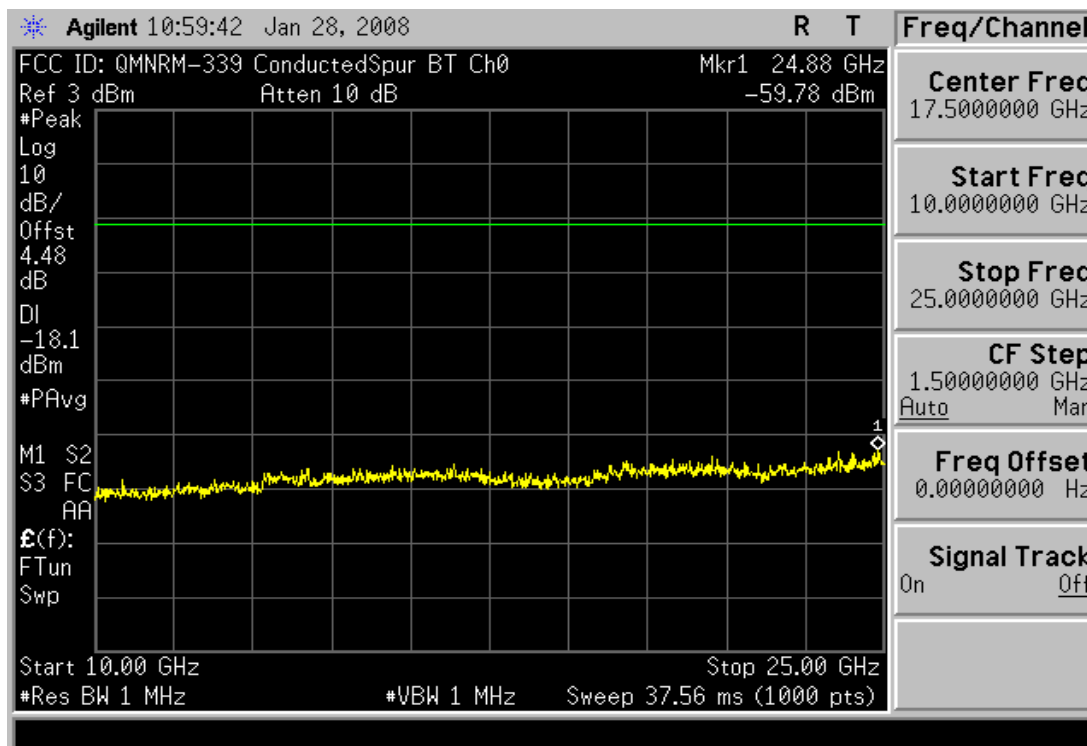
Plot 6-20. Conducted Spurious Plot (Bluetooth (GFSK)– Ch. 0)
