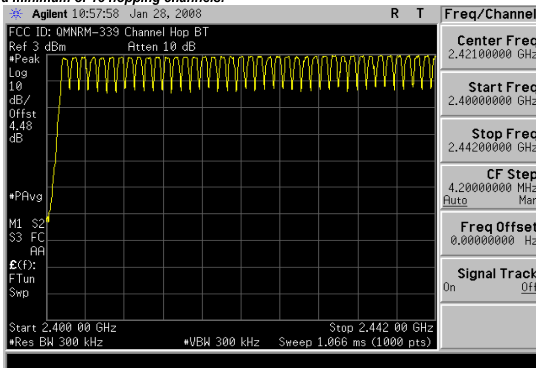
Plot 6-15. Low End Spectrum Channel Hopping Plot (Bluetooth (GFSK))
