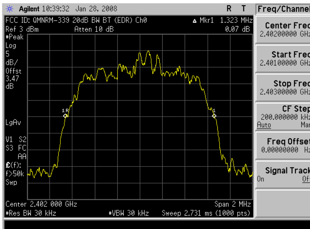
Plot 6-4. 20dB Bandwidth Plot (Bluetooth 2.0 with Enhanced Data Rate – Ch. 0)
