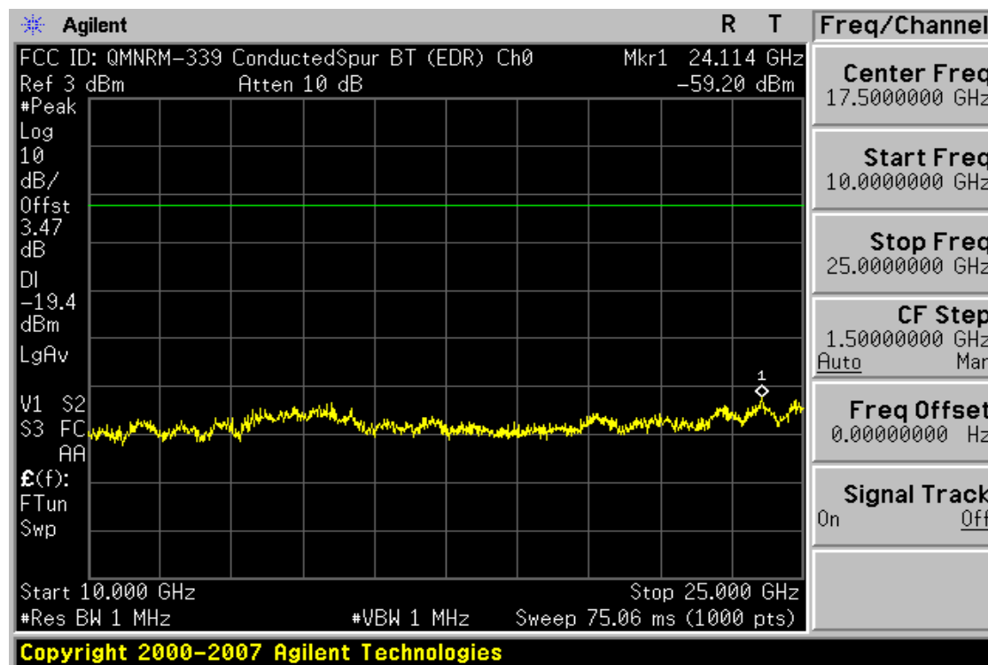
Plot 6-26. Conducted Spurious Plot (Bluetooth 2.0 with Enhanced Data Rate – Ch. 0)
