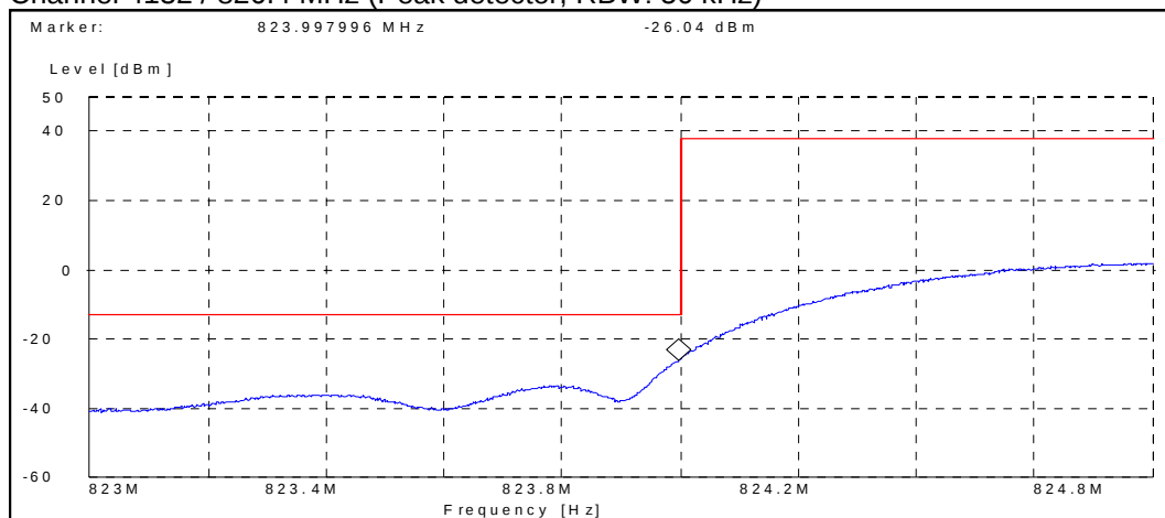
Channel 4132 / 826.4 MHz (Peak detector, RBW: 50 kHz)
