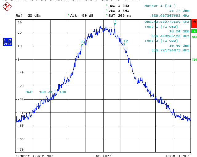
GSM mode, channel 190 / 836.6 MHz
