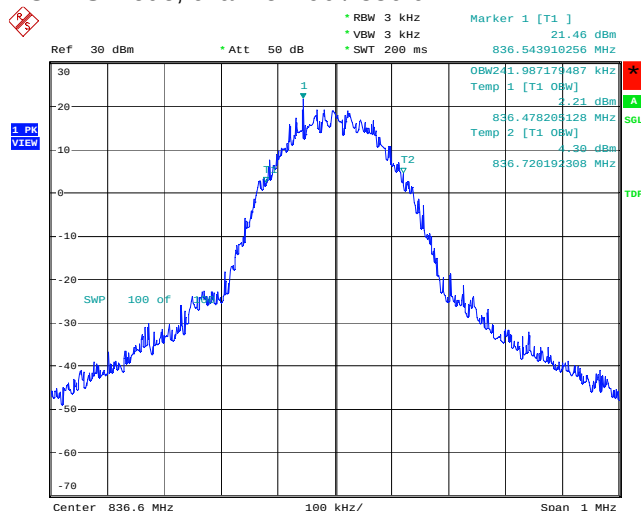
EGPRS mode, channel 190 / 836.6 MHz
