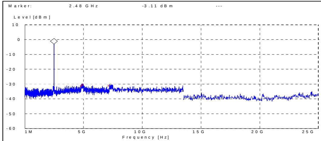
Channel 78 / 2480 MHz
