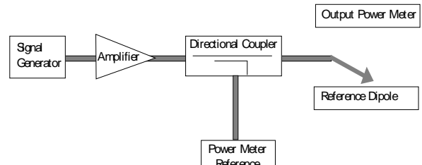
Figure 15 Setup to Dipole
