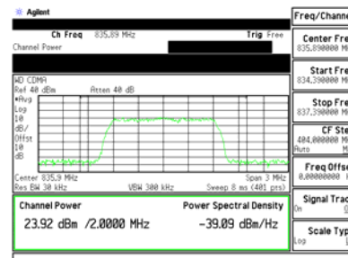
Figure 18 Wireless Device Modulated Signal
