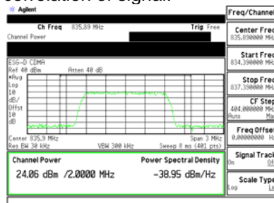
Figure 17 Signal Generator Modulated Signal
