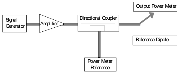
Figure 14 Setup for Desired Output Power to Dipole
