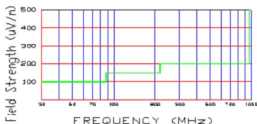
Figure A-1. Limits at 3 meters
