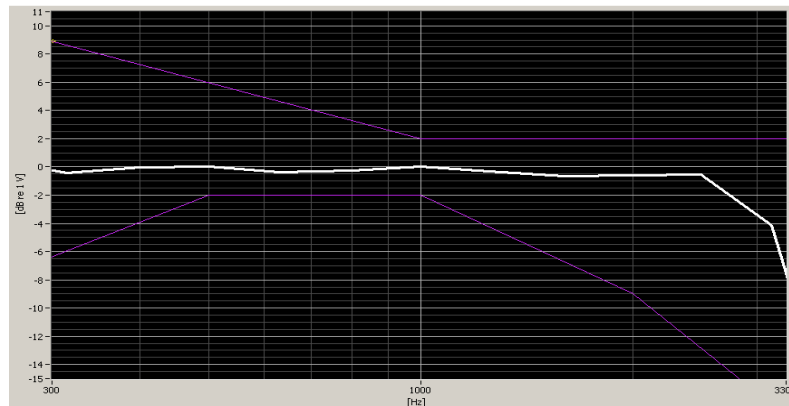
Figure 7-1 Axial Frequency Response
