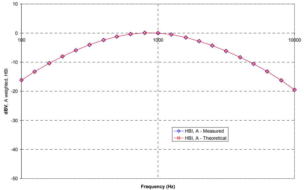
Figure 5-5 ABM2 Frequency Response Validation
