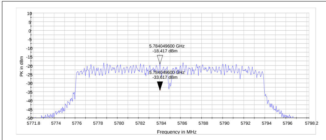
Channel 157 / 5785MHz
