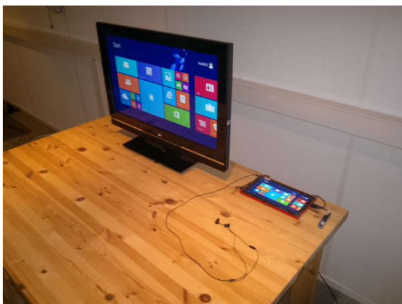
Picture 6. FCC Part 15B AC powerline conducted emissions, HDMI+TV set
