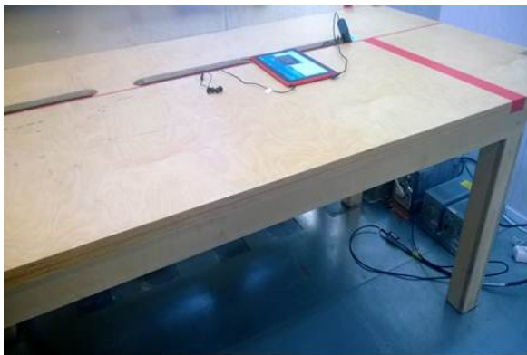
Picture 4. FCC Part 15C AC powerline conducted emissions
