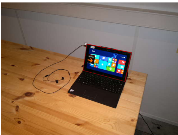
Picture 5. FCC Part 15B AC powerline conducted emissions, Smart cover
