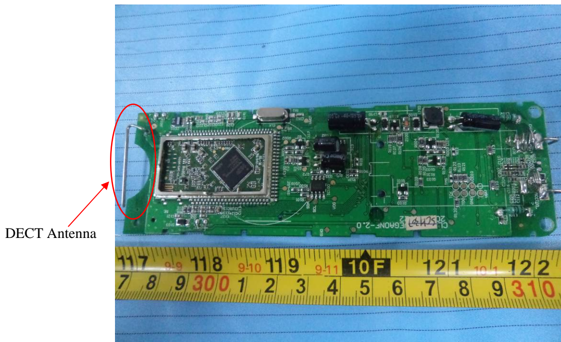
EUT – Handset Main Board Shielding off Bottom View
