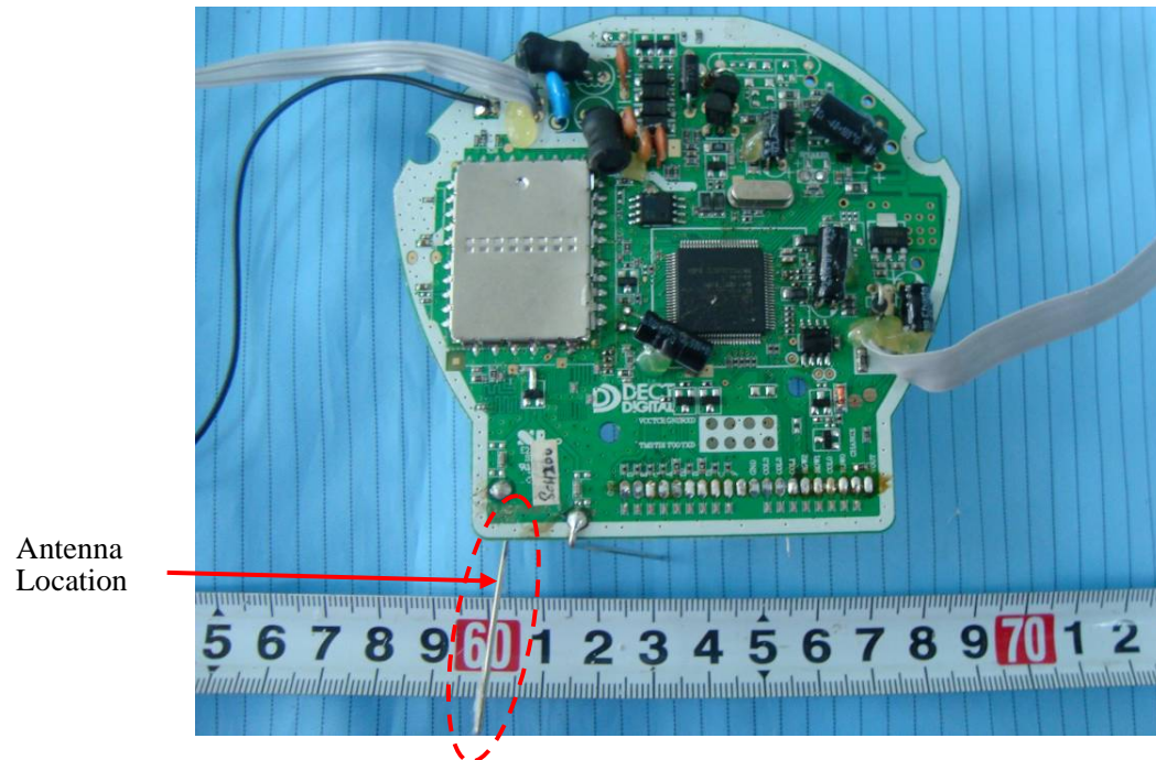
EUT – Main Board without Shielded CoveTop View
