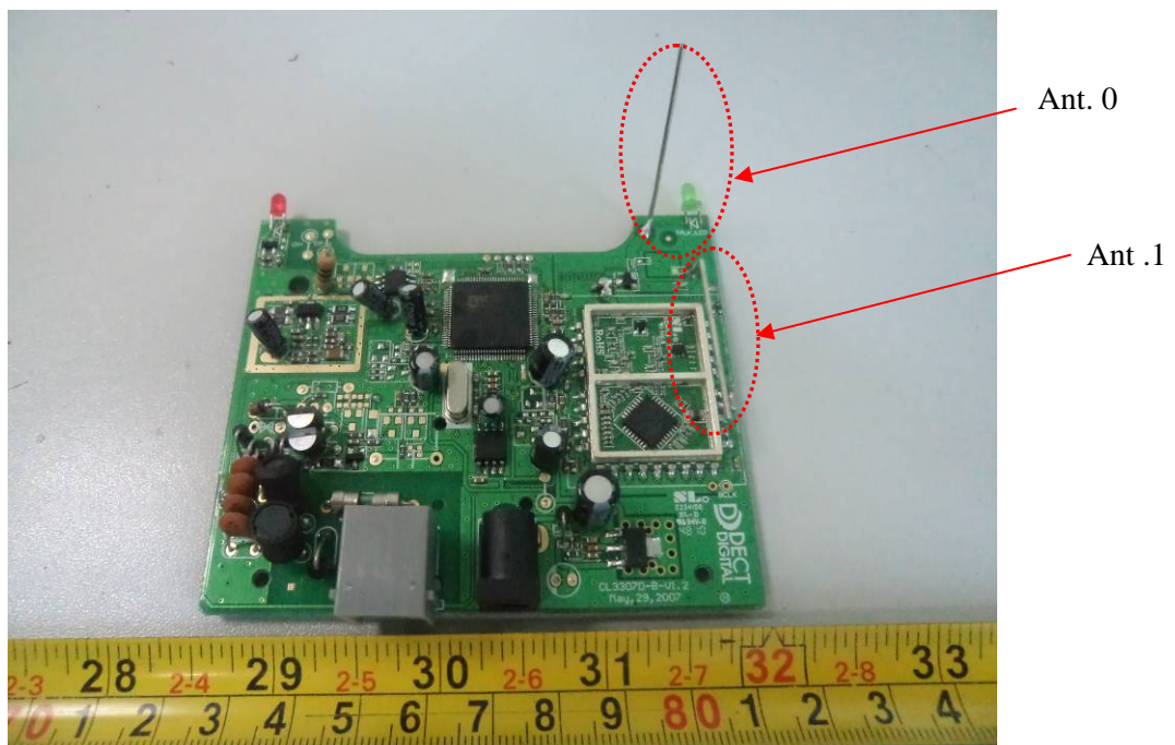
EUT – Main Board Shielding off Top View
