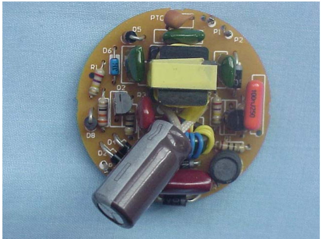
FIGURE 14 SELF-BALLASTED FLUORESCENT LAMP (M/N: DSG/G0-71) PCB BOARD (COMPONENT SIDE)
