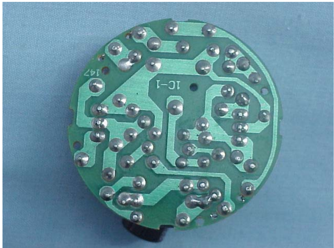
FIGURE 9 SELF-BALLASTED FLUORESCENT LAMP (M/N: DEX/A3-141) PCB BOARD (SOLDERED SIDE)
