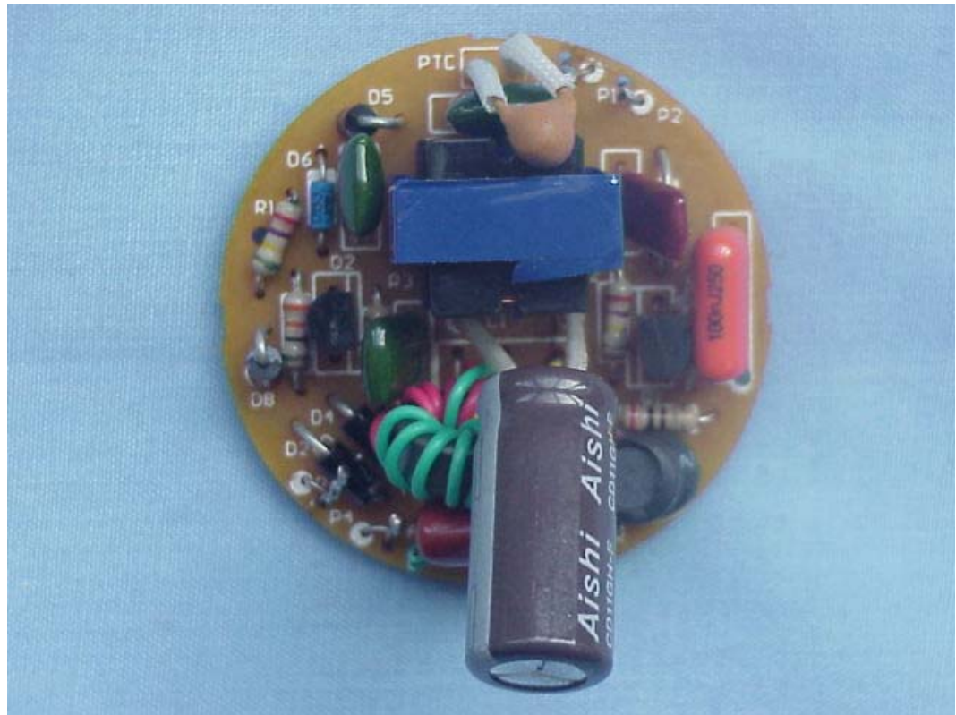
FIGURE 23 SELF-BALLASTED FLUORESCENT LAMP (M/N: DSG/G0-131) PCB BOARD (COMPONENT SIDE)
