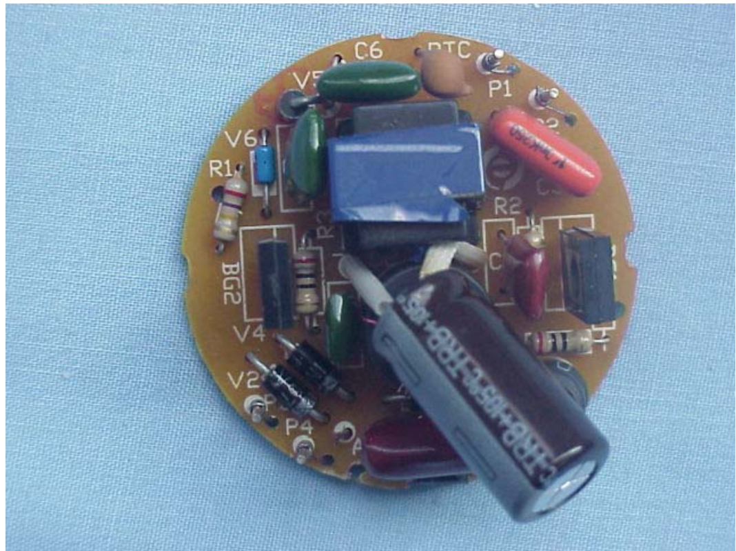
FIGURE 8 SELF-BALLASTED FLUORESCENT LAMP (M/N: DEX/A3-141) PCB BOARD (COMPONENT SIDE)
