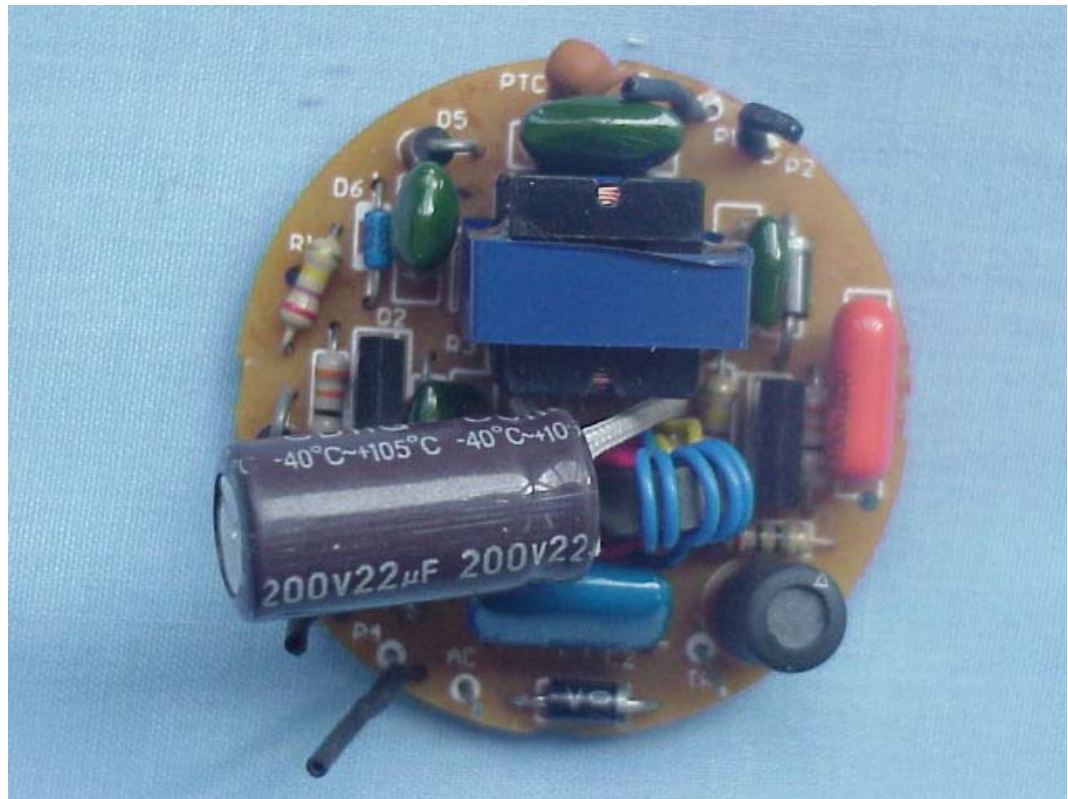
FIGURE 11 SELF-BALLASTED FLUORESCENT LAMP (M/N: DEX/A3-171) PCB BOARD (COMPONENT SIDE)
