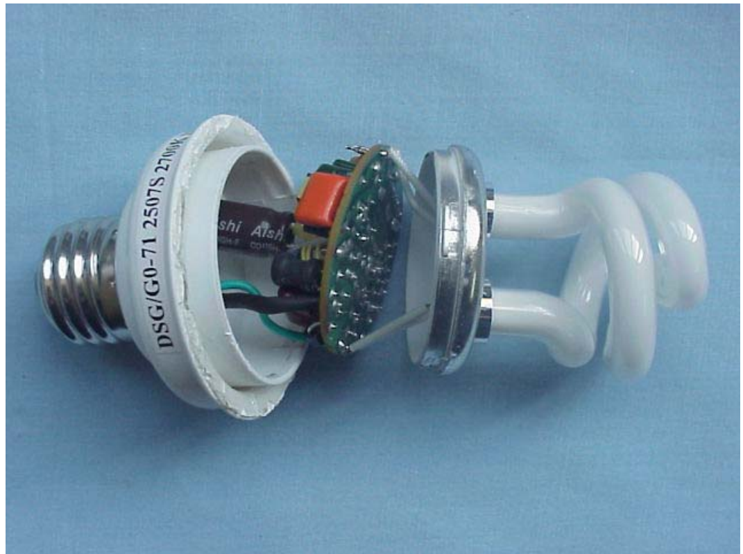
FIGURE 13 SELF-BALLASTED FLUORESCENT LAMP (M/N: DSG/G0-71) COVER REMOVED
