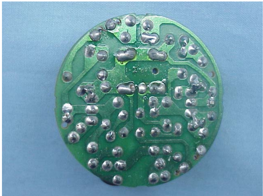
FIGURE 24 SELF-BALLASTED FLUORESCENT LAMP (M/N: DSG/G0-131) PCB BOARD (SOLDERED SIDE)
