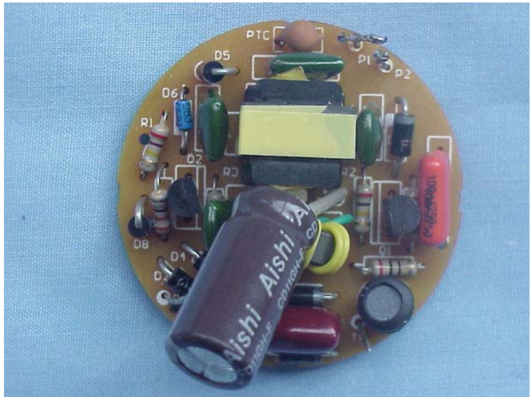
FIGURE 17 SELF-BALLASTED FLUORESCENT LAMP (M/N: DSG/G0-91) PCB BOARD (COMPONENT SIDE)
