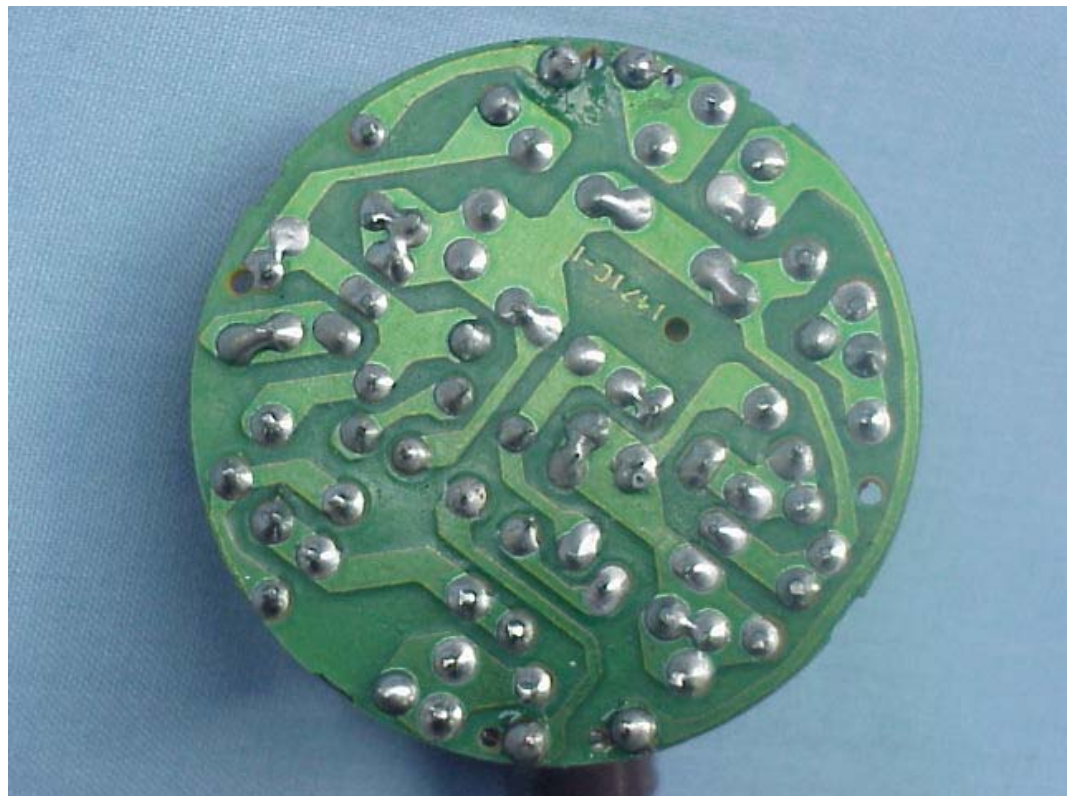
FIGURE 15 SELF-BALLASTED FLUORESCENT LAMP (M/N: DSG/G0-71) PCB BOARD (SOLDERED SIDE)
