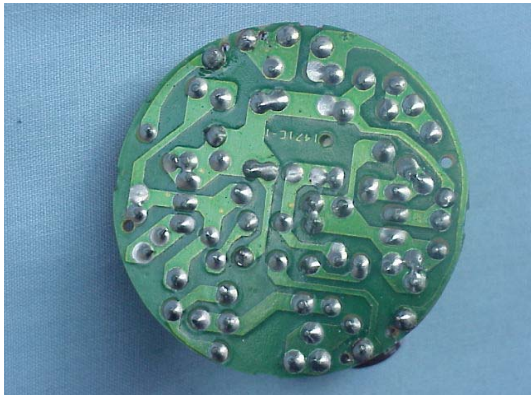
FIGURE 18 SELF-BALLASTED FLUORESCENT LAMP (M/N: DSG/G0-91) PCB BOARD (SOLDERED SIDE)
