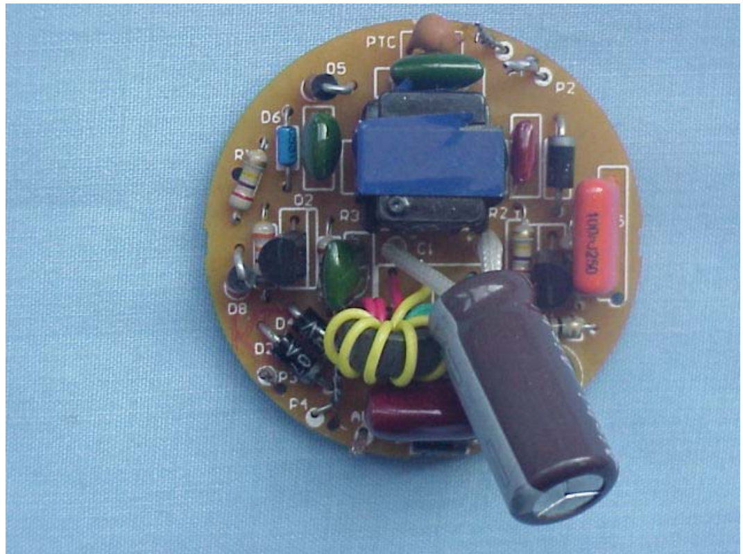
FIGURE 20 SELF-BALLASTED FLUORESCENT LAMP (M/N: DSG/G0-111) PCB BOARD (COMPONENT SIDE)
