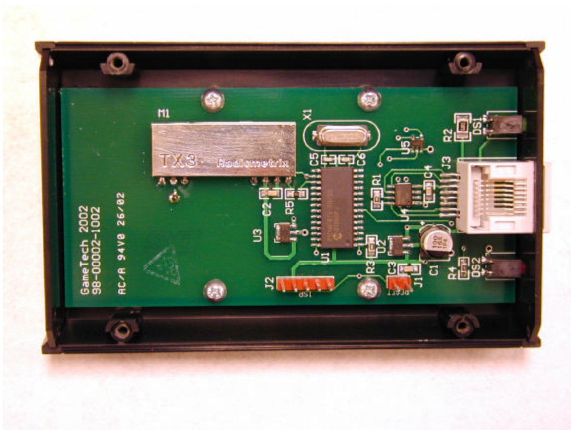
PC IN ENCLOSURE
