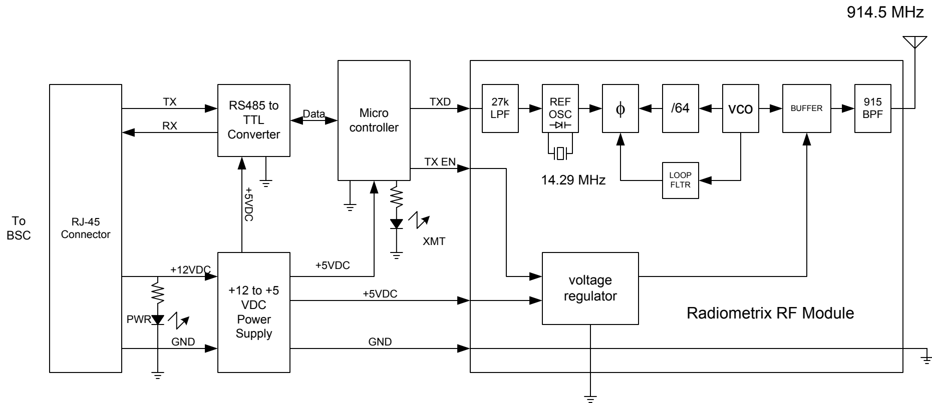
GameTech 900 MHz Single Frequency RF Transmitter Block Diagram
