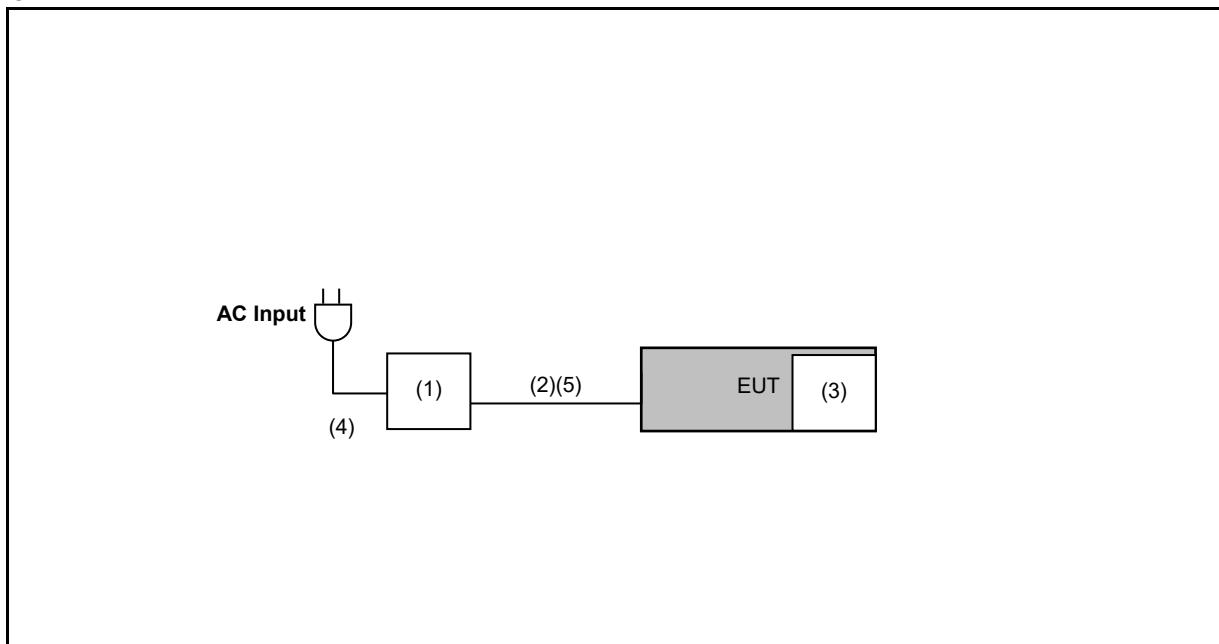
Conduction Emission
