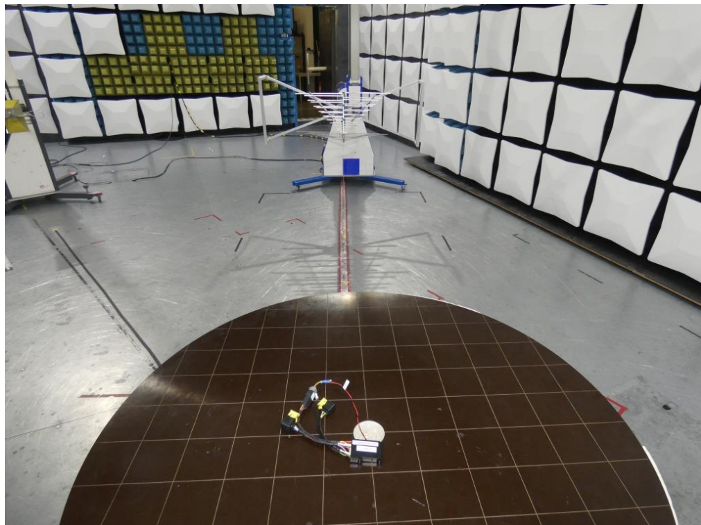
Photo 2: Test setup for radiated measurements below 1 GHz
