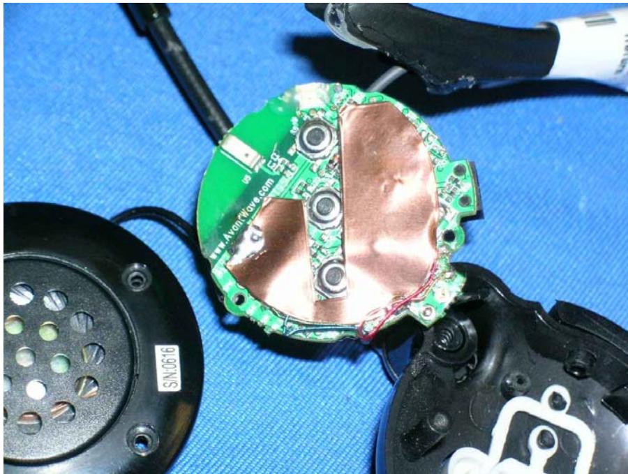
Headset Main PCB solder side (View 1)
