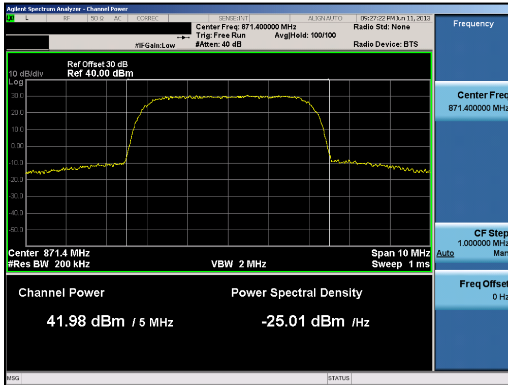
Plot 6-3. Maximum Conducted Power (Low Ch – 871.4MHz – 64QAM)
