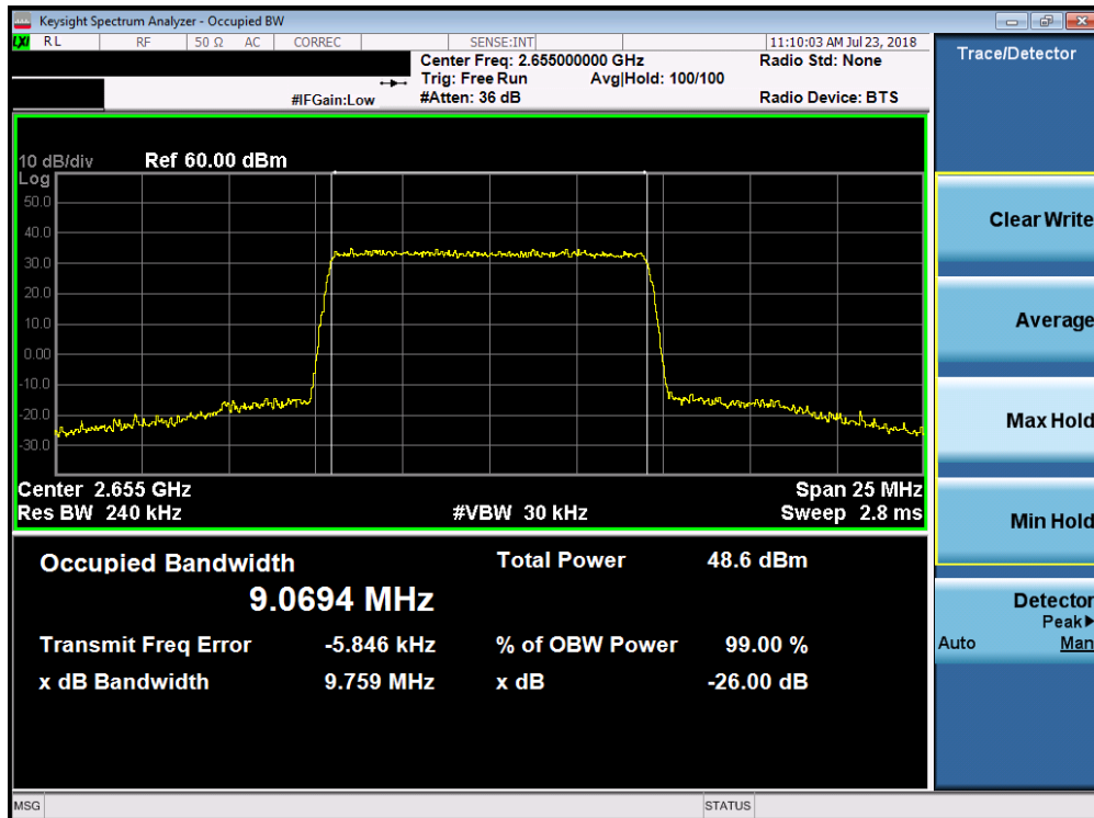
Plot 7-104. Occupied Bandwidth Plot (Band 7 - 10.0MHz 256-QAM)
