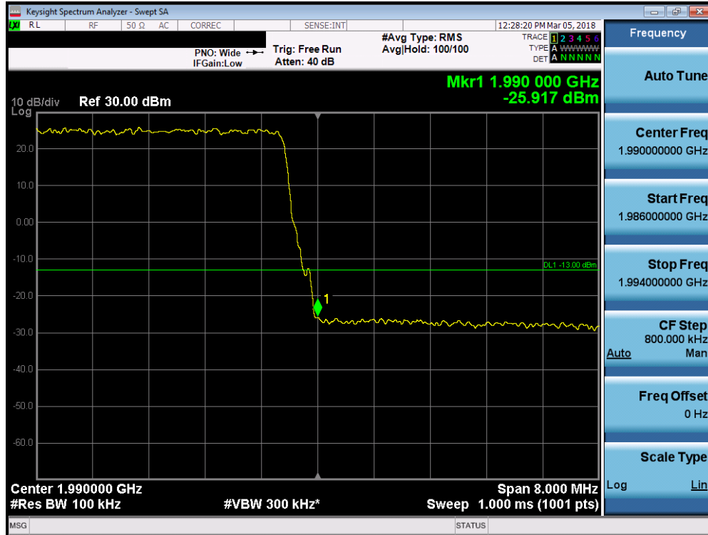
Plot 7-361. Upper Band Edge Plot (Band 2 - 10.0MHz 16-QAM)
