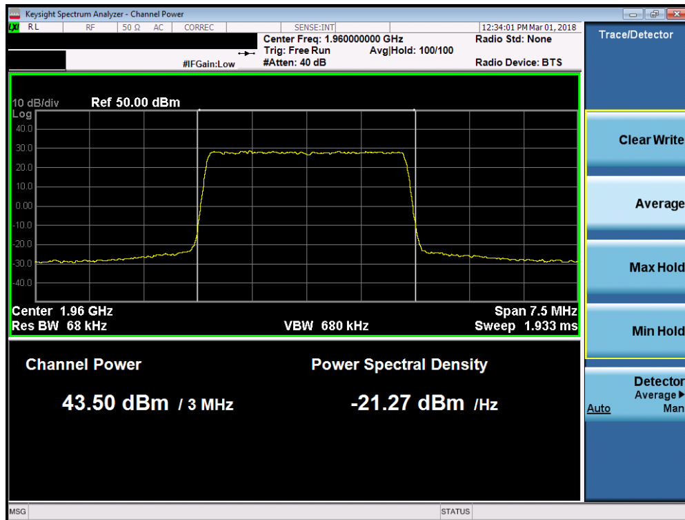
Plot 7-20. Maximum Conducted Power (Band 2 - 3.0MHz 64-QAM – Mid Channel)
