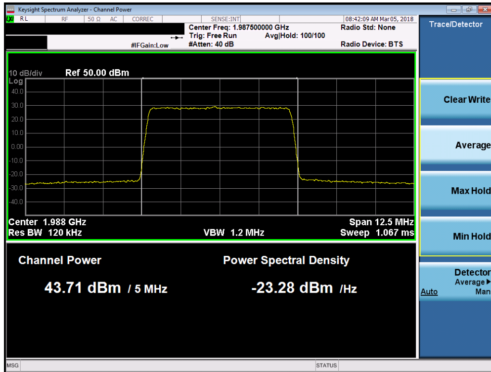
Plot 7-99. Maximum Conducted Power (Band 2 - 5.0MHz QPSK – High Channel)
