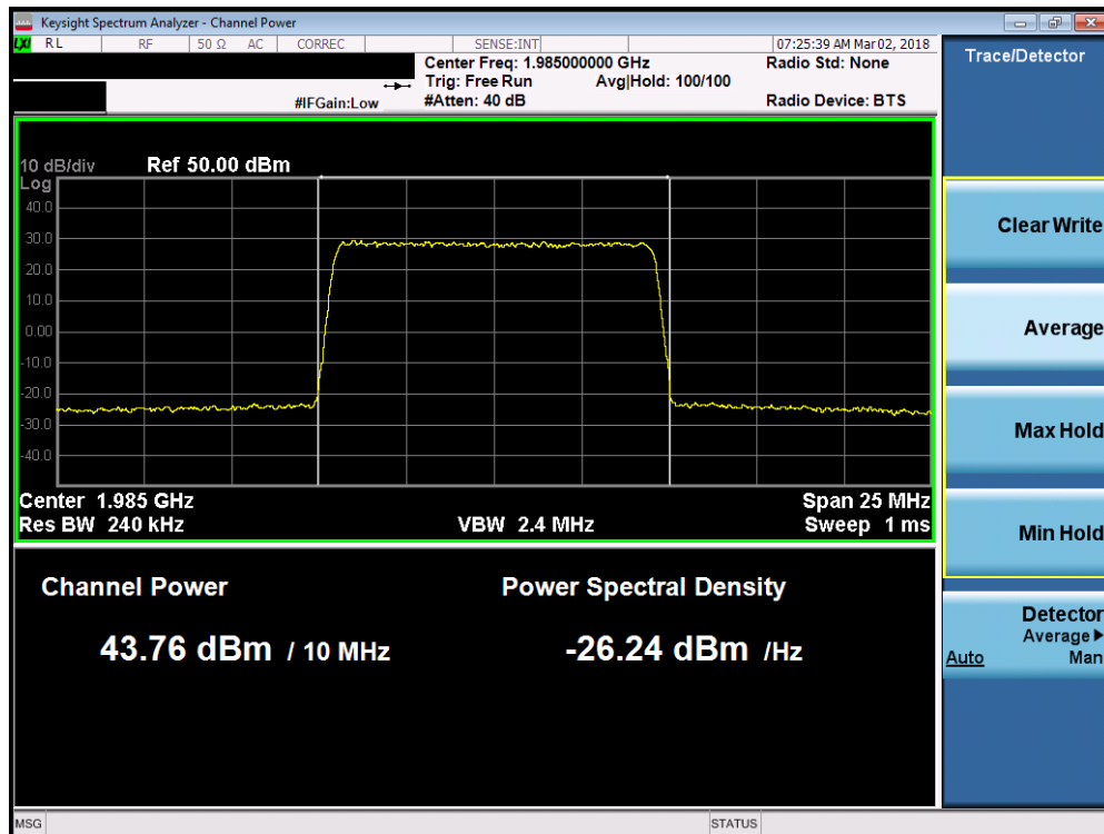
Plot 7-48. Maximum Conducted Power (Band 2 - 10.0MHz 256-QAM – High Channel)
