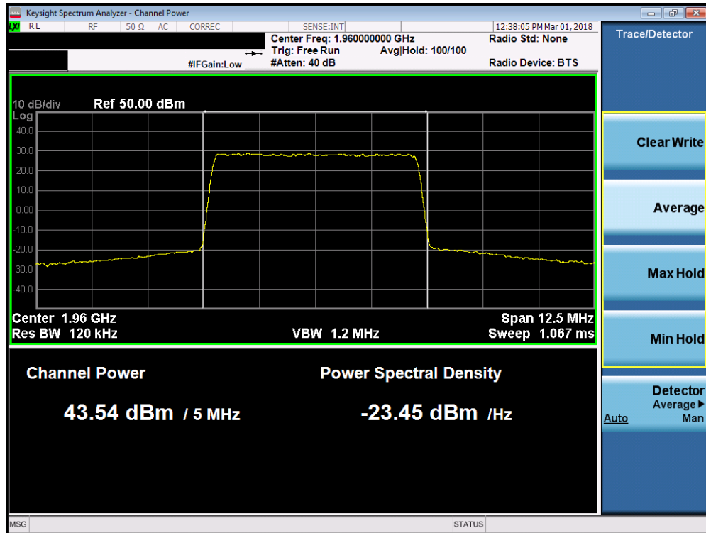
Plot 7-32. Maximum Conducted Power (Band 2 - 5.0MHz 64-QAM – Mid Channel)
