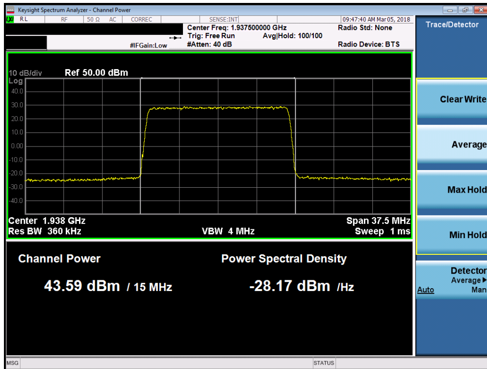
Plot 7-130. Maximum Conducted Power (Band 2 - 15.0MHz 256-QAM – Low Channel)
