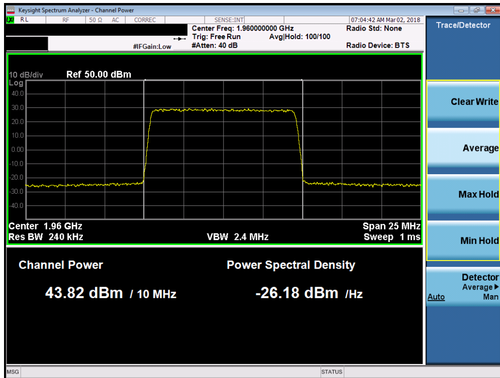
Plot 7-38. Maximum Conducted Power (Band 2 - 10.0MHz QPSK – Mid Channel)
