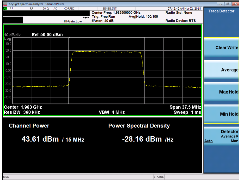
Plot 7-51. Maximum Conducted Power (Band 2 - 15.0MHz QPSK – High Channel)
