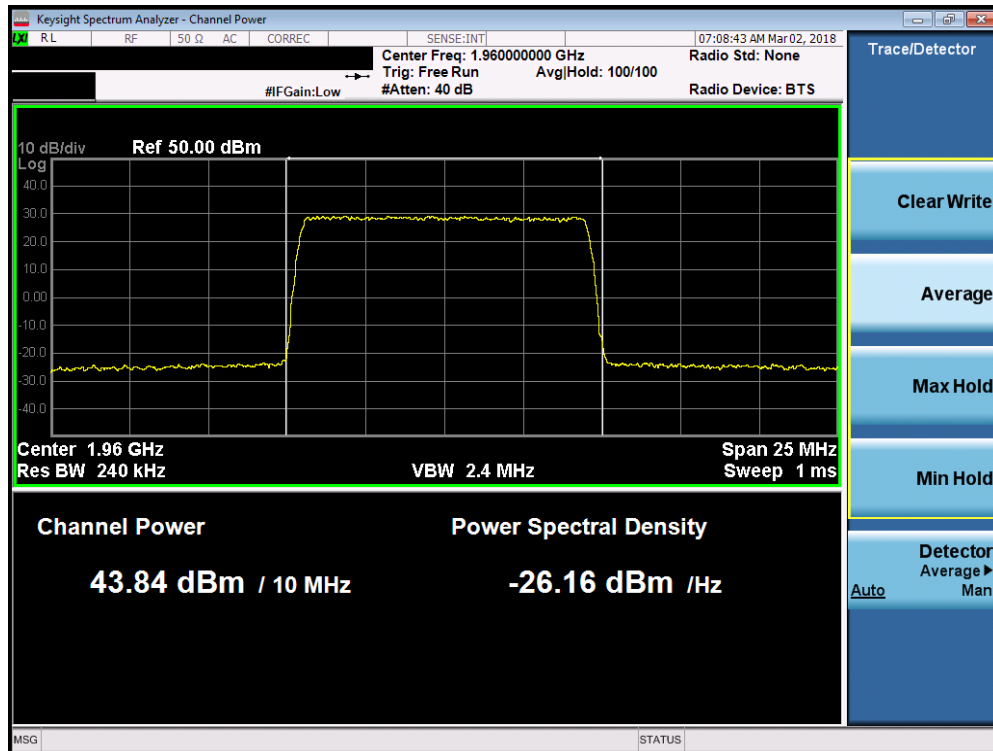
Plot 7-47. Maximum Conducted Power (Band 2 - 10.0MHz 256-QAM – Mid Channel)
