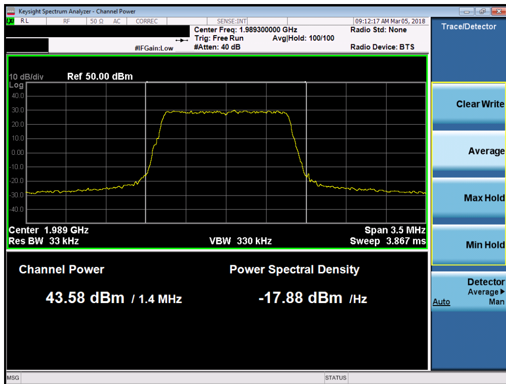
Plot 7-78. Maximum Conducted Power (Band 2 - 1.4MHz 16-QAM – High Channel)
