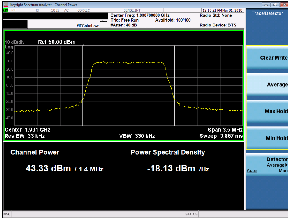
Plot 7-1. Maximum Conducted Power (Band 2 - 1.4MHz QPSK – Low Channel)
