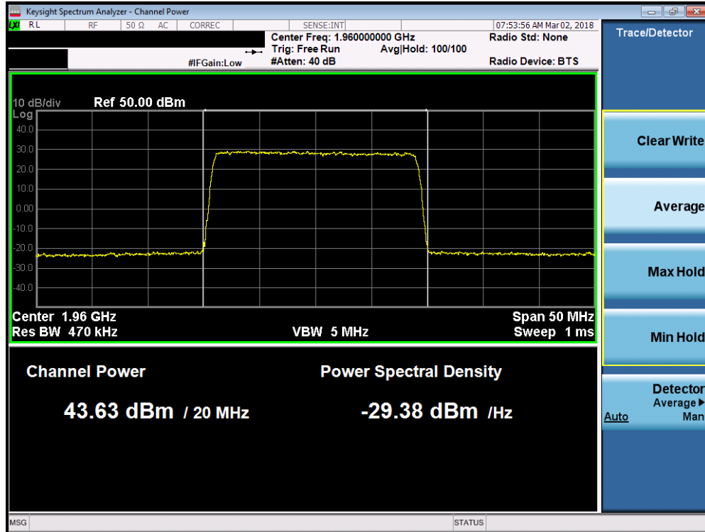
Plot 7-71. Maximum Conducted Power (Band 2 - 20.0MHz 256-QAM – Mid Channel)
