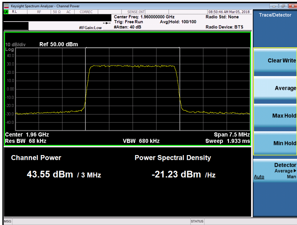
Plot 7-92. Maximum Conducted Power (Band 2 - 3.0MHz 64-QAM – Mid Channel)
