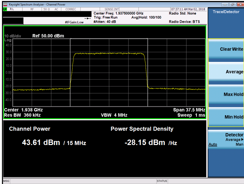
Plot 7-52. Maximum Conducted Power (Band 2 - 15.0MHz 16-QAM – Low Channel)
