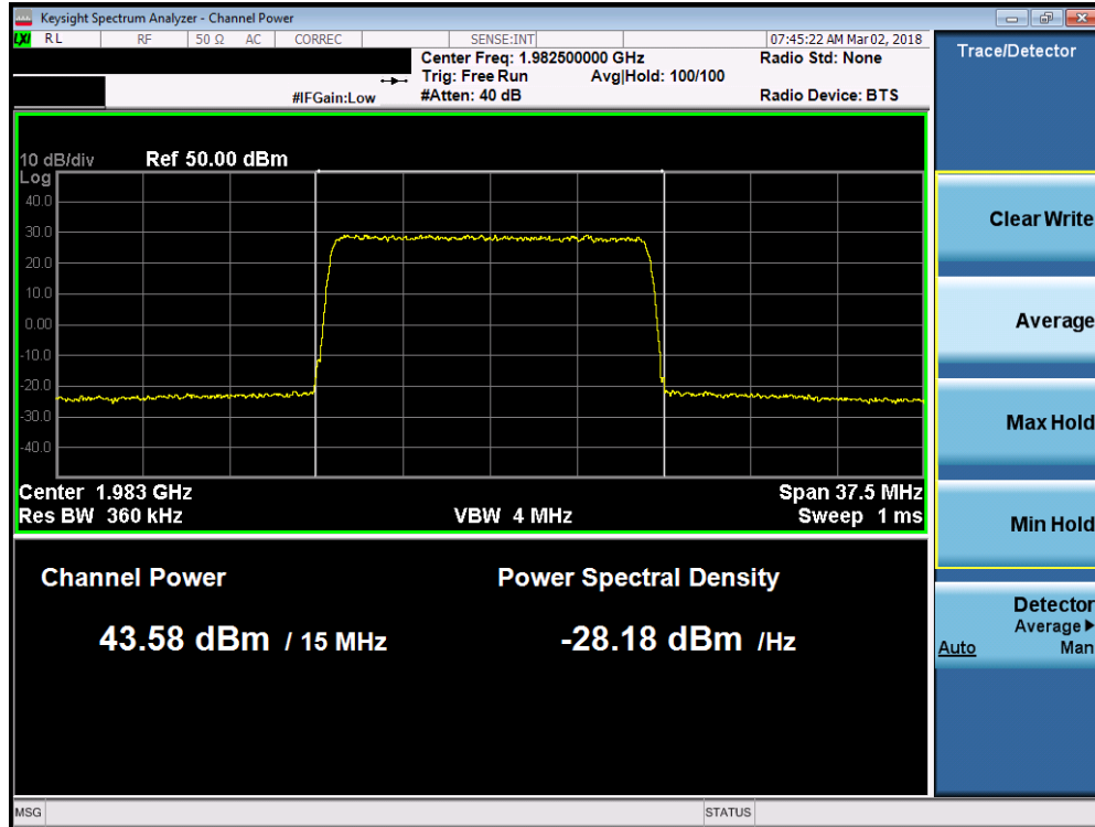
Plot 7-57. Maximum Conducted Power (Band 2 - 15.0MHz 64-QAM – High Channel)
