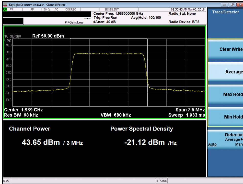
Plot 7-87. Maximum Conducted Power (Band 2 - 3.0MHz QPSK – High Channel)
