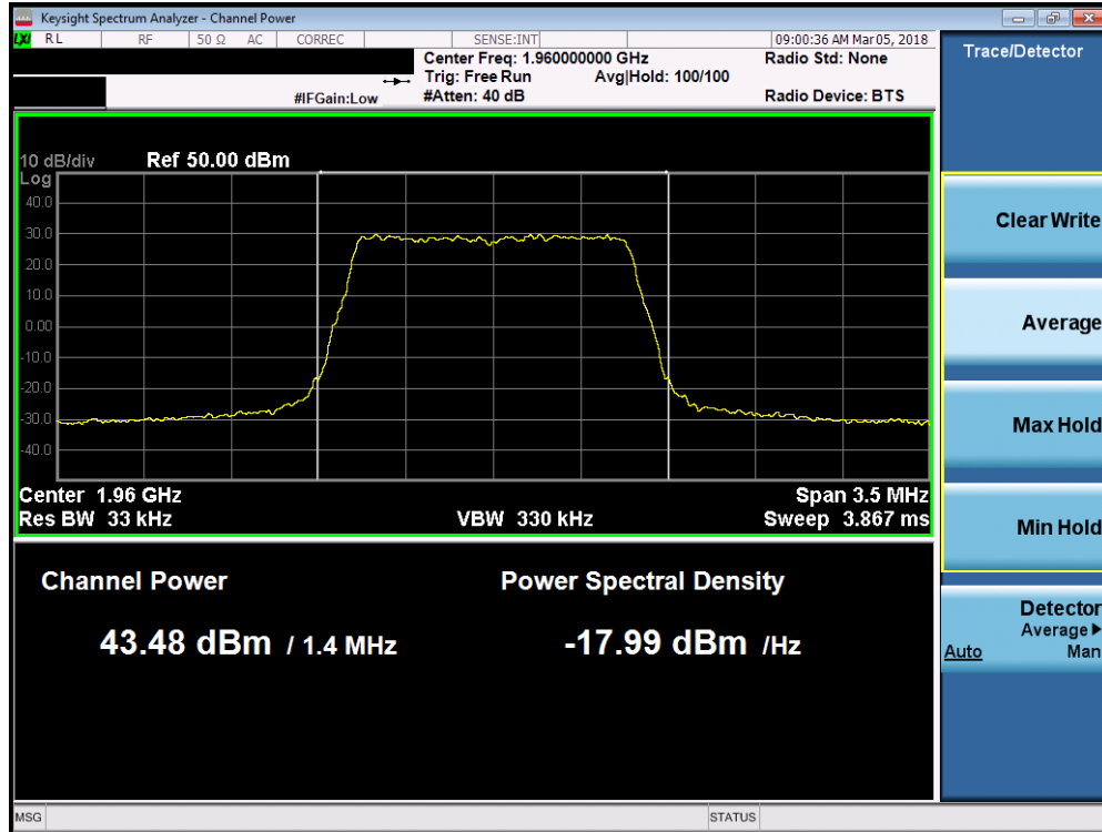
Plot 7-83. Maximum Conducted Power (Band 2 - 1.4MHz 256-QAM – Mid Channel)
