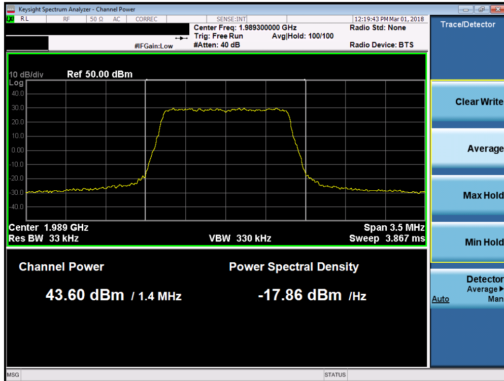
Plot 7-12. Maximum Conducted Power (Band 2 - 1.4MHz 256-QAM – High Channel)
