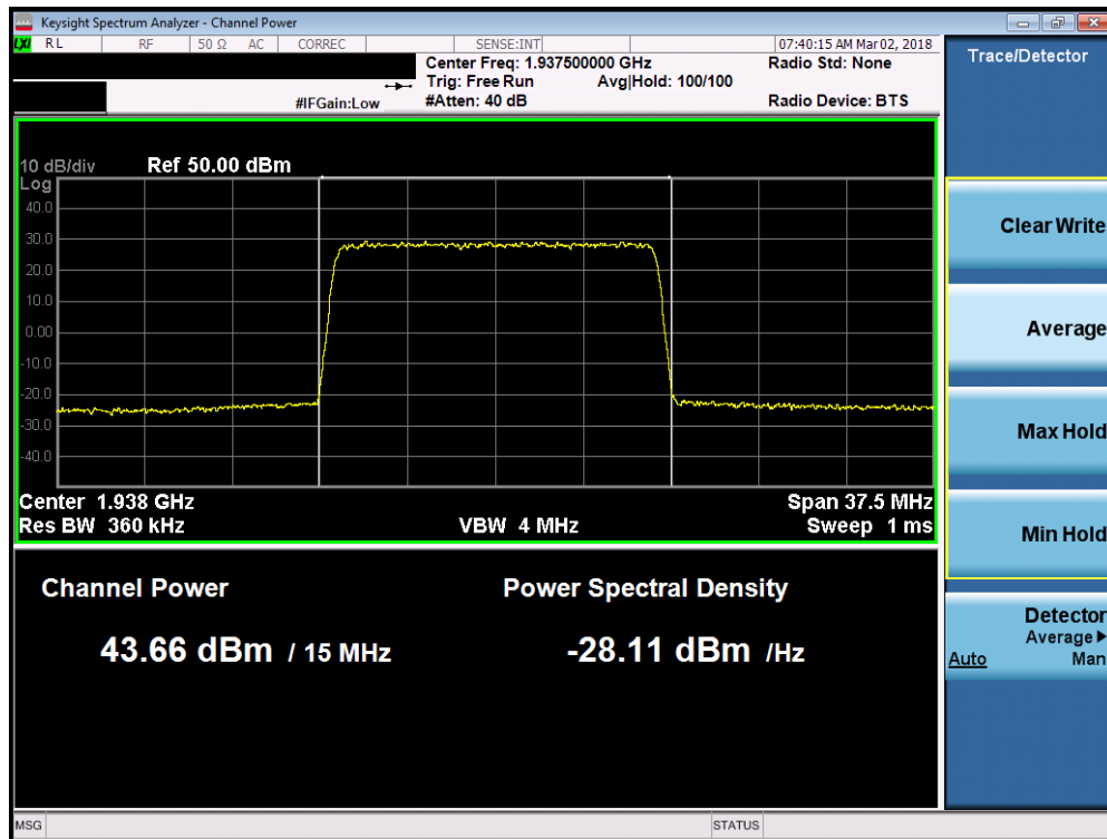
Plot 7-58. Maximum Conducted Power (Band 2 - 15.0MHz 256-QAM – Low Channel)
