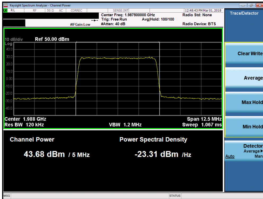
Plot 7-36. Maximum Conducted Power (Band 2 - 5.0MHz 256-QAM – High Channel)
