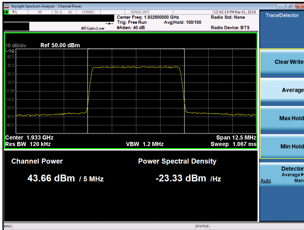
Plot 7-28. Maximum Conducted Power (Band 2 - 5.0MHz 16-QAM – Low Channel)
