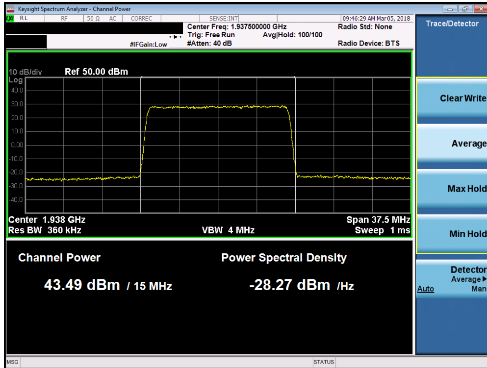
Plot 7-124. Maximum Conducted Power (Band 2 - 15.0MHz 16-QAM – Low Channel)
