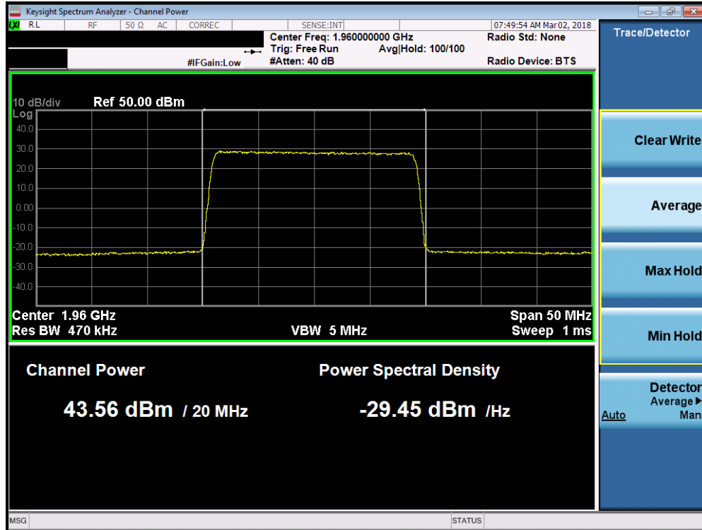
Plot 7-65. Maximum Conducted Power (Band 2 - 20.0MHz 16-QAM – Mid Channel)
