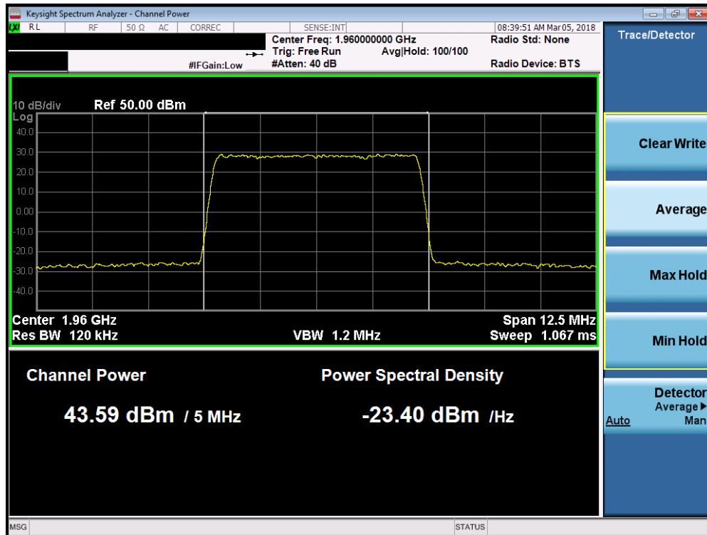
Plot 7-107. Maximum Conducted Power (Band 2 - 5.0MHz 256-QAM – Mid Channel)
