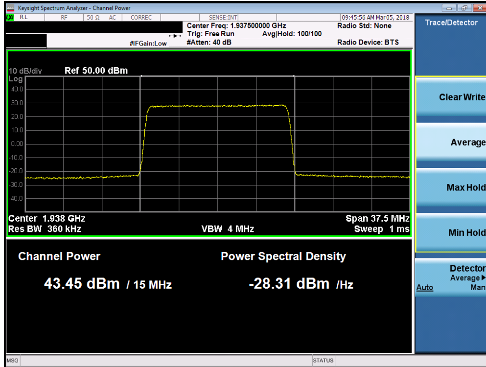
Plot 7-121. Maximum Conducted Power (Band 2 - 15.0MHz QPSK – Low Channel)
