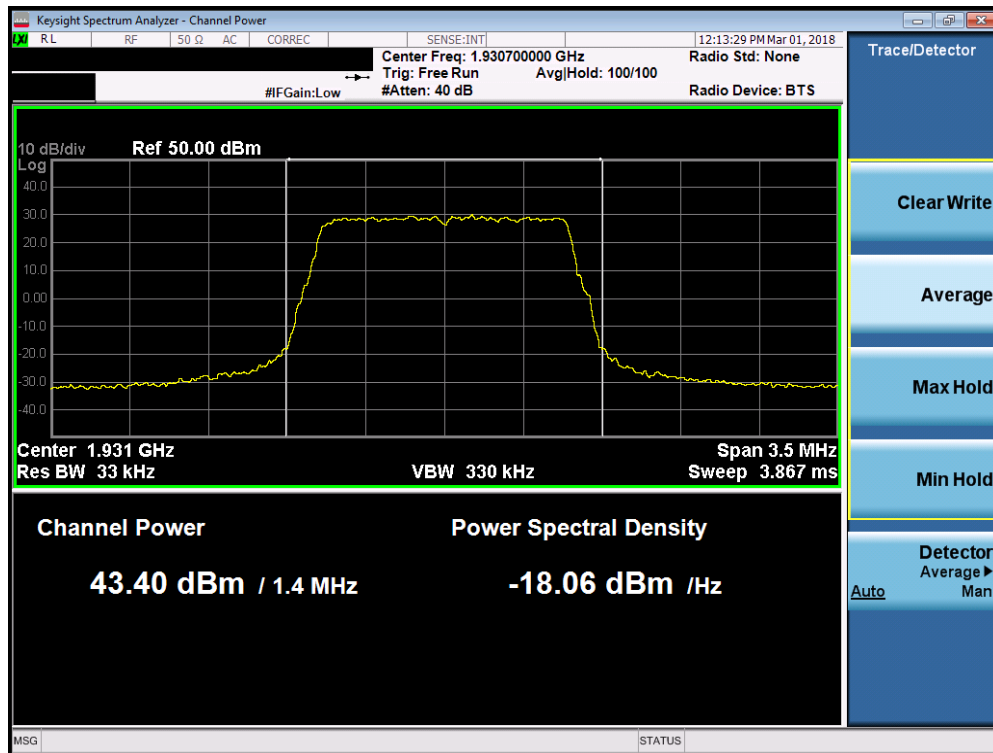
Plot 7-10. Maximum Conducted Power (Band 2 - 1.4MHz 256-QAM – Low Channel)
