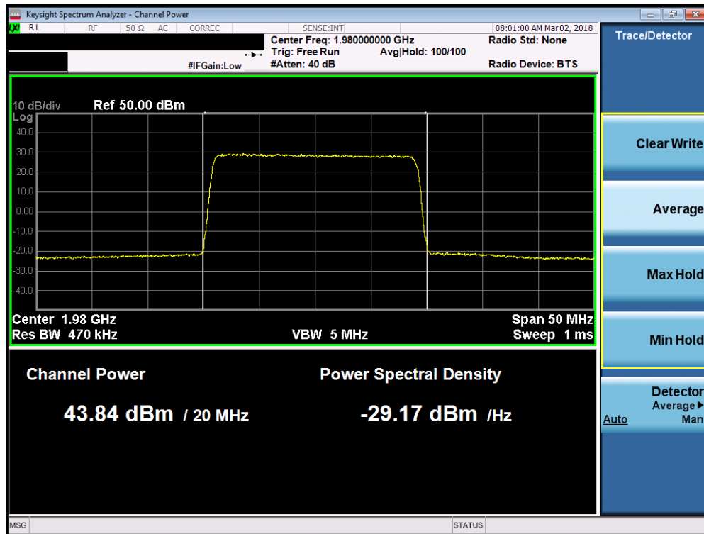
Plot 7-66. Maximum Conducted Power (Band 2 - 20.0MHz 16-QAM – High Channel)
