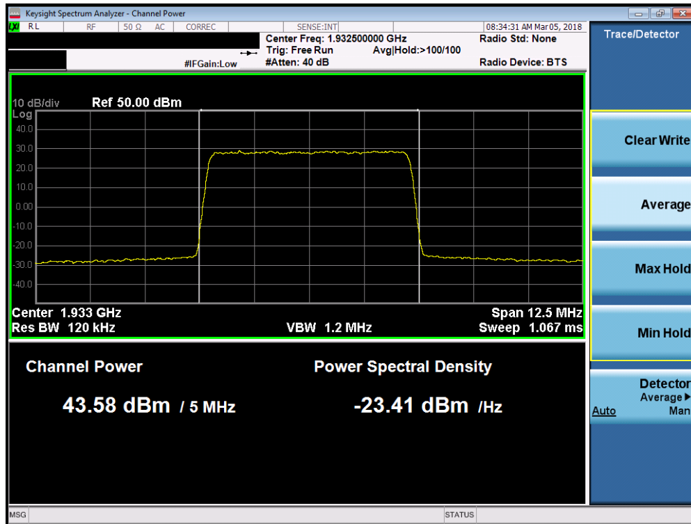
Plot 7-97. Maximum Conducted Power (Band 2 - 5.0MHz QPSK - Low Channel)
