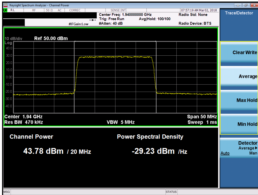
Plot 7-64. Maximum Conducted Power (Band 2 – 20.0MHz 16-QAM – Low Channel)
