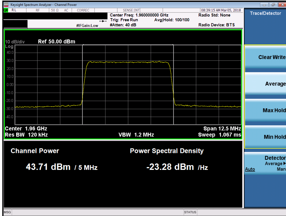
Plot 7-101. Maximum Conducted Power (Band 2 - 5.0MHz 16-QAM – Mid Channel)
