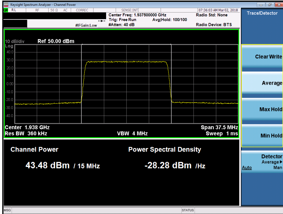
Plot 7-49. Maximum Conducted Power (Band 2 - 15.0MHz QPSK – Low Channel)
