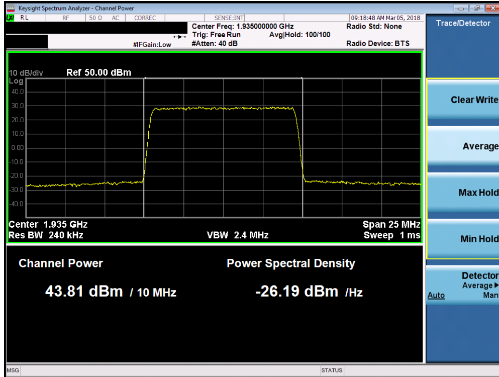
Plot 7-115. Maximum Conducted Power (Band 2 - 10.0MHz 64-QAM - Low Channel)
