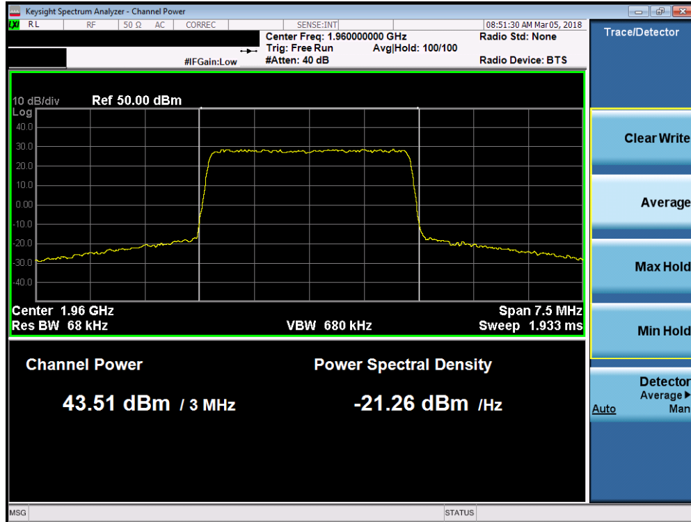
Plot 7-95. Maximum Conducted Power (Band 2 - 3.0MHz 256-QAM – Mid Channel)
