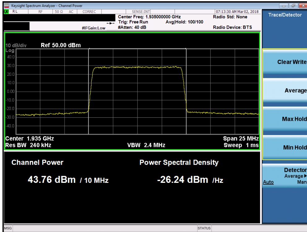
Plot 7-46. Maximum Conducted Power (Band 2 - 10.0MHz 256-QAM – Low Channel)
