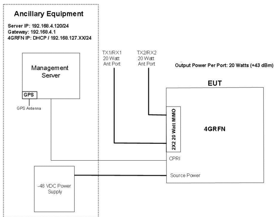
Figure 2-1. Test Setup
