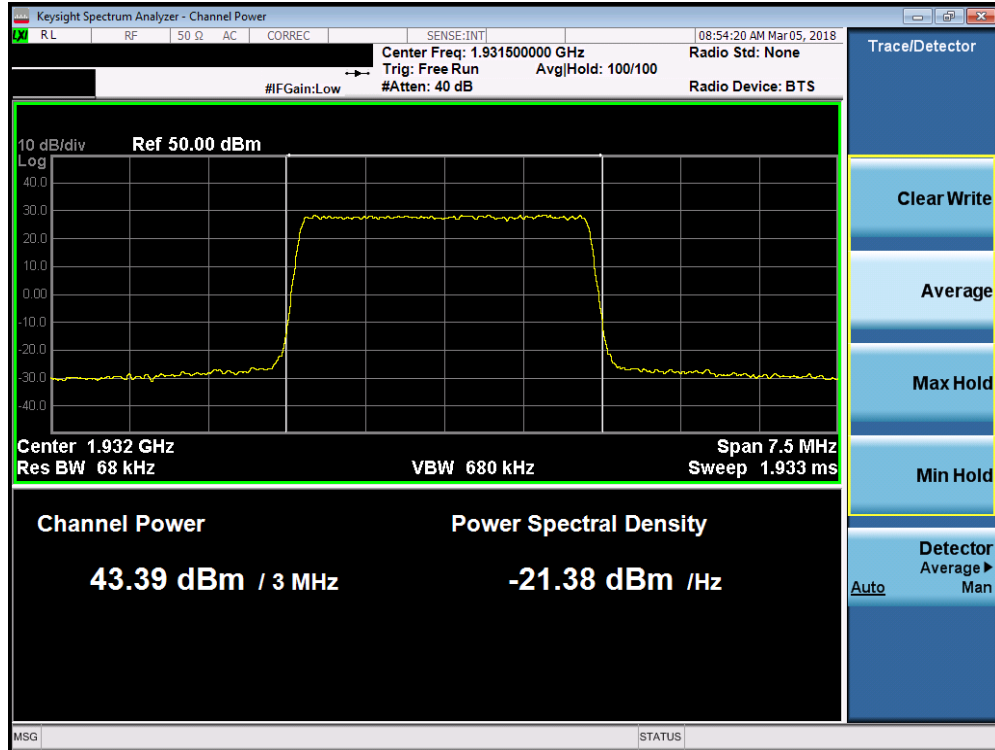
Plot 7-91. Maximum Conducted Power (Band 2 - 3.0MHz 64-QAM - Low Channel)
