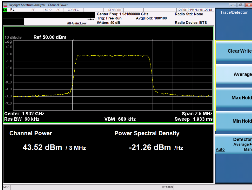
Plot 7-19. Maximum Conducted Power (Band 2 - 3.0MHz 64-QAM – Low Channel)
