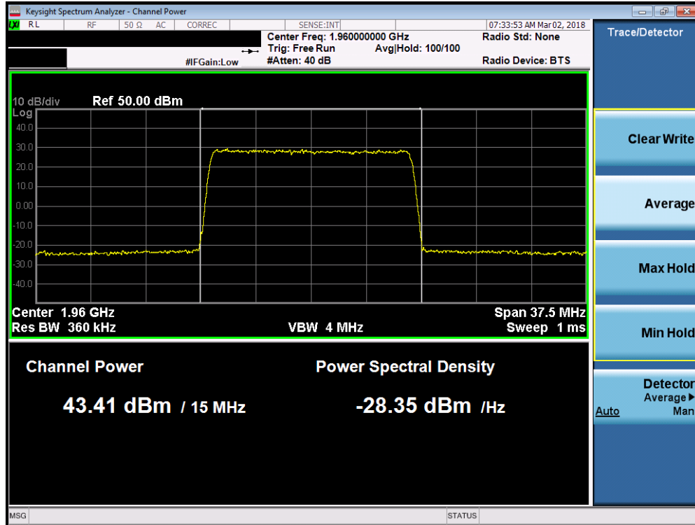
Plot 7-59. Maximum Conducted Power (Band 2 - 15.0MHz 256-QAM – Mid Channel)
