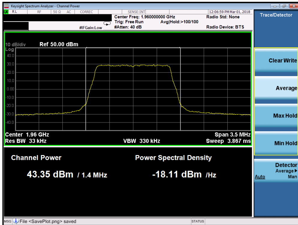
Plot 7-8. Maximum Conducted Power (Band 2 - 1.4MHz 64-QAM – Mid Channel)
