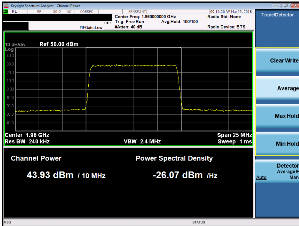
Plot 7-113. Maximum Conducted Power (Band 2 - 10.0MHz 16-QAM – Mid Channel)
