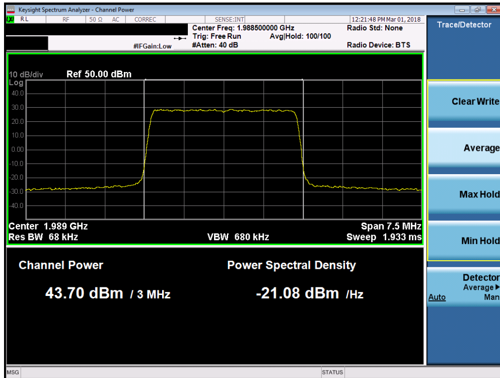
Plot 7-15. Maximum Conducted Power (Band 2 - 3.0MHz QPSK – High Channel)
