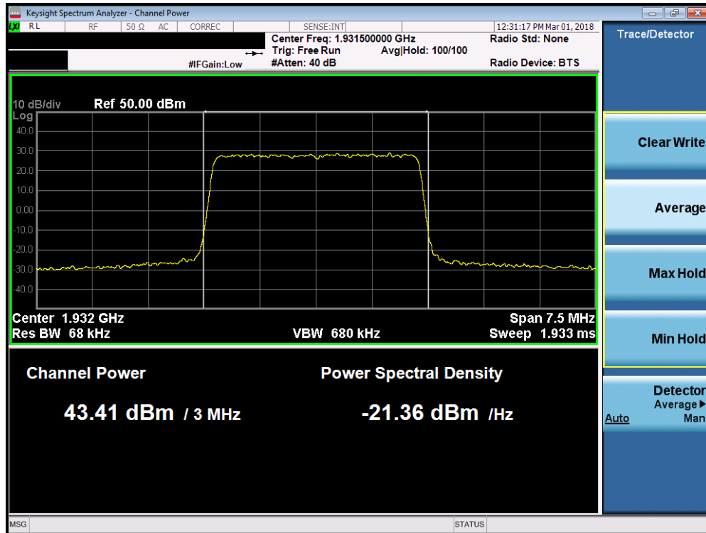
Plot 7-22. Maximum Conducted Power (Band 2 - 3.0MHz 256-QAM – Low Channel)
