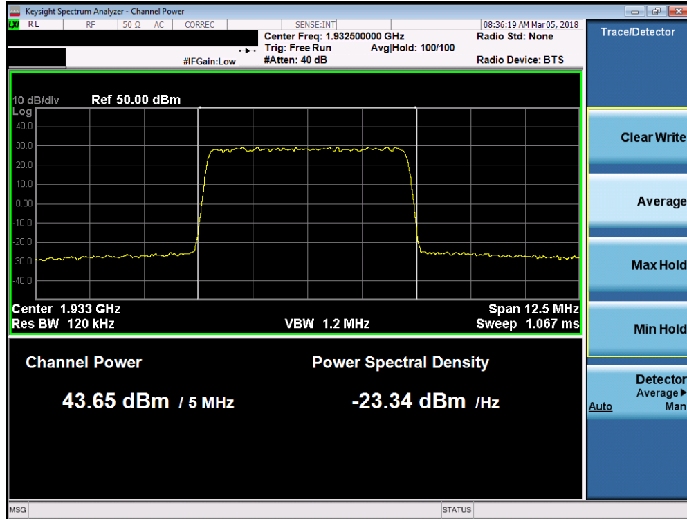
Plot 7-103. Maximum Conducted Power (Band 2 - 5.0MHz 64-QAM - Low Channel)
