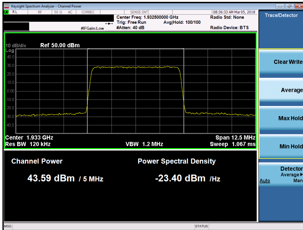
Plot 7-106. Maximum Conducted Power (Band 2 - 5.0MHz 256-QAM - Low Channel)
