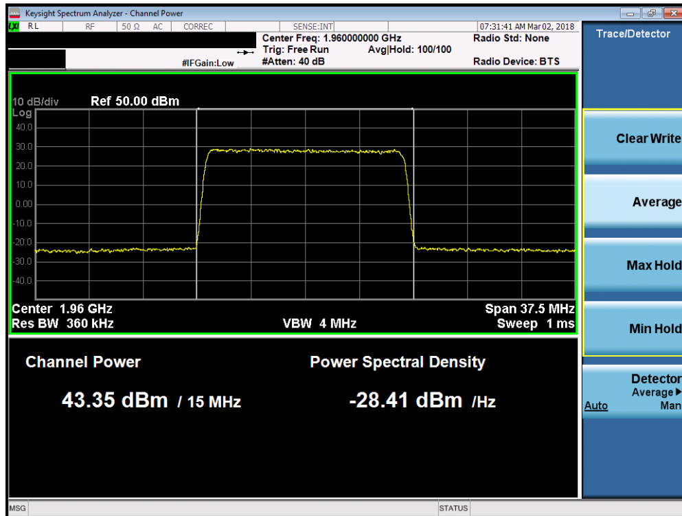
Plot 7-53. Maximum Conducted Power (Band 2 - 15.0MHz 16-QAM – Mid Channel)
