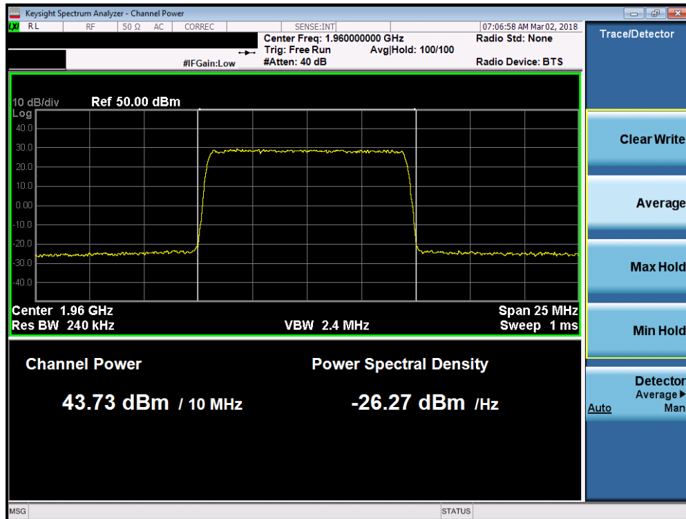
Plot 7-41. Maximum Conducted Power (Band 2 - 10.0MHz 16-QAM – Mid Channel)
