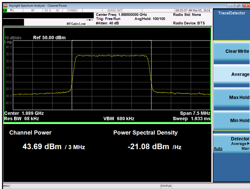
Plot 7-90. Maximum Conducted Power (Band 2 - 3.0MHz 16-QAM – High Channel)
