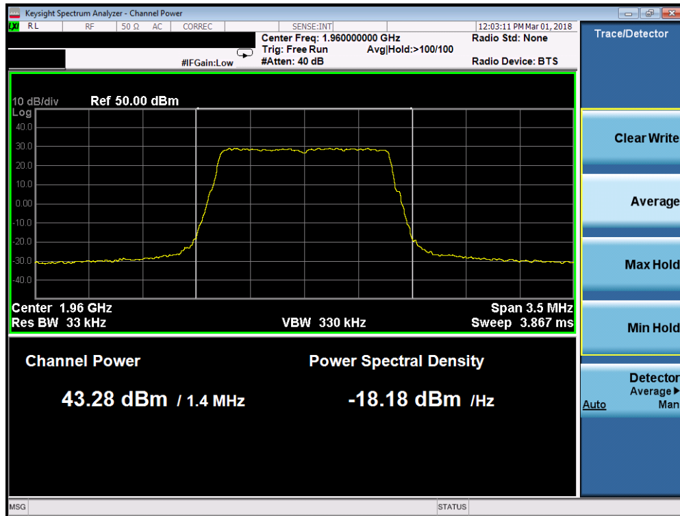
Plot 7-5. Maximum Conducted Power (Band 2 - 1.4MHz 16-QAM – Mid Channel)
