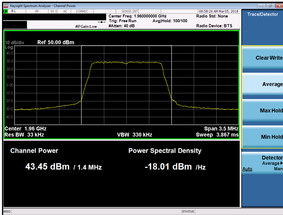
Plot 7-74. Maximum Conducted Power (Band 2 - 1.4MHz QPSK – Mid Channel)
