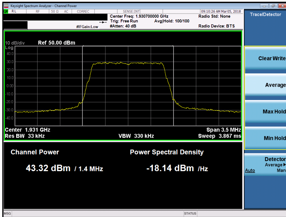
Plot 7-82. Maximum Conducted Power (Band 2 - 1.4MHz 256-QAM - Low Channel)
