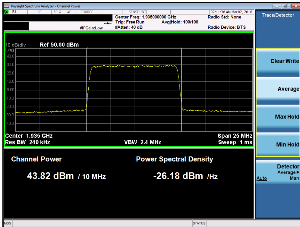
Plot 7-40. Maximum Conducted Power (Band 2 - 10.0MHz 16-QAM – Low Channel)
