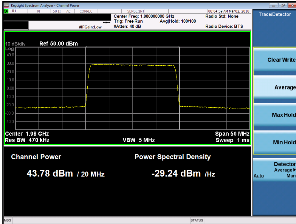
Plot 7-72. Maximum Conducted Power (Band 2 - 20.0MHz 256-QAM – High Channel)
