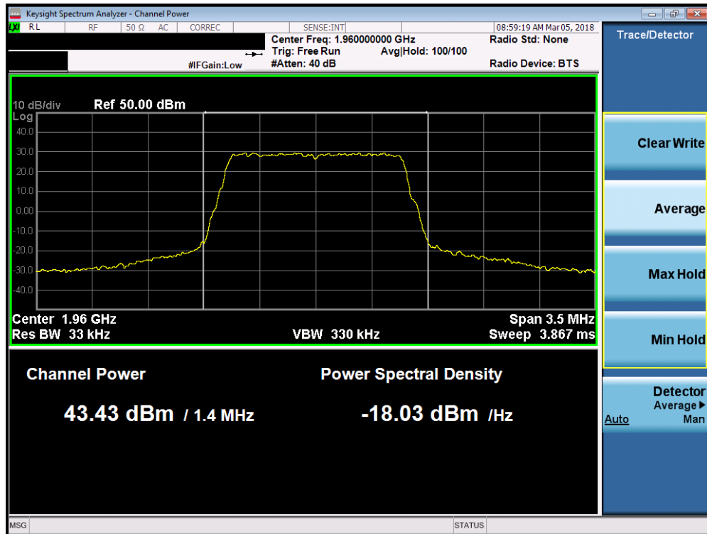
Plot 7-77. Maximum Conducted Power (Band 2 - 1.4MHz 16-QAM – Mid Channel)
