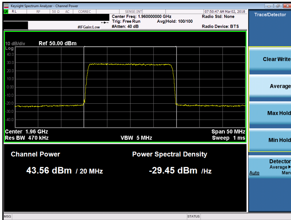
Plot 7-68. Maximum Conducted Power (Band 2 - 20.0MHz 64-QAM – Mid Channel)
