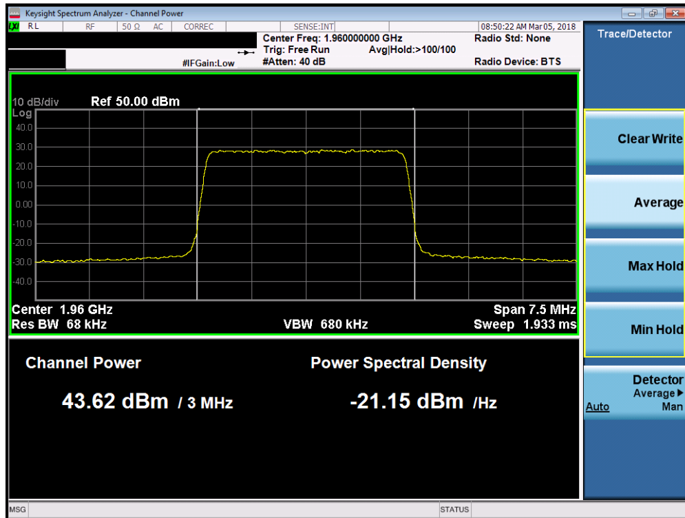
Plot 7-89. Maximum Conducted Power (Band 2 - 3.0MHz 16-QAM – Mid Channel)
