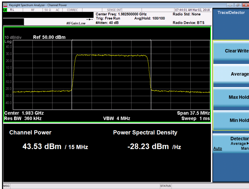
Plot 7-54. Maximum Conducted Power (Band 2 - 15.0MHz 16-QAM – High Channel)
