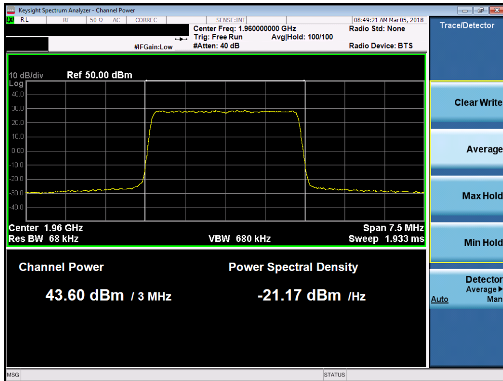
Plot 7-86. Maximum Conducted Power (Band 2 - 3.0MHz QPSK – Mid Channel)
