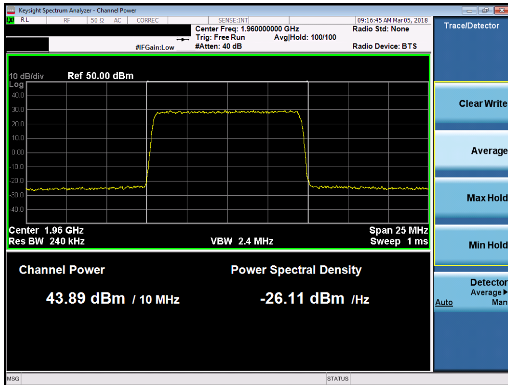
Plot 7-116. Maximum Conducted Power (Band 2 - 10.0MHz 64-QAM - Mid Channel)
