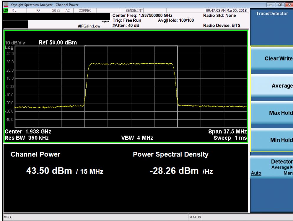
Plot 7-127. Maximum Conducted Power (Band 2 - 15.0MHz 64-QAM – Low Channel)
