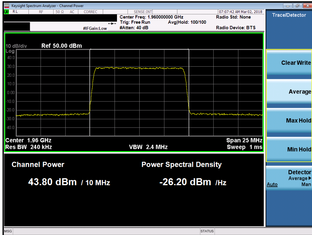
Plot 7-44. Maximum Conducted Power (Band 2 - 10.0MHz 64-QAM – Mid Channel)
