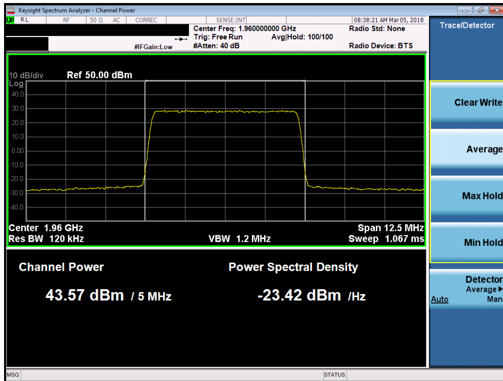
Plot 7-98. Maximum Conducted Power (Band 2 - 5.0MHz QPSK – Mid Channel)
