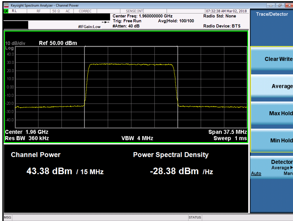
Plot 7-56. Maximum Conducted Power (Band 2 - 15.0MHz 64-QAM – Mid Channel)
