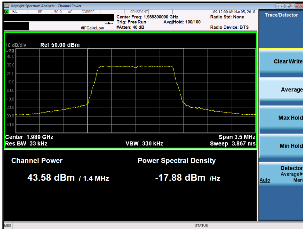
Plot 7-75. Maximum Conducted Power (Band 2 - 1.4MHz QPSK – High Channel)
