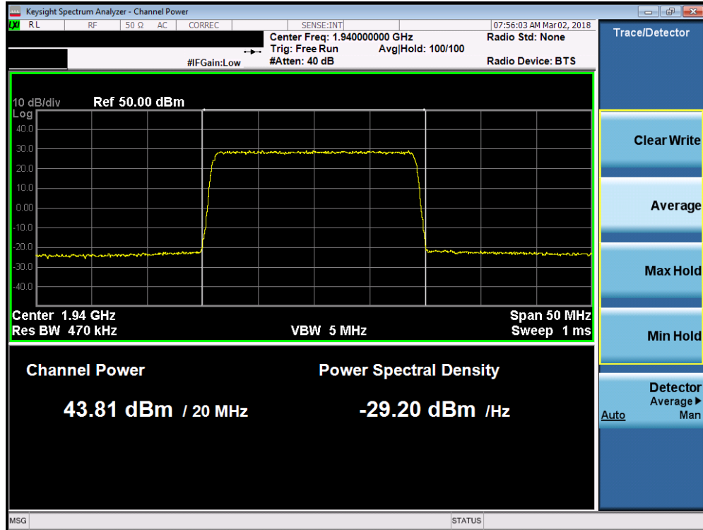
Plot 7-61. Maximum Conducted Power (Band 2 - 20.0MHz QPSK – Low Channel)
