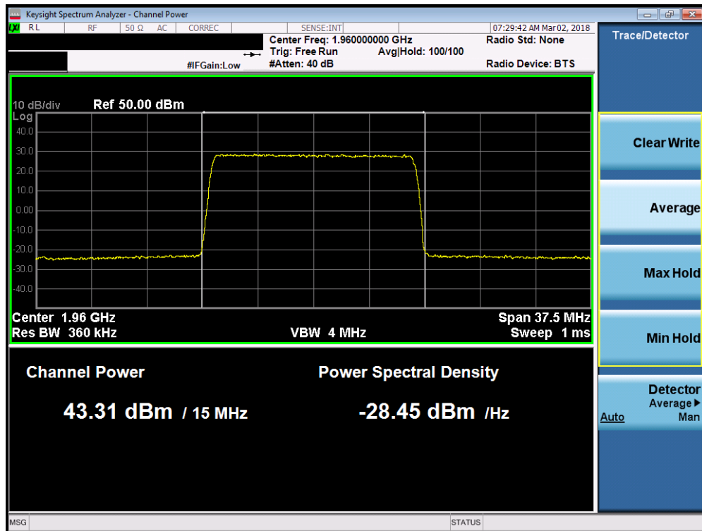
Plot 7-50. Maximum Conducted Power (Band 2 - 15.0MHz QPSK – Mid Channel)
