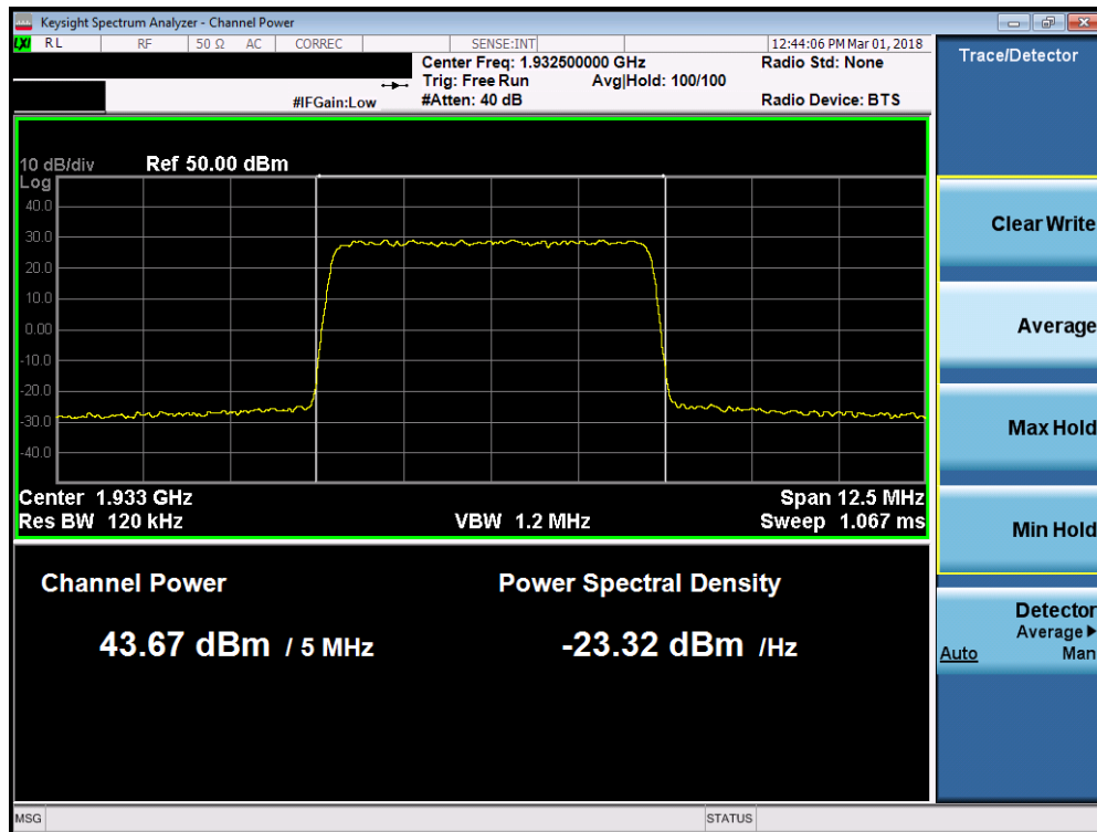
Plot 7-34. Maximum Conducted Power (Band 2 - 5.0MHz 256-QAM – Low Channel)
