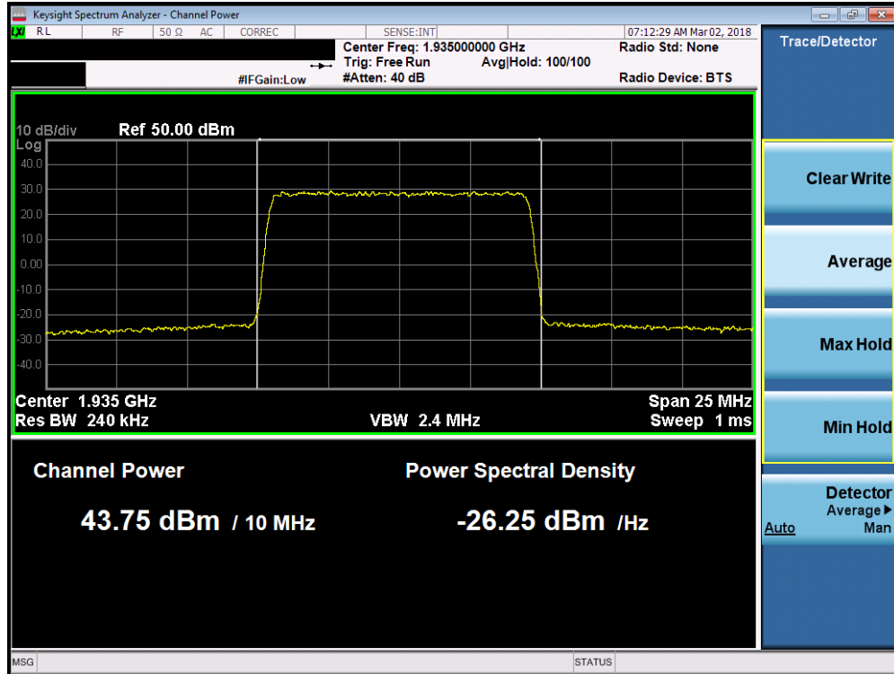
Plot 7-43. Maximum Conducted Power (Band 2 - 10.0MHz 64-QAM – Low Channel)
