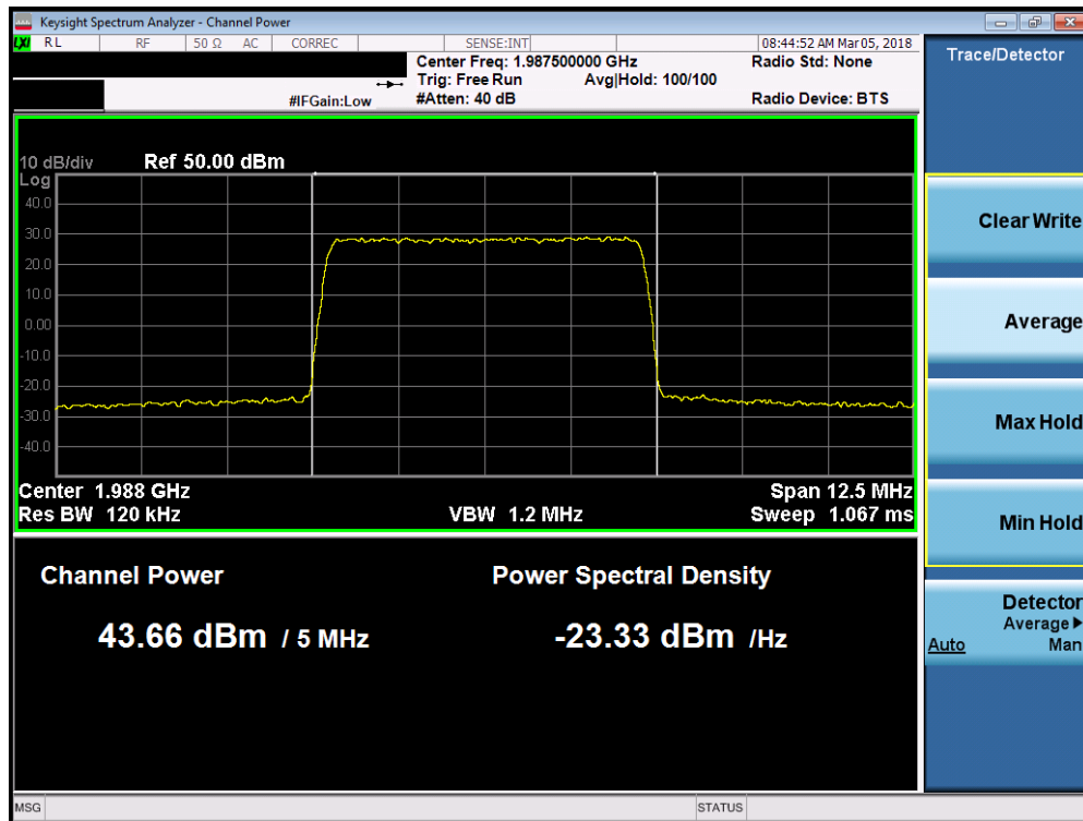
Plot 7-108. Maximum Conducted Power (Band 2 - 5.0MHz 256-QAM – High Channel)
