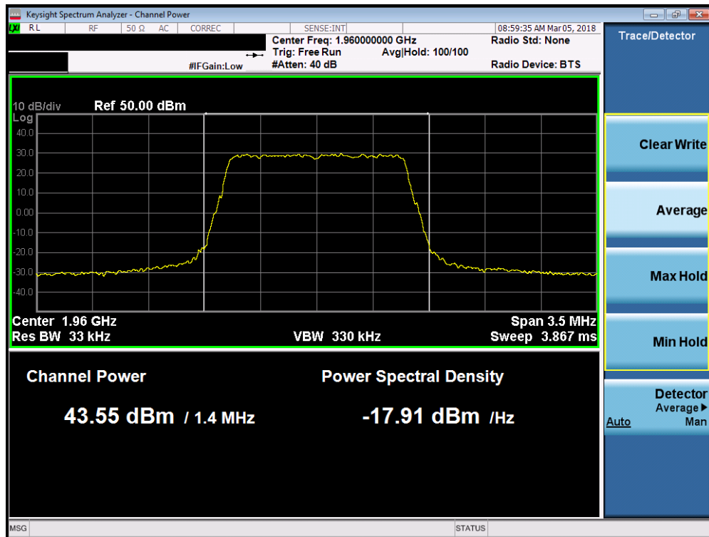
Plot 7-80. Maximum Conducted Power (Band 2 - 1.4MHz 64-QAM – Mid Channel)
