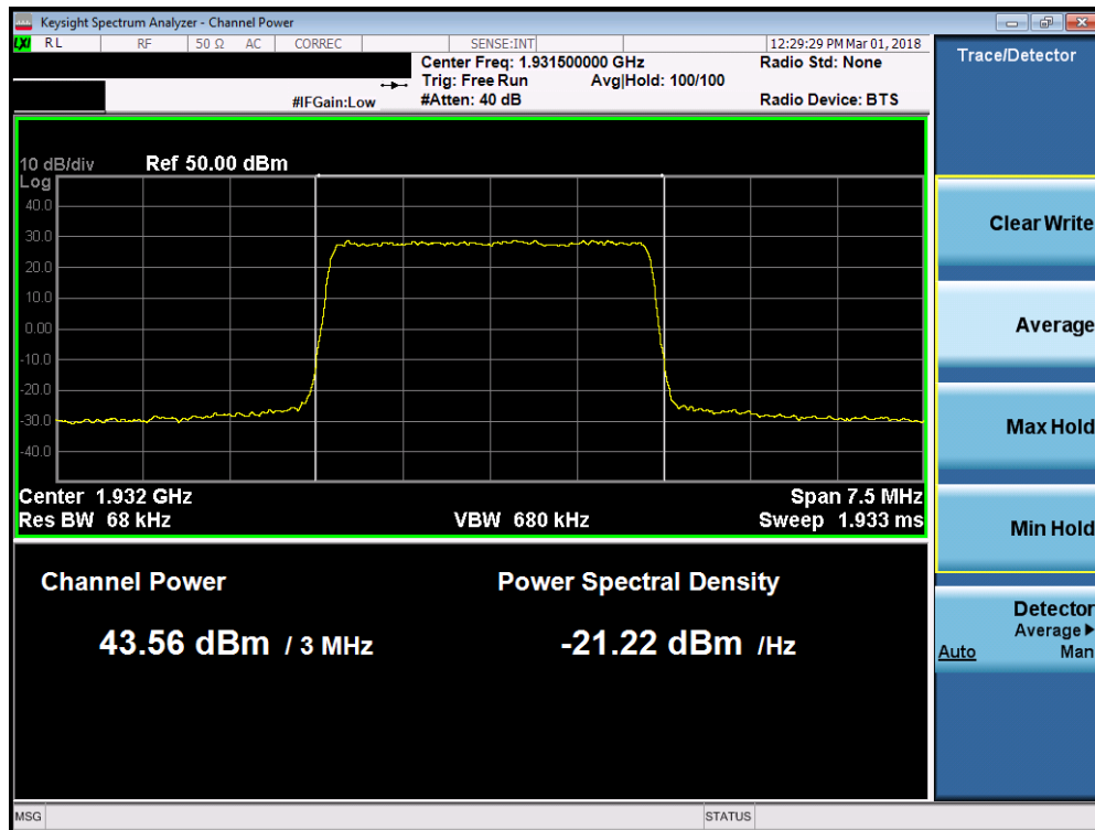
Plot 7-16. Maximum Conducted Power (Band 2 - 3.0MHz 16-QAM – Low Channel)
