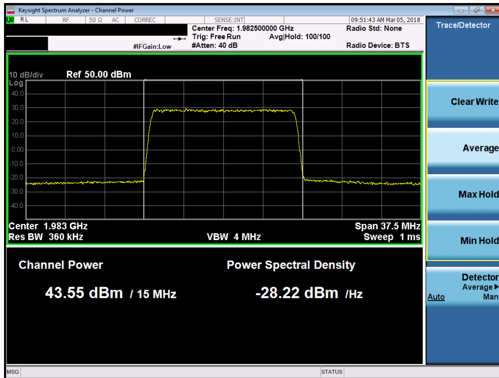
Plot 7-126. Maximum Conducted Power (Band 2 - 15.0MHz 16-QAM – High Channel)
