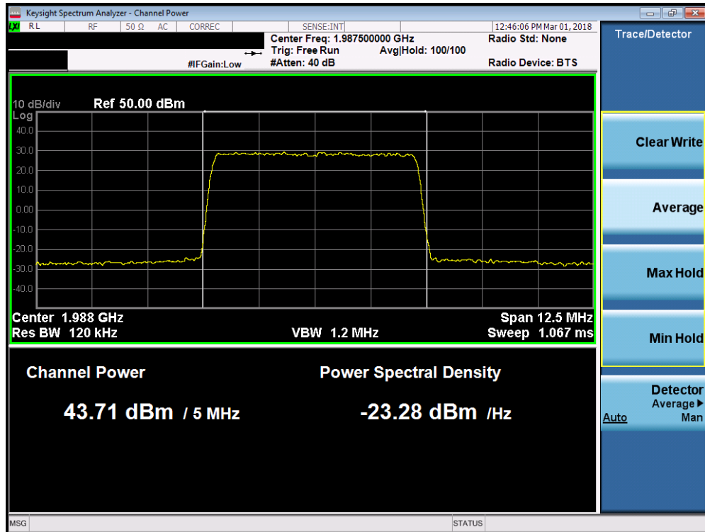
Plot 7-30. Maximum Conducted Power (Band 2 - 5.0MHz 16-QAM – High Channel)
