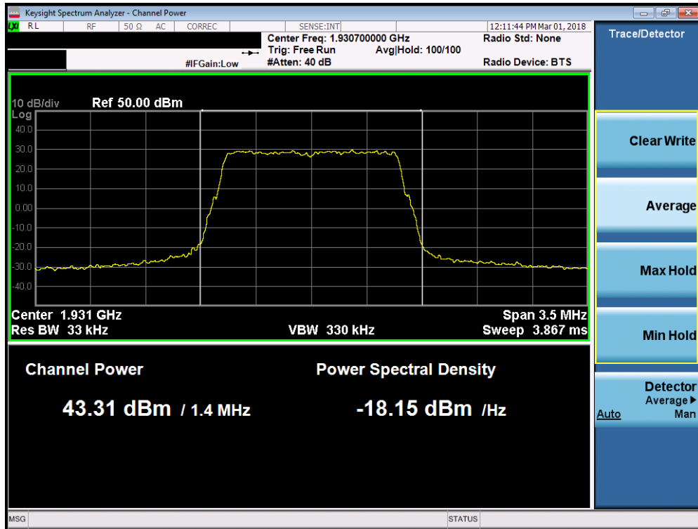
Plot 7-4. Maximum Conducted Power (Band 2 - 1.4MHz 16-QAM – Low Channel)
