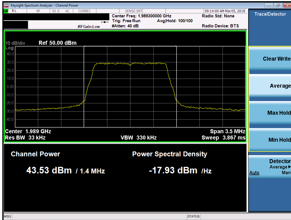
Plot 7-84. Maximum Conducted Power (Band 2 - 1.4MHz 256-QAM – High Channel)
