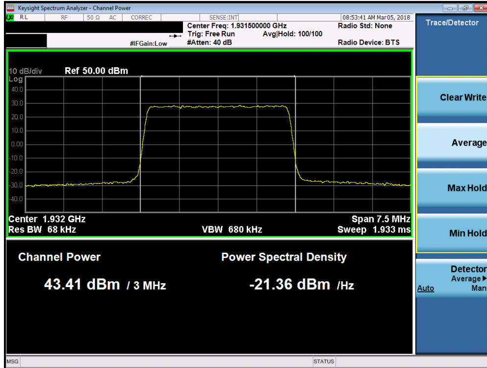
Plot 7-85. Maximum Conducted Power (Band 2 - 3.0MHz QPSK - Low Channel)
