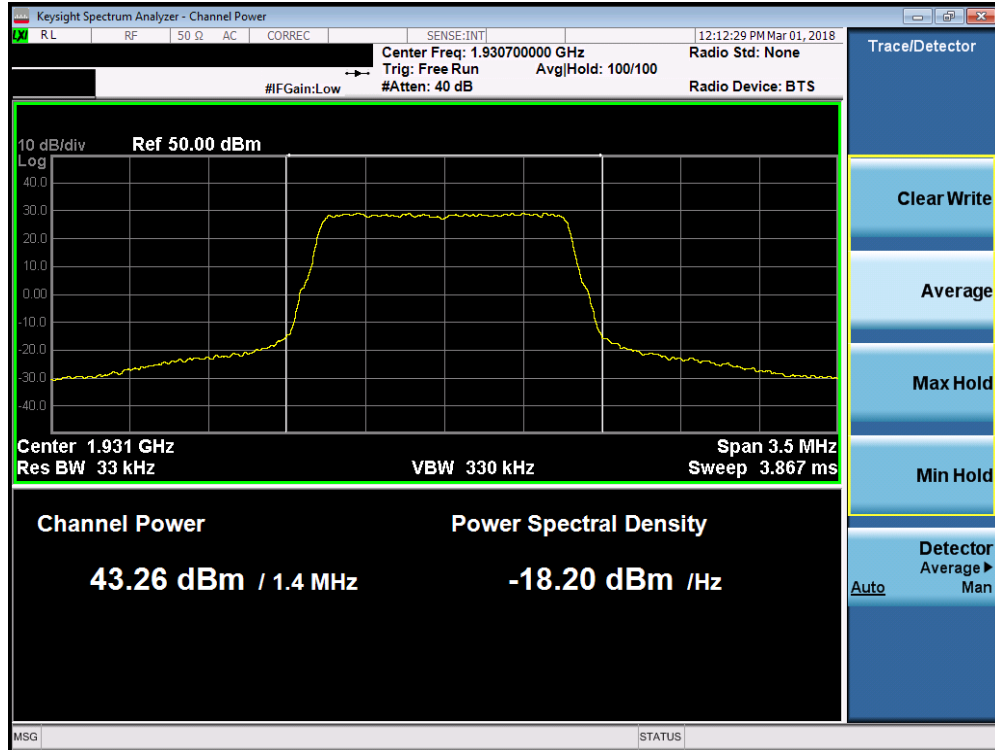
Plot 7-7. Maximum Conducted Power (Band 2 - 1.4MHz 64-QAM – Low Channel)
