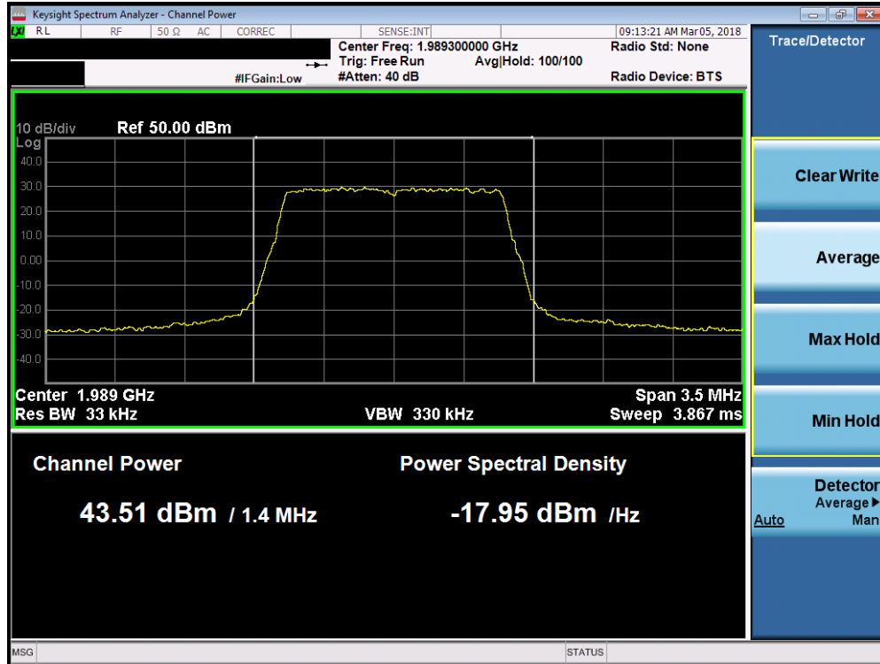
Plot 7-81. Maximum Conducted Power (Band 2 - 1.4MHz 64-QAM – High Channel)
