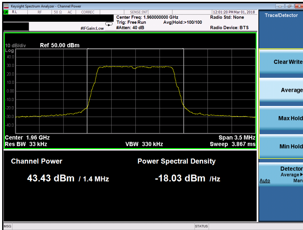
Plot 7-2. Maximum Conducted Power (Band 2 - 1.4MHz QPSK – Mid Channel)
