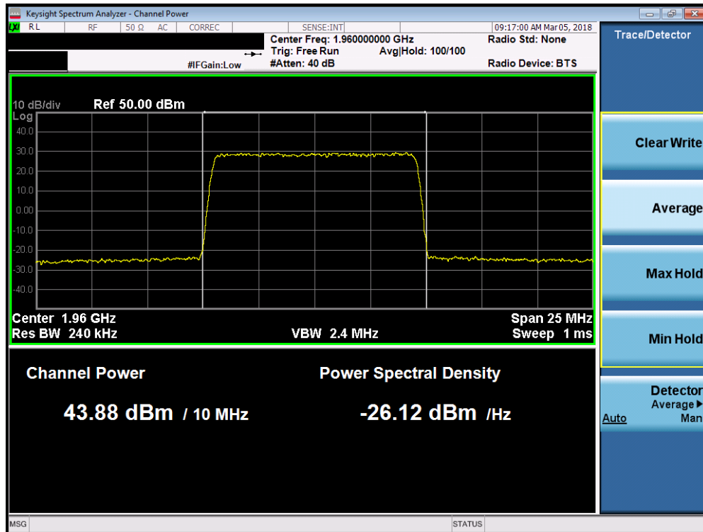
Plot 7-119. Maximum Conducted Power (Band 2 - 10.0MHz 256-QAM – Mid Channel)
