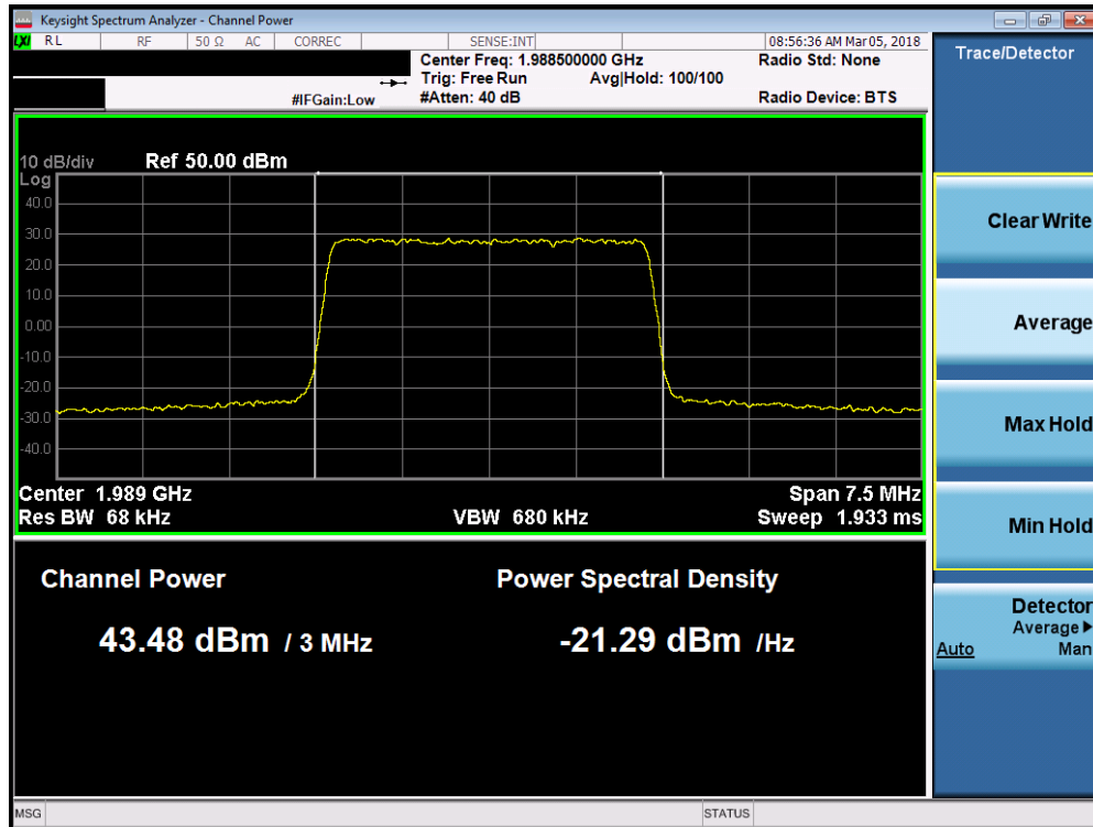
Plot 7-96. Maximum Conducted Power (Band 2 - 3.0MHz 256-QAM – High Channel)
