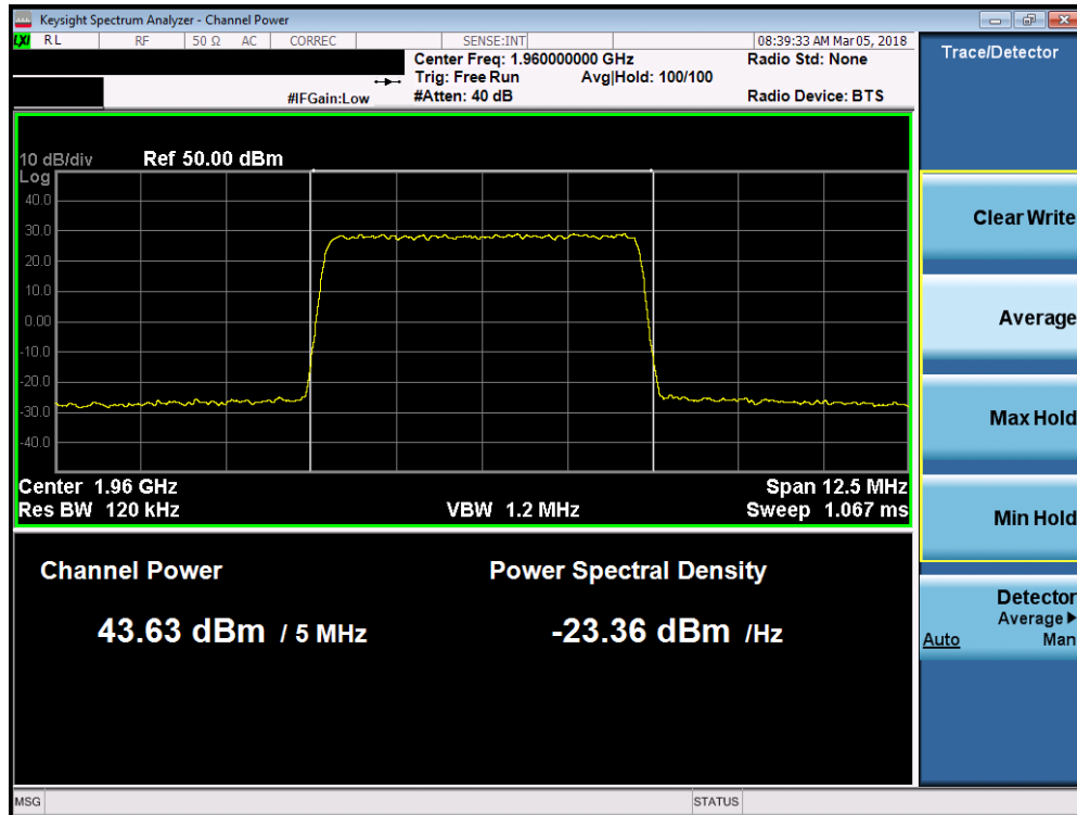
Plot 7-104. Maximum Conducted Power (Band 2 - 5.0MHz 64-QAM - Mid Channel)
