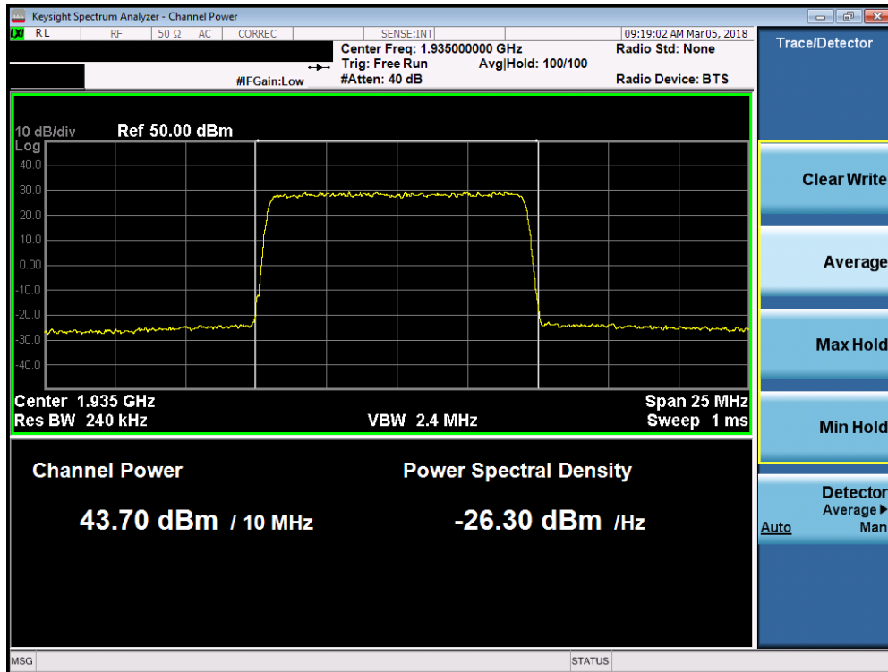
Plot 7-118. Maximum Conducted Power (Band 2 - 10.0MHz 256-QAM - Low Channel)
