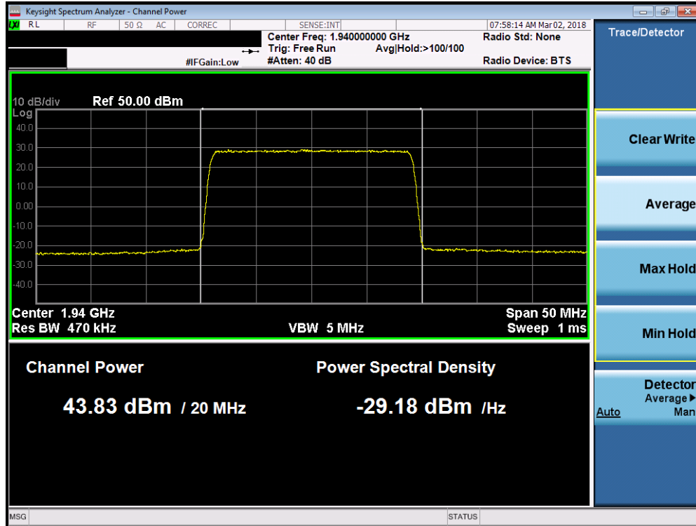
Plot 7-67. Maximum Conducted Power (Band 2 - 20.0MHz 64-QAM – Low Channel)
