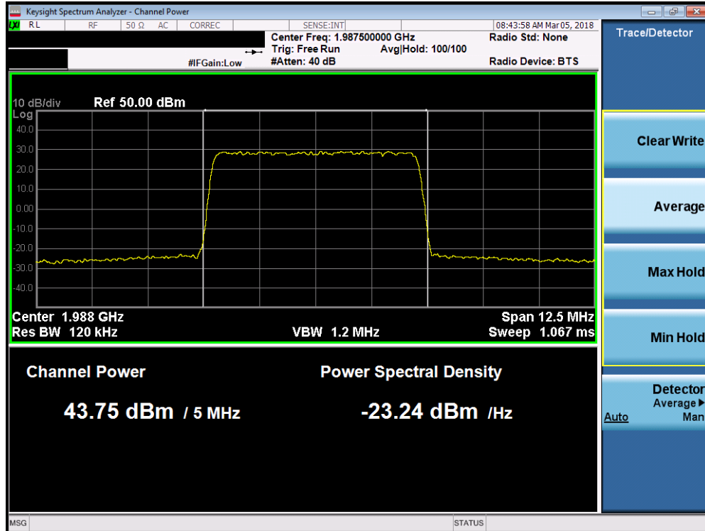
Plot 7-105. Maximum Conducted Power (Band 2 - 5.0MHz 64-QAM – High Channel)
