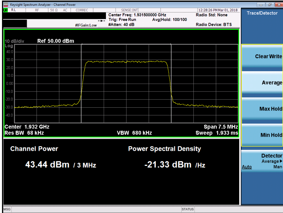
Plot 7-13. Maximum Conducted Power (Band 2 - 3.0MHz QPSK – Low Channel)
