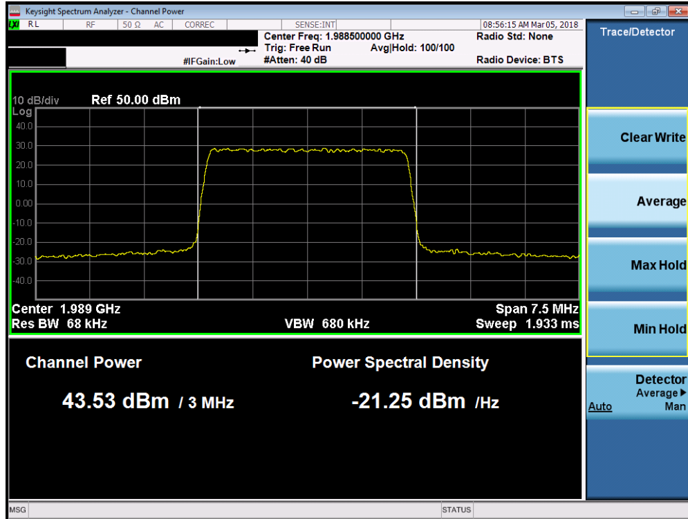
Plot 7-93. Maximum Conducted Power (Band 2 - 3.0MHz 64-QAM – High Channel)
