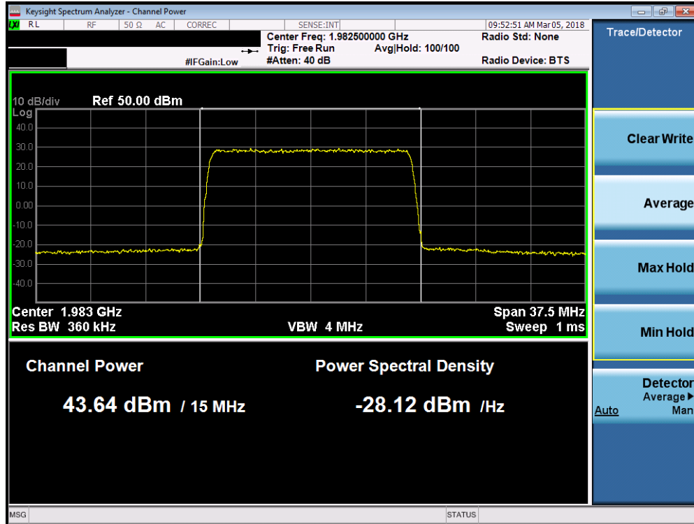
Plot 7-129. Maximum Conducted Power (Band 2 - 15.0MHz 64-QAM – High Channel)
