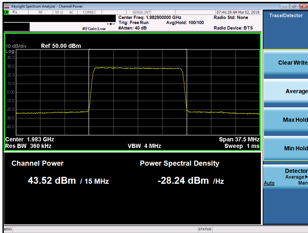
Plot 7-60. Maximum Conducted Power (Band 2 - 15.0MHz 256-QAM – High Channel)
