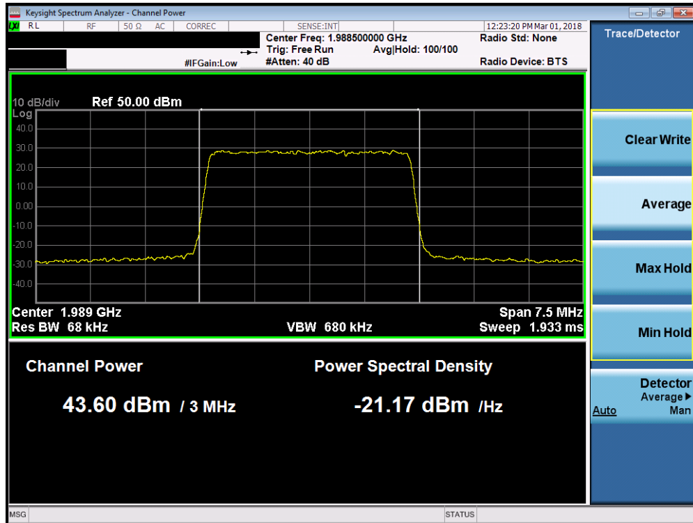
Plot 7-18. Maximum Conducted Power (Band 2 - 3.0MHz 16-QAM – High Channel)
