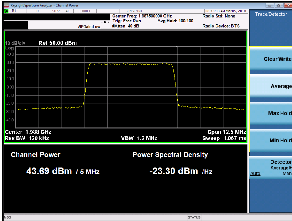
Plot 7-102. Maximum Conducted Power (Band 2 - 5.0MHz 16-QAM – High Channel)
