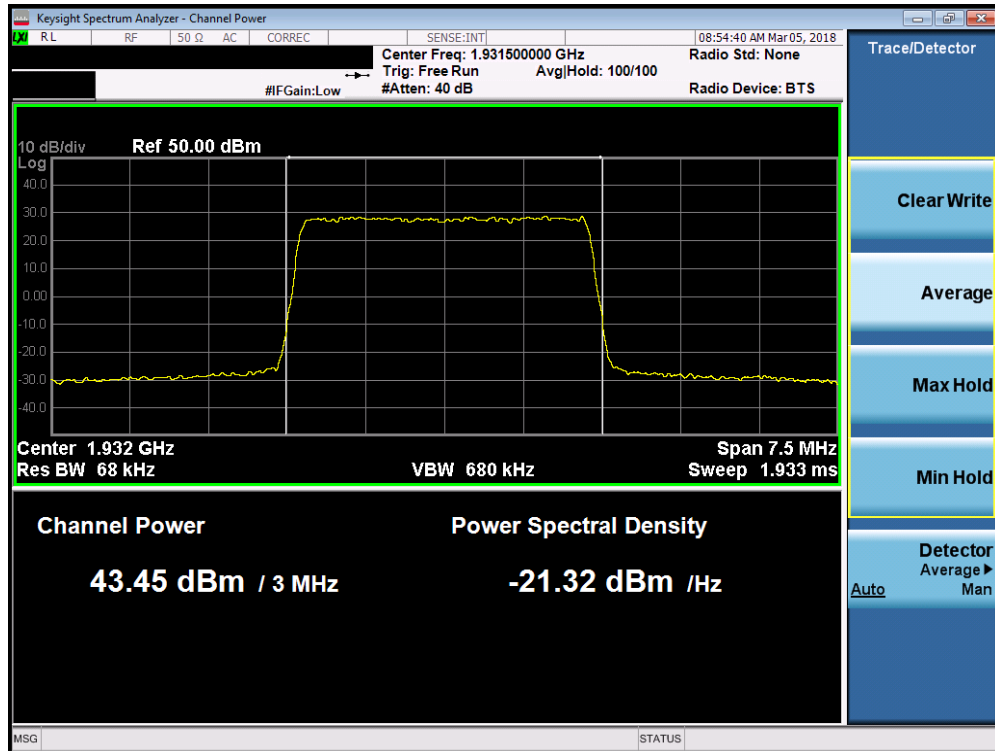
Plot 7-94. Maximum Conducted Power (Band 2 - 3.0MHz 256-QAM - Low Channel)
