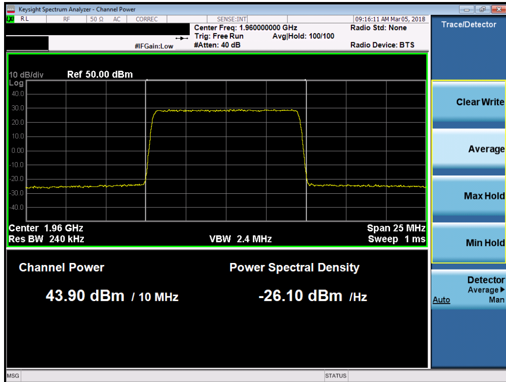
Plot 7-110. Maximum Conducted Power (Band 2 - 10.0MHz QPSK – Mid Channel)
