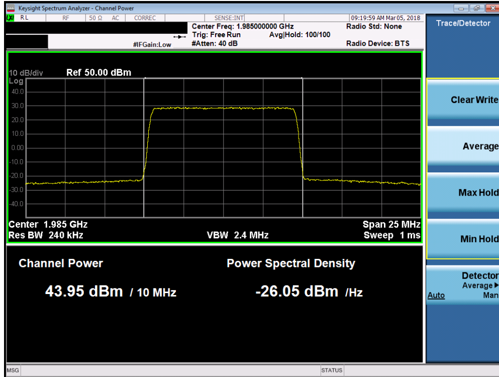
Plot 7-111. Maximum Conducted Power (Band 2 - 10.0MHz QPSK – High Channel)
