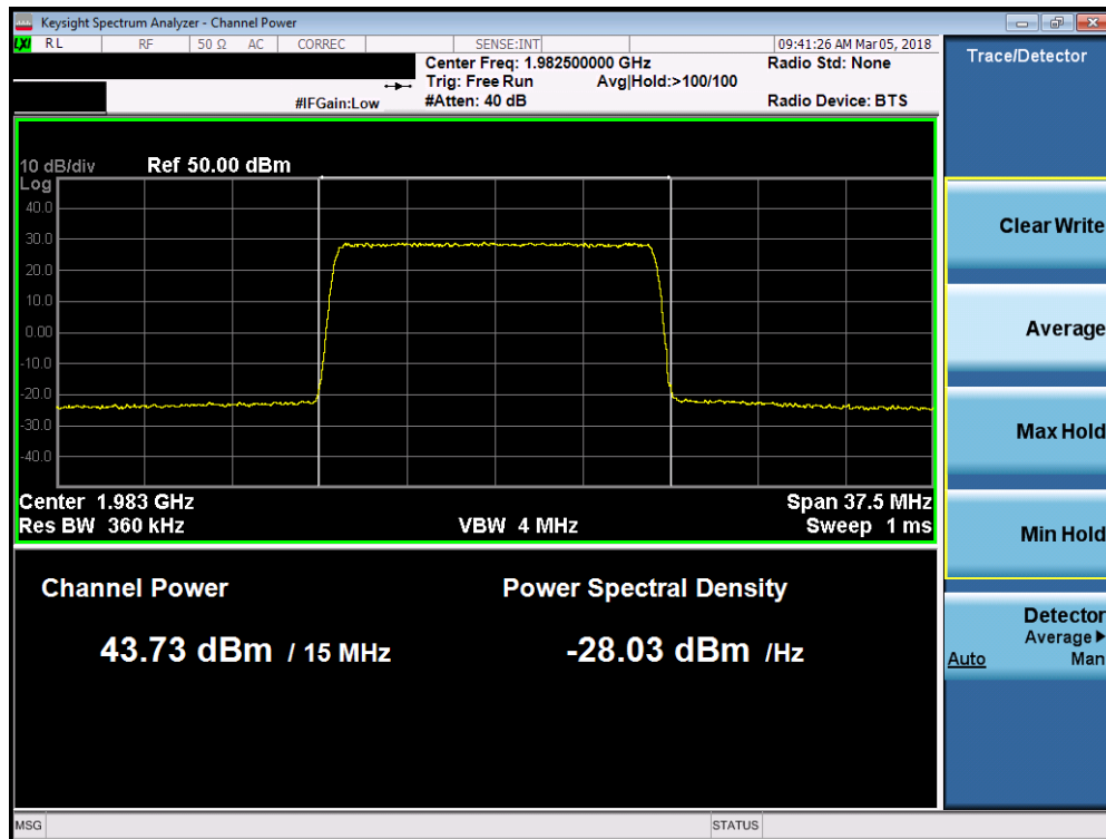
Plot 7-122. Maximum Conducted Power (Band 2 - 15.0MHz QPSK – Mid Channel)
