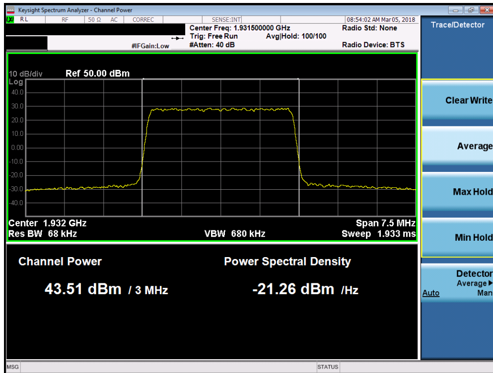
Plot 7-88. Maximum Conducted Power (Band 2 - 3.0MHz 16-QAM - Low Channel)
