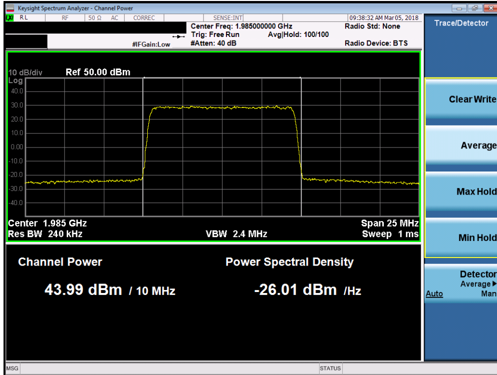
Plot 7-117. Maximum Conducted Power (Band 2 - 10.0MHz 64-QAM – High Channel)
