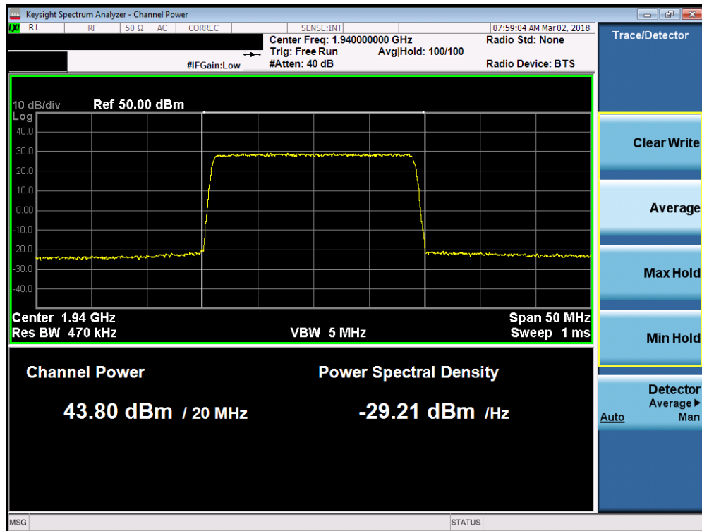
Plot 7-70. Maximum Conducted Power (Band 2 - 20.0MHz 256-QAM – Low Channel)
