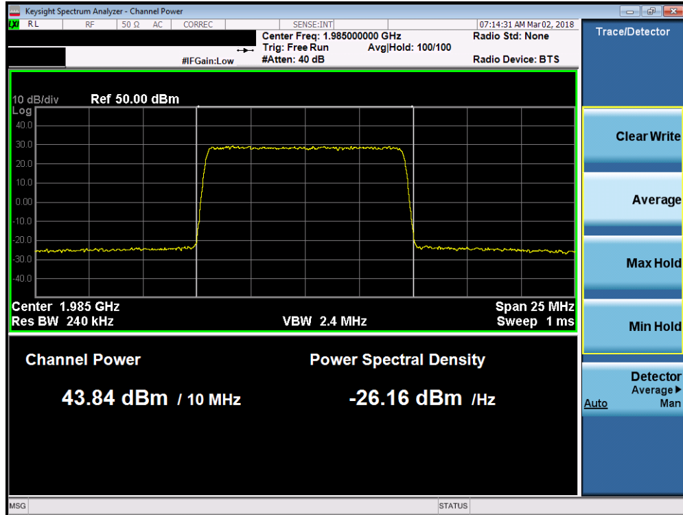
Plot 7-39. Maximum Conducted Power (Band 2 - 10.0MHz QPSK – High Channel)
