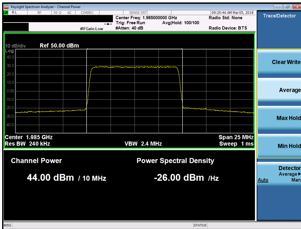
Plot 7-114. Maximum Conducted Power (Band 2 - 10.0MHz 16-QAM – High Channel)
