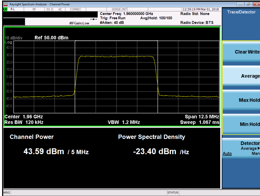
Plot 7-35. Maximum Conducted Power (Band 2 - 5.0MHz 256-QAM – Mid Channel)
