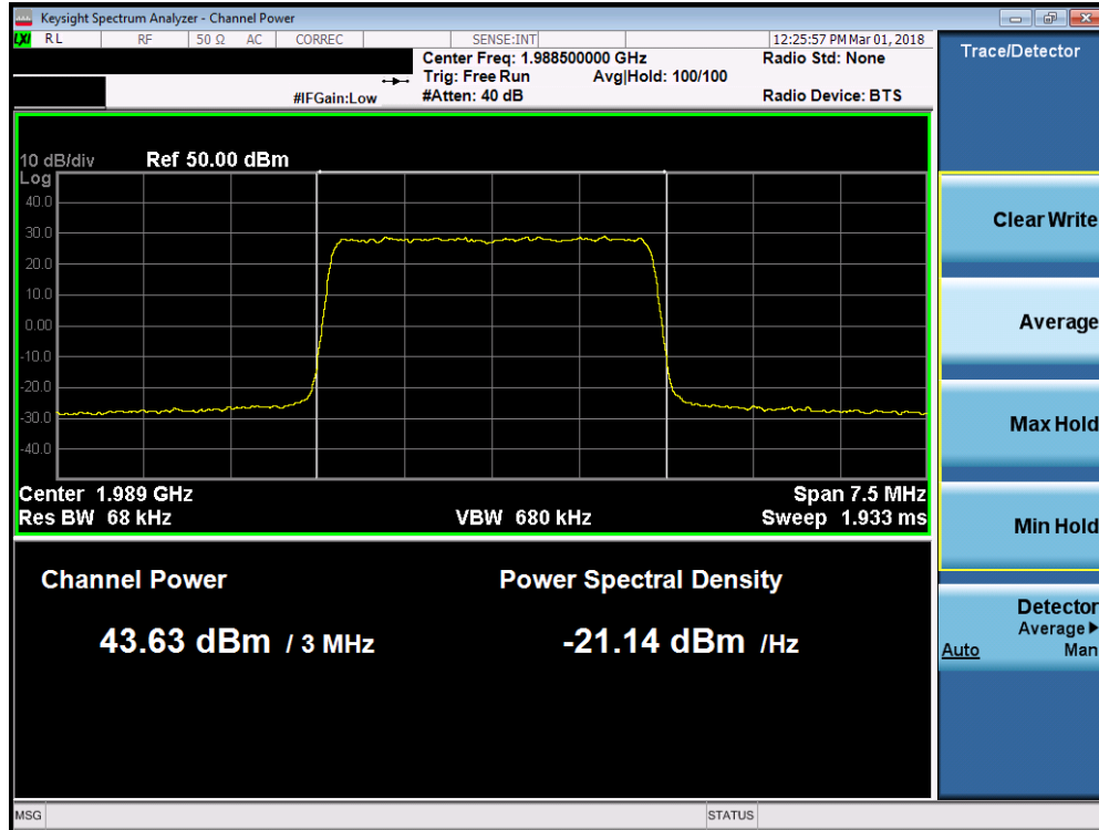
Plot 7-21. Maximum Conducted Power (Band 2 - 3.0MHz 64-QAM – High Channel)
