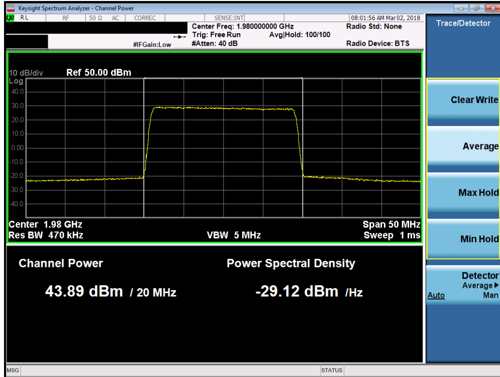
Plot 7-69. Maximum Conducted Power (Band 2 - 20.0MHz 64-QAM – High Channel)
