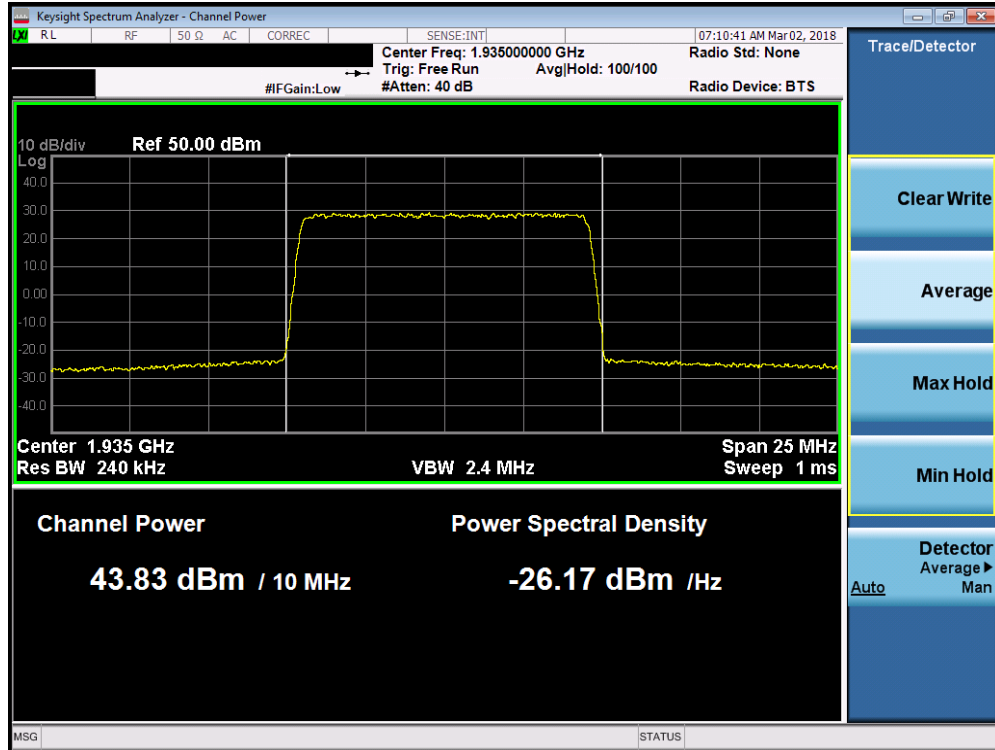
Plot 7-37. Maximum Conducted Power (Band 2 - 10.0MHz QPSK – Low Channel)
