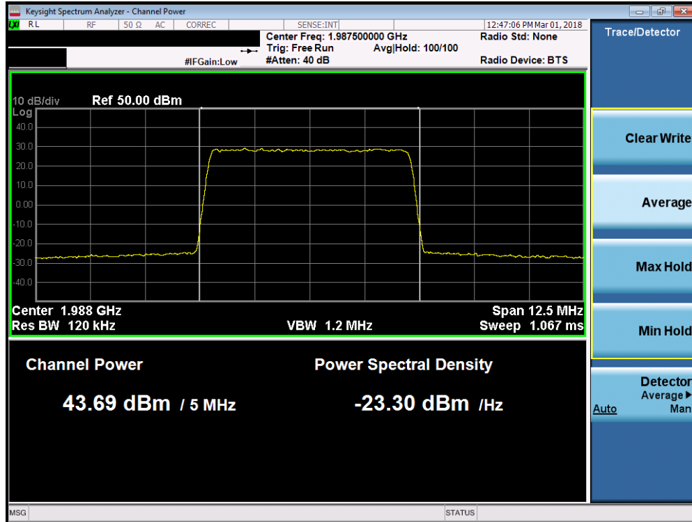
Plot 7-33. Maximum Conducted Power (Band 2 - 5.0MHz 64-QAM – High Channel)
