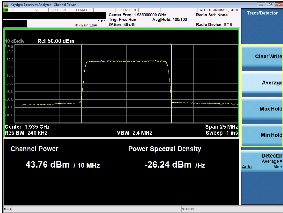
Plot 7-109. Maximum Conducted Power (Band 2 - 10.0MHz QPSK - Low Channel)
