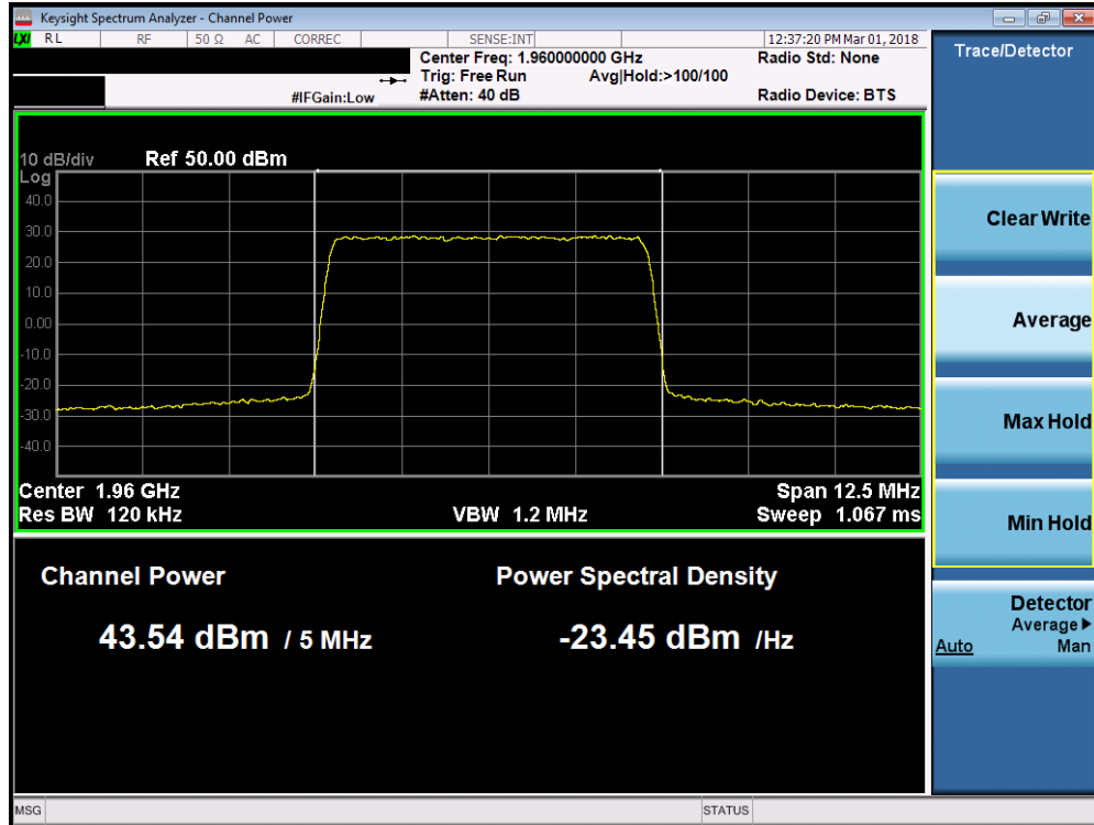
Plot 7-29. Maximum Conducted Power (Band 2 - 5.0MHz 16-QAM – Mid Channel)
