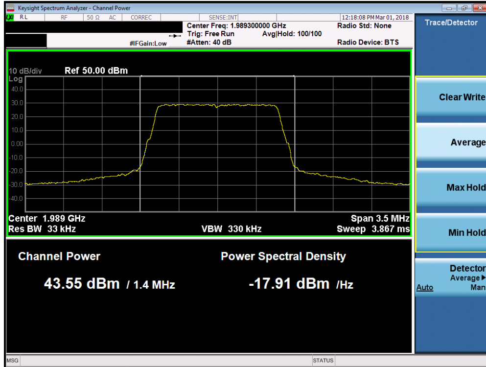
Plot 7-9. Maximum Conducted Power (Band 2 - 1.4MHz 64-QAM – High Channel)
