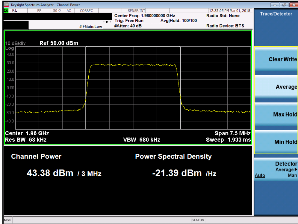
Plot 7-23. Maximum Conducted Power (Band 2 - 3.0MHz 256-QAM – Mid Channel)
