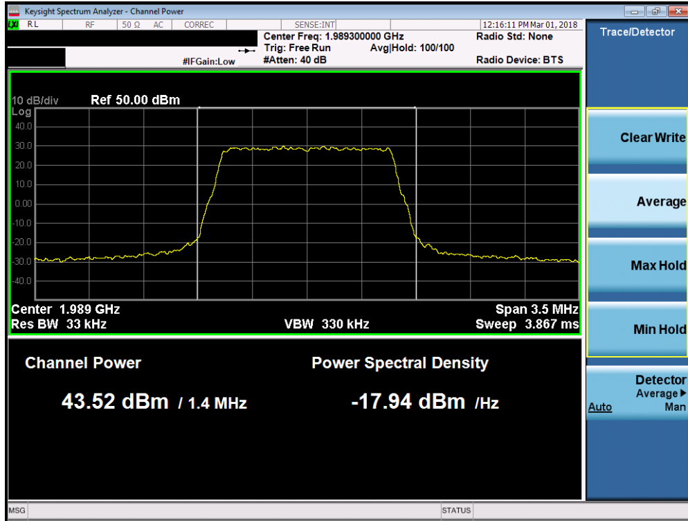
Plot 7-3. Maximum Conducted Power (Band 2 - 1.4MHz QPSK – High Channel)
