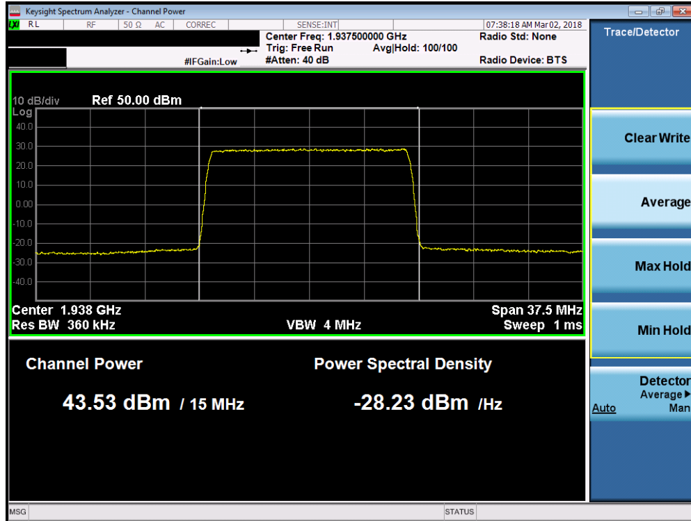
Plot 7-55. Maximum Conducted Power (Band 2 - 15.0MHz 64-QAM – Low Channel)
