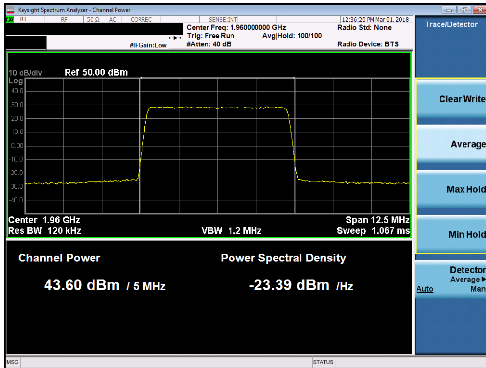
Plot 7-26. Maximum Conducted Power (Band 2 - 5.0MHz QPSK – Mid Channel)
