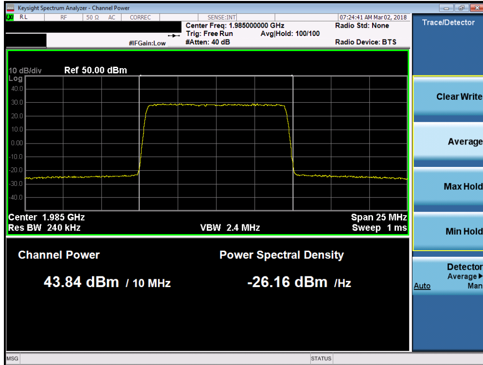
Plot 7-45. Maximum Conducted Power (Band 2 - 10.0MHz 64-QAM – High Channel)
