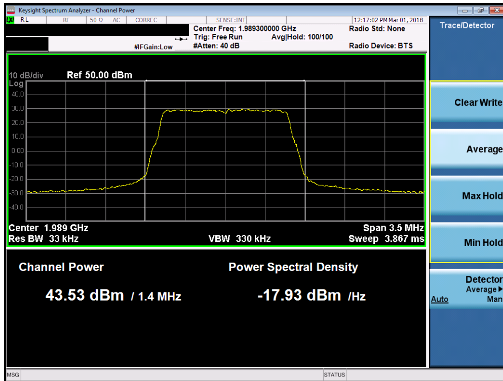
Plot 7-6. Maximum Conducted Power (Band 2 - 1.4MHz 16-QAM – High Channel)
