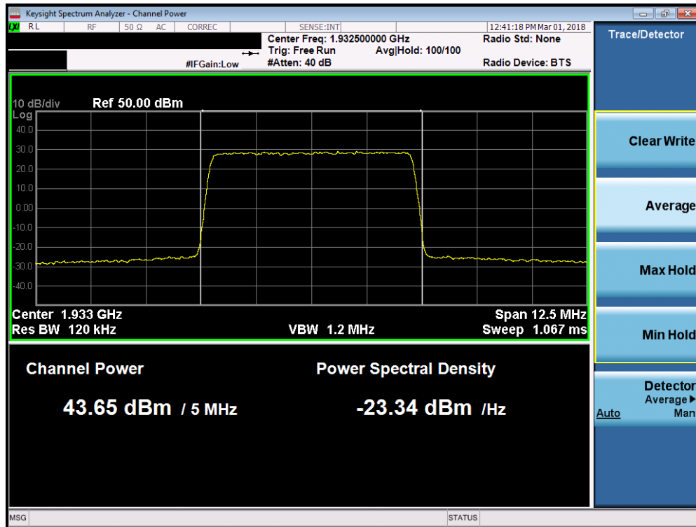
Plot 7-25. Maximum Conducted Power (Band 2 - 5.0MHz QPSK – Low Channel)
