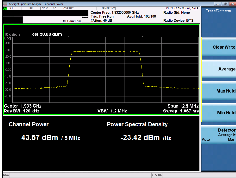
Plot 7-31. Maximum Conducted Power (Band 2 - 5.0MHz 64-QAM – Low Channel)
