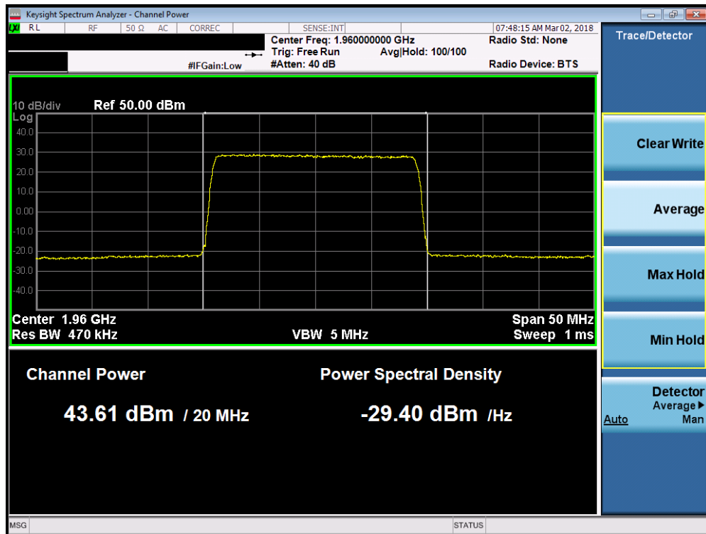
Plot 7-62. Maximum Conducted Power (Band 2 - 20.0MHz QPSK – Mid Channel)
