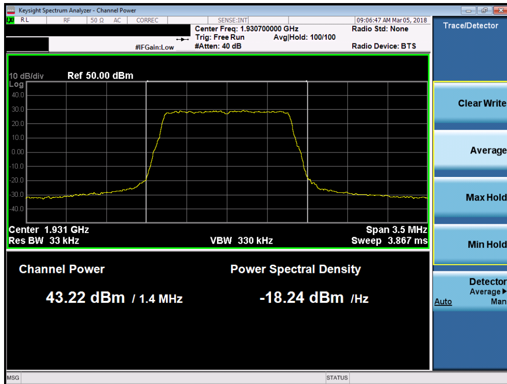
Plot 7-76. Maximum Conducted Power (Band 2 - 1.4MHz 16-QAM - Low Channel)
