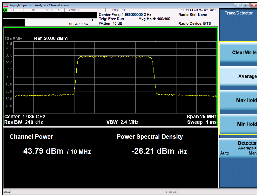
Plot 7-42. Maximum Conducted Power (Band 2 - 10.0MHz 16-QAM – High Channel)
