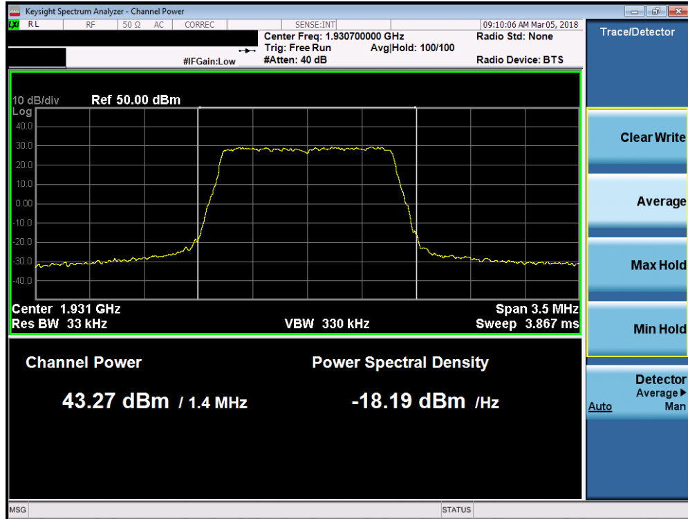
Plot 7-79. Maximum Conducted Power (Band 2 - 1.4MHz 64-QAM - Low Channel)
