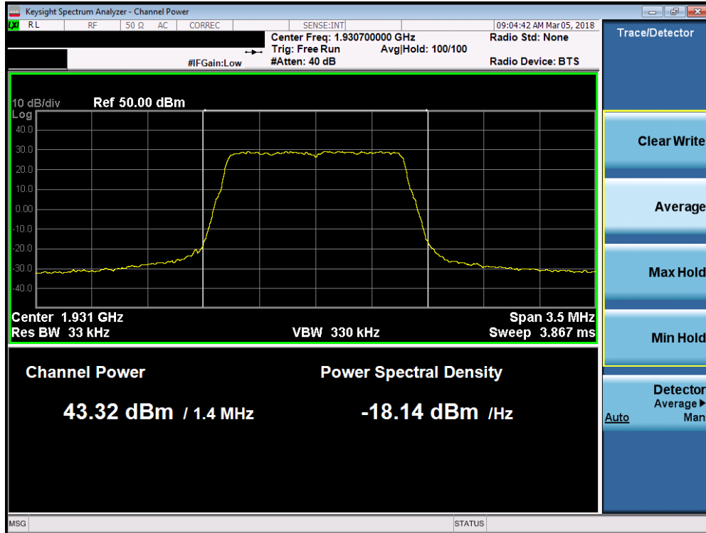
Plot 7-73. Maximum Conducted Power (Band 2 - 1.4MHz QPSK - Low Channel)
