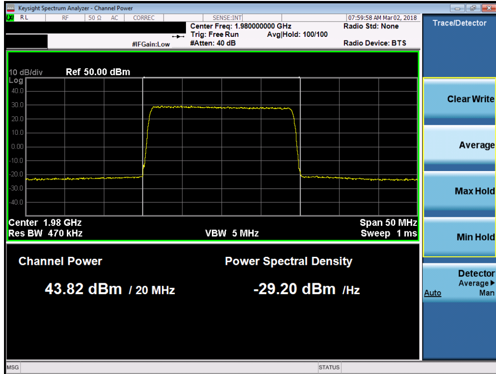
Plot 7-63. Maximum Conducted Power (Band 2 - 20.0MHz QPSK – High Channel)
