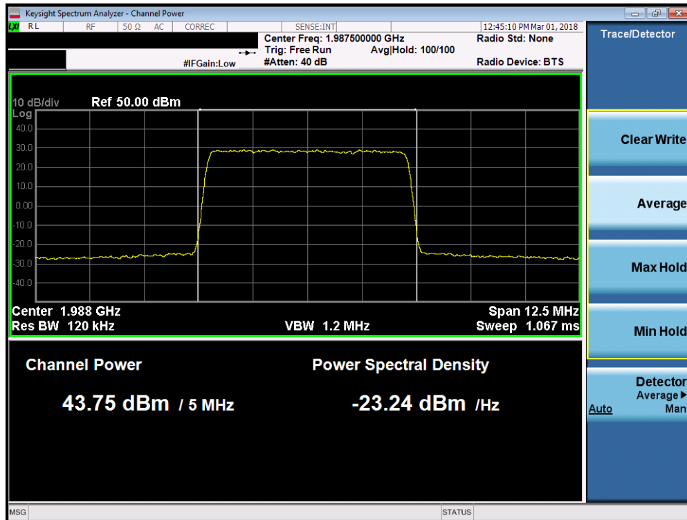
Plot 7-27. Maximum Conducted Power (Band 2 - 5.0MHz QPSK – High Channel)
