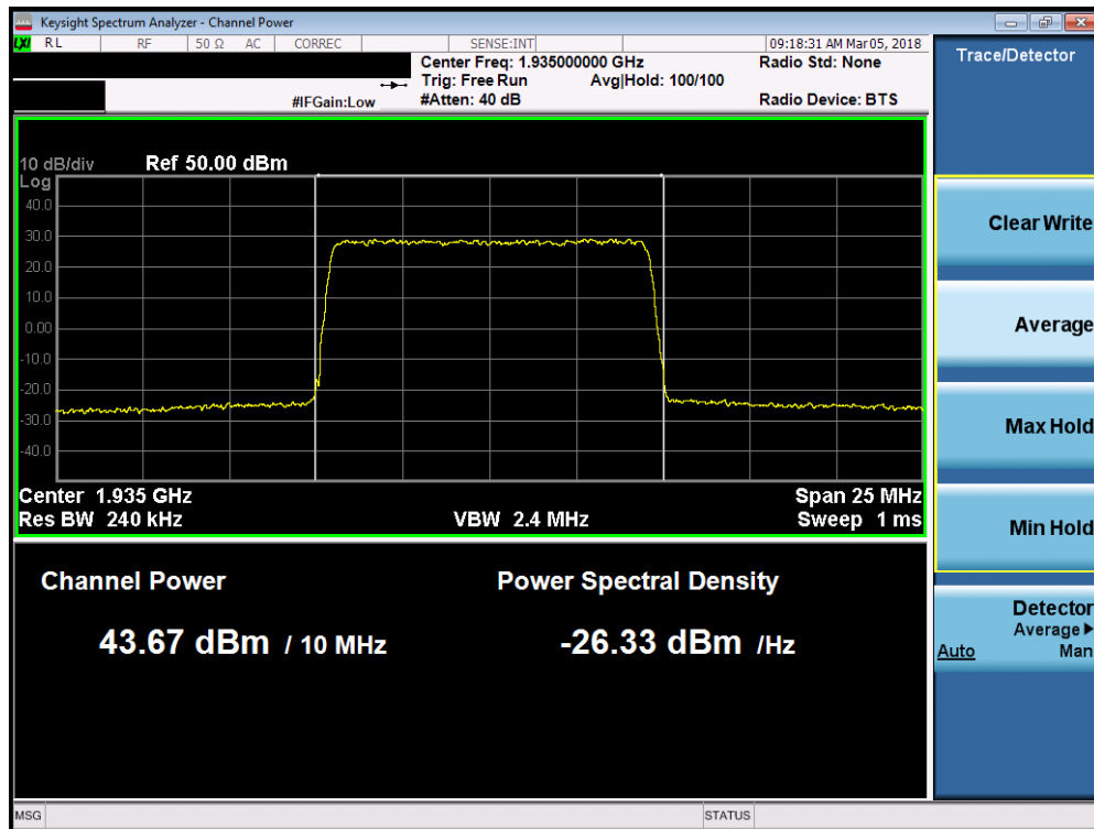
Plot 7-112. Maximum Conducted Power (Band 2 - 10.0MHz 16-QAM - Low Channel)
