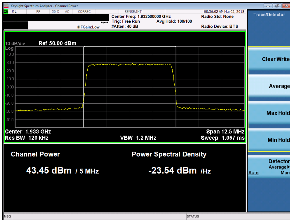
Plot 7-100. Maximum Conducted Power (Band 2 - 5.0MHz 16-QAM - Low Channel)
