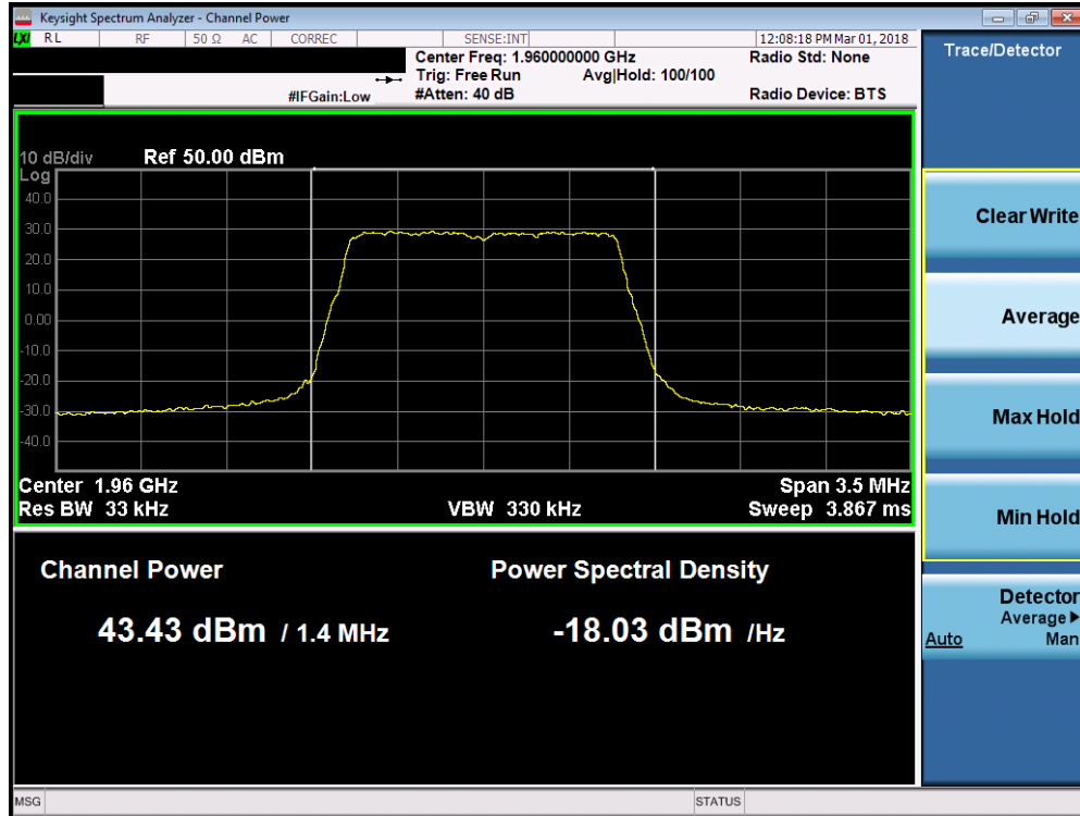
Plot 7-11. Maximum Conducted Power (Band 2 - 1.4MHz 256-QAM – Mid Channel)
