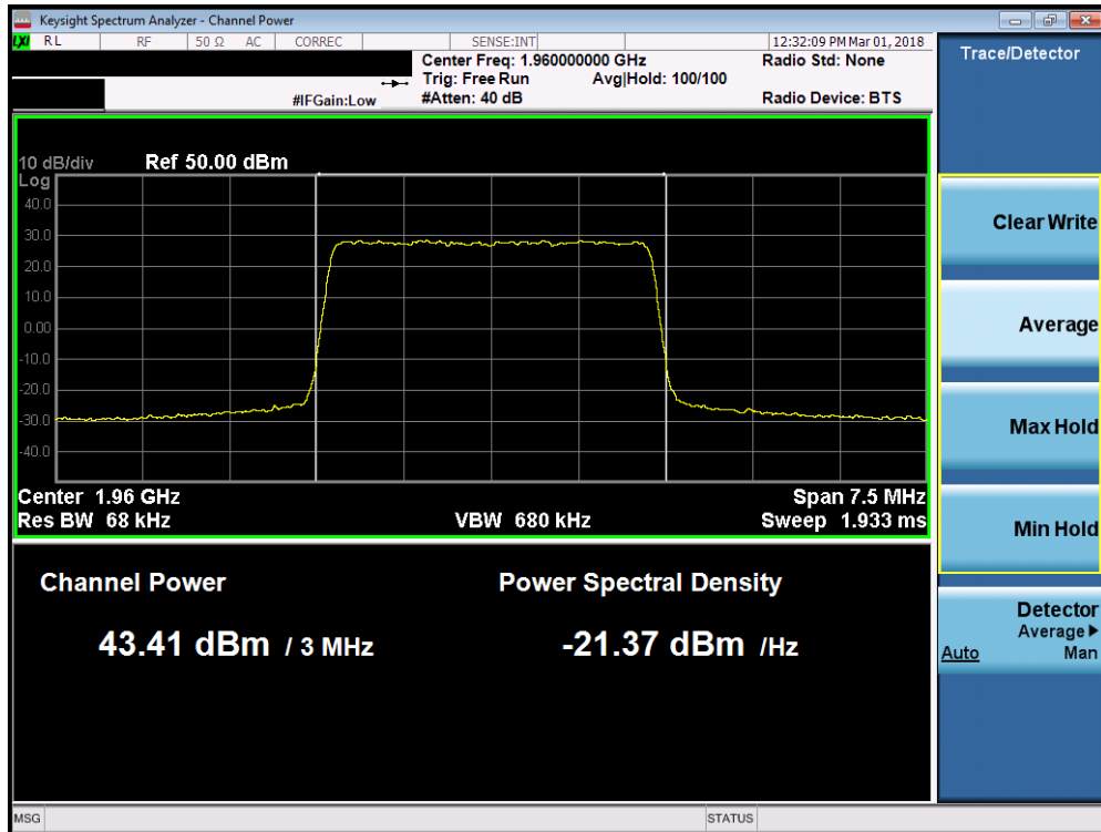
Plot 7-14. Maximum Conducted Power (Band 2 - 3.0MHz QPSK – Mid Channel)
