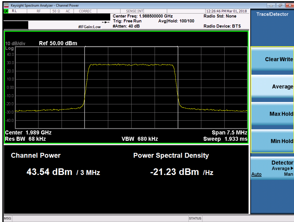
Plot 7-24. Maximum Conducted Power (Band 2 - 3.0MHz 256-QAM – High Channel)
