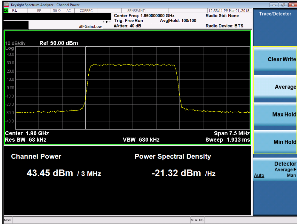
Plot 7-17. Maximum Conducted Power (Band 2 - 3.0MHz 16-QAM – Mid Channel)
