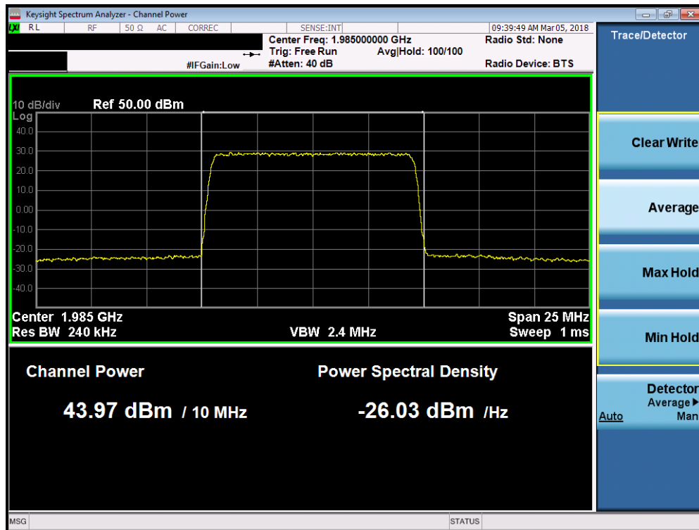
Plot 7-120. Maximum Conducted Power (Band 2 - 10.0MHz 256-QAM – High Channel)
