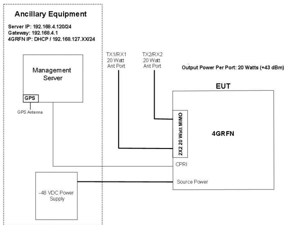
Figure 2-1. Test Setup
