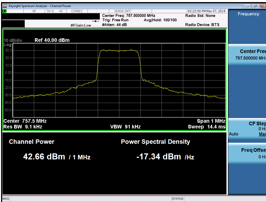
Plot 7-15. Max Conducted Power Plot (757.5 - 200 kHz - QPSK – ANT1 MIMO)
