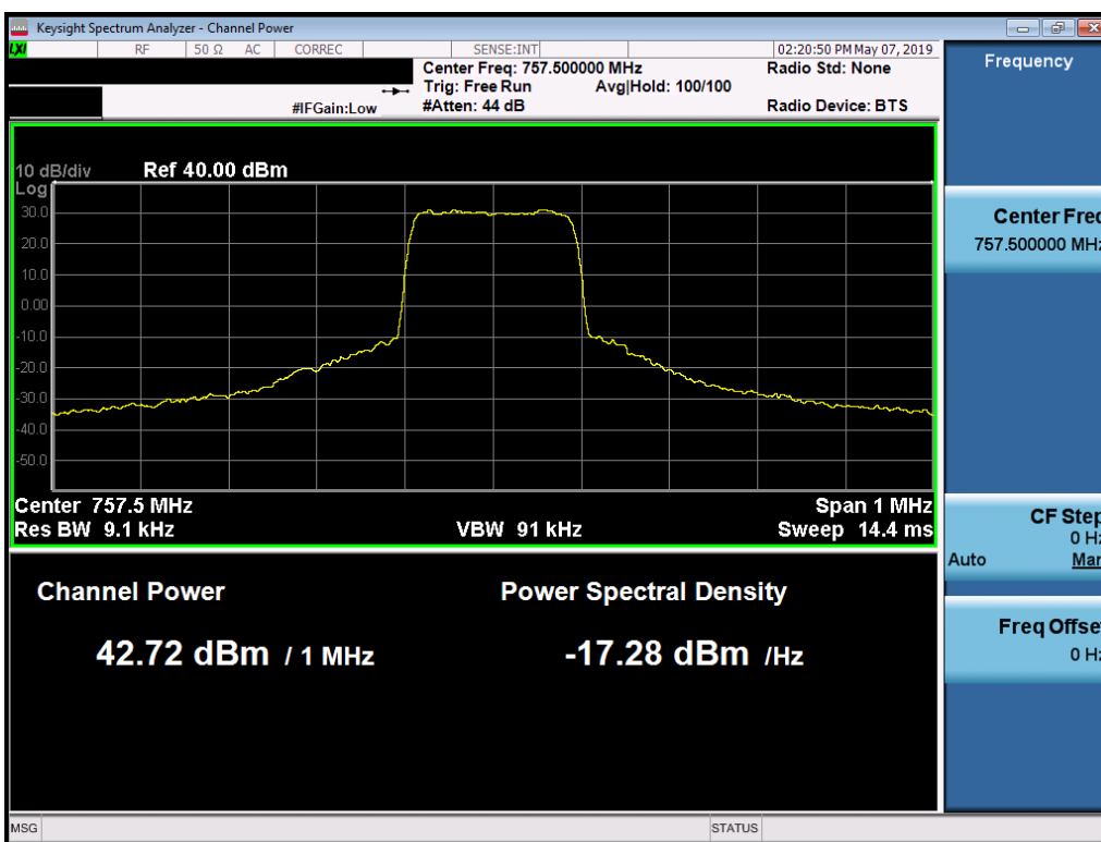
Plot 7-3. Max Conducted Power Plot (757.5 - 200 kHz - QPSK - ANT1 SISO)
