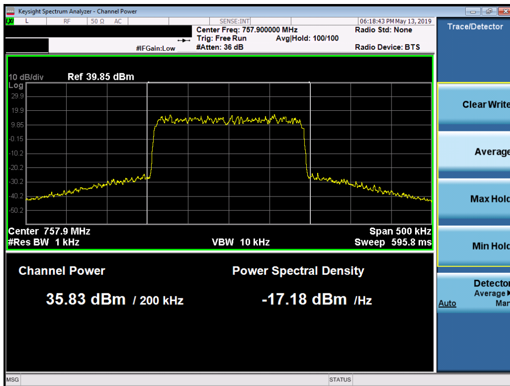
Plot 7-5. Max Conducted Power Plot (757.9 - 200 kHz - QPSK - ANT1 SISO)
