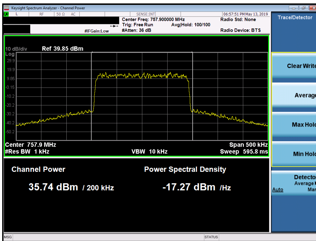
Plot 7-10. Max Conducted Power Plot (757.9 - 200 kHz - QPSK – ANT2 SISO)
