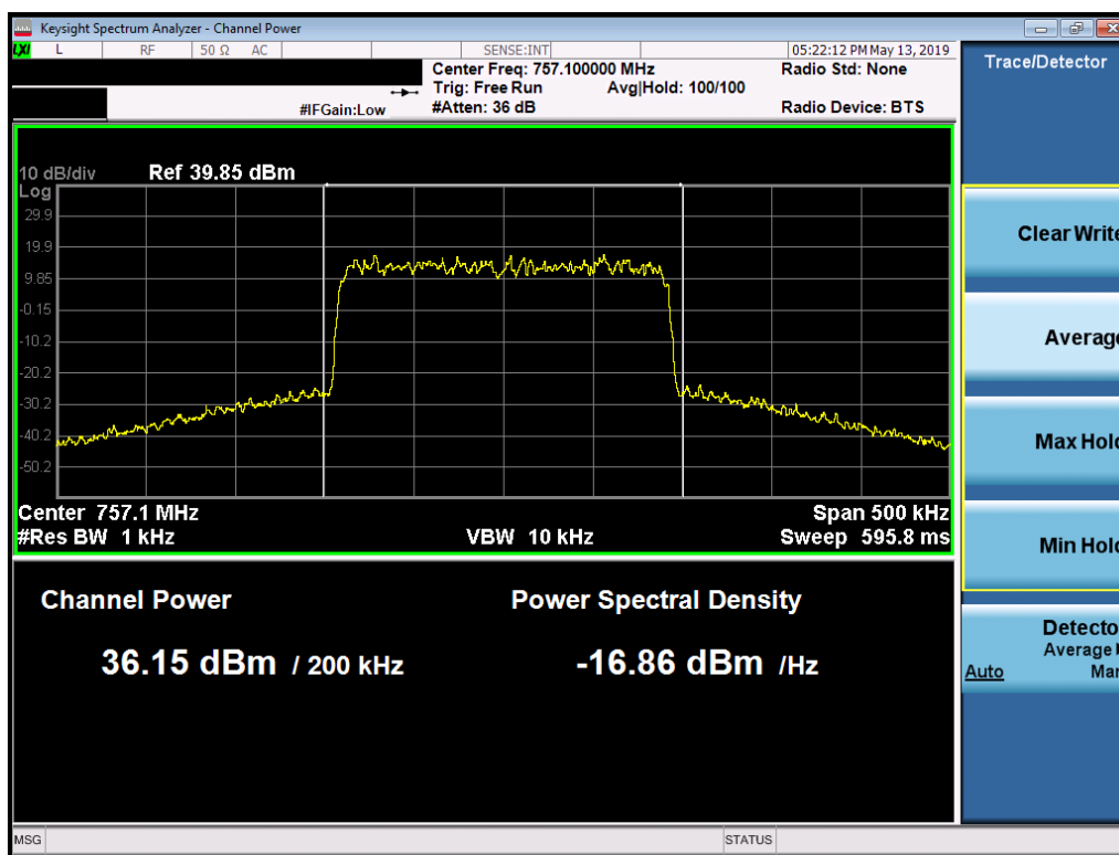
Plot 7-6. Max Conducted Power Plot (757.1 - 200 kHz - QPSK – ANT2 SISO)
