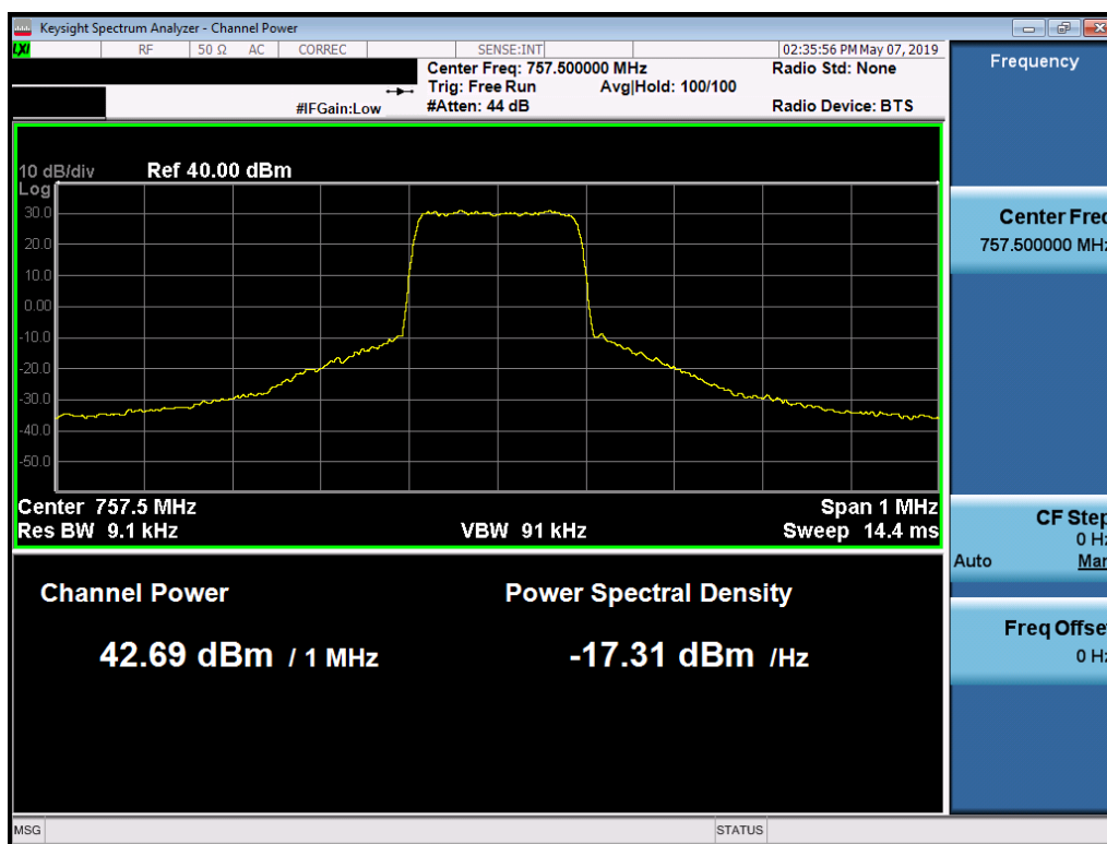
Plot 7-8. Max Conducted Power Plot (757.5 - 200 kHz - QPSK – ANT2 SISO)
