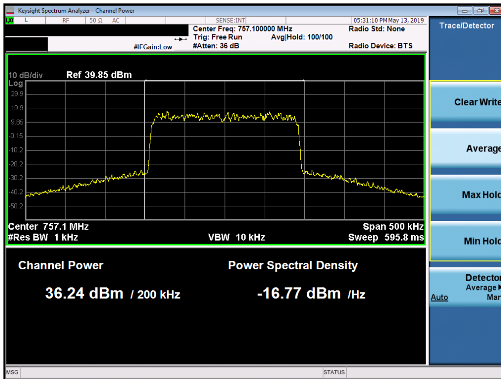
Plot 7-1. Max Conducted Power Plot (757.1 - 200 kHz - QPSK - ANT1 SISO)
