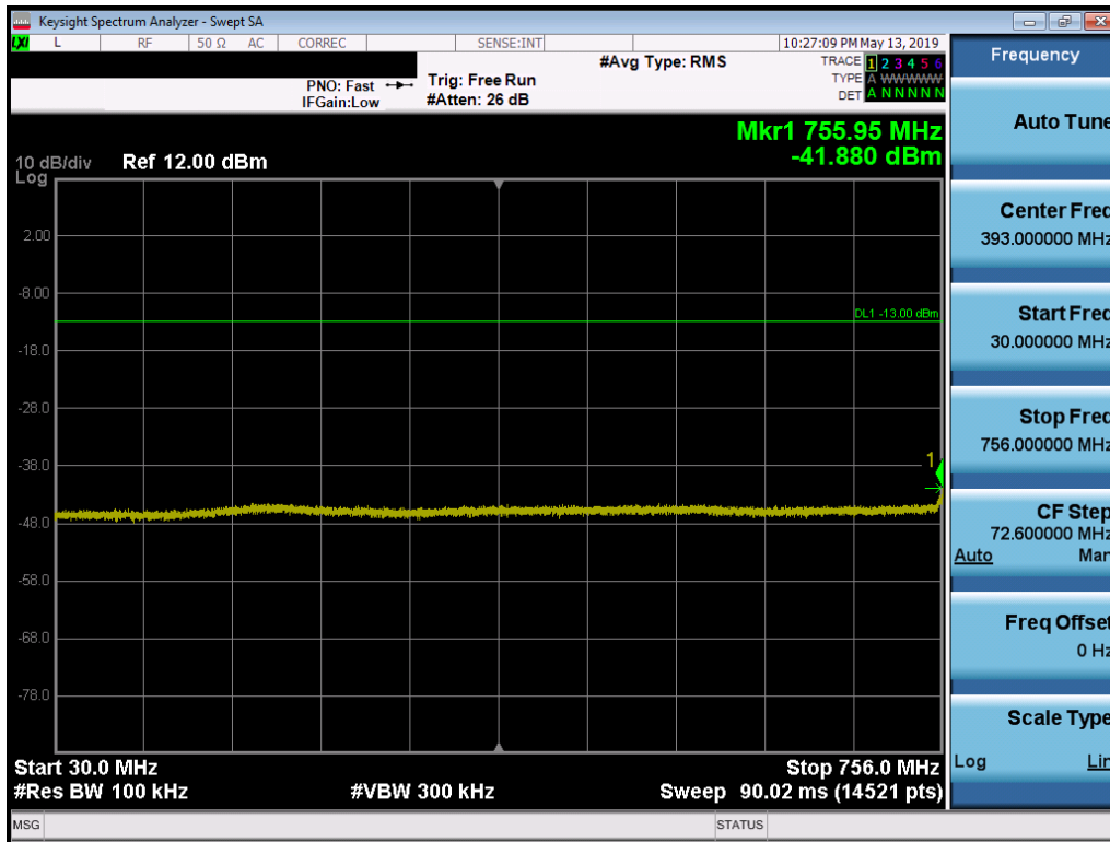
Plot 7-23. Conducted Spurious Plot (200kHz QPSK – Low Channel)
