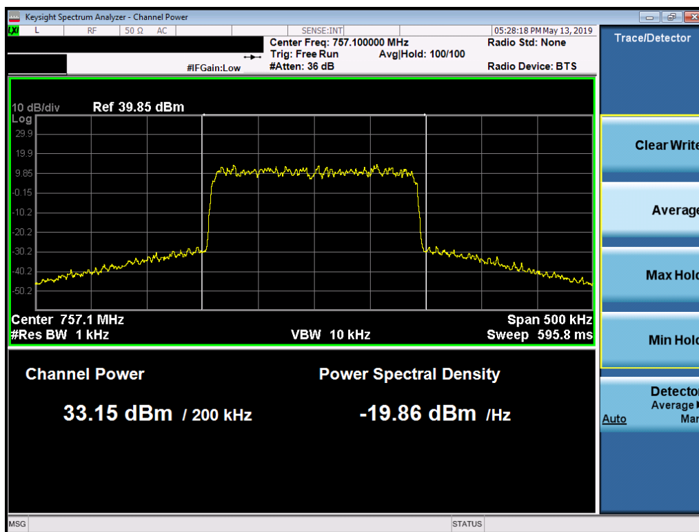
Plot 7-11. Max Conducted Power Plot (757.1 - 200 kHz - QPSK – ANT1 MIMO)
