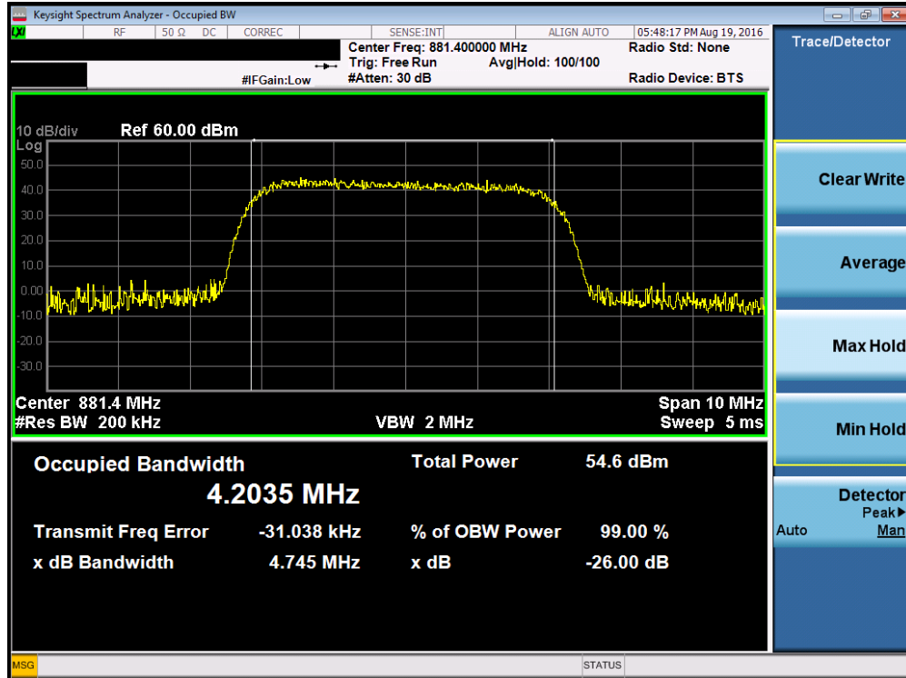
Plot 7-1. Occupied Bandwidth Plot (Cellular UMTS Mode – Ch. 4407 - QPSK)
