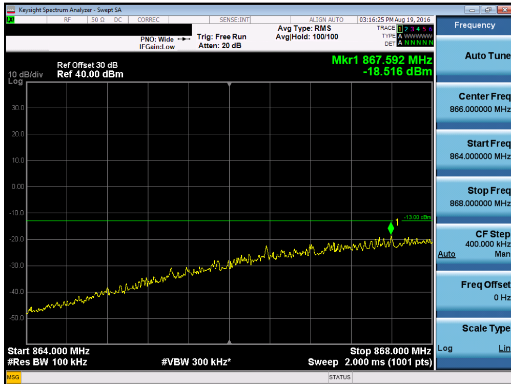
Plot 7-14. 4MHz Span Plot (Cellular UMTS Mode – Ch. 4357)
