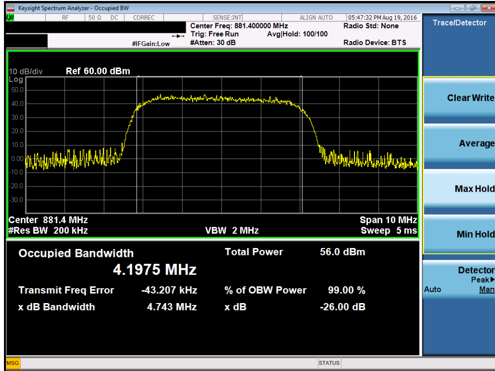
Plot 7-3. Occupied Bandwidth Plot (Cellular UMTS Mode – Ch. 4407 – 64-QAM)
