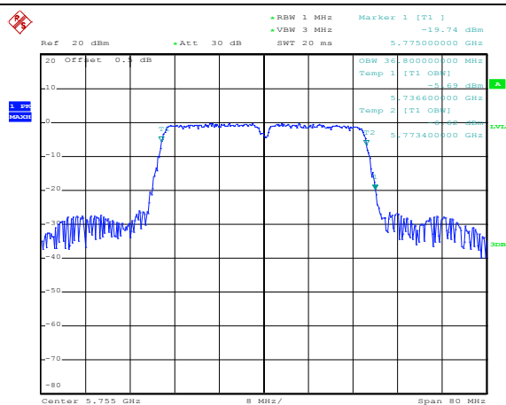
802.11n HT40_Low Channel / 5755MHz
