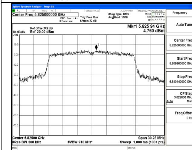
802.11a_High Channel / 5825MHz
