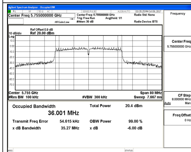
802.11n HT40_Low Channel / 5755MHz
