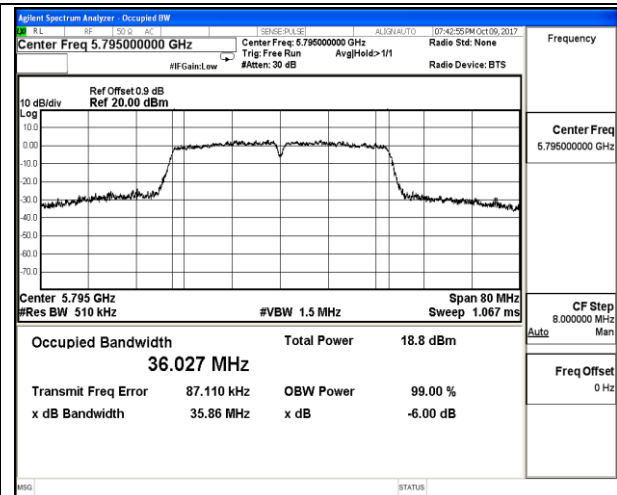
802.11n HT40_High Channel / 5795MHz
