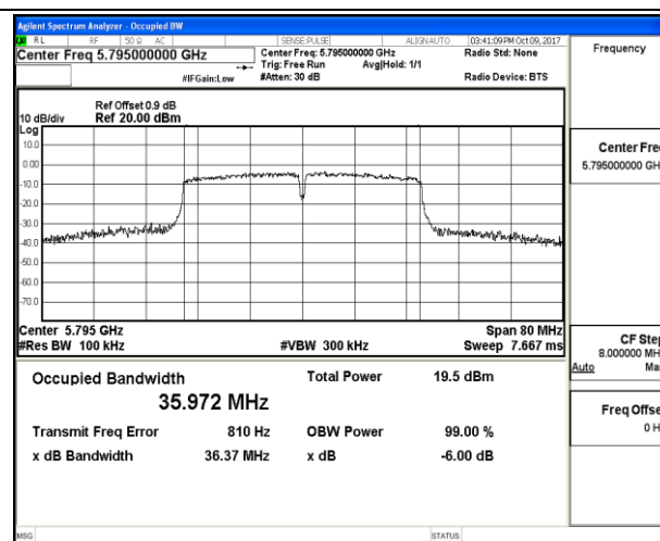
802.11n HT40_High Channel / 5795MHz
