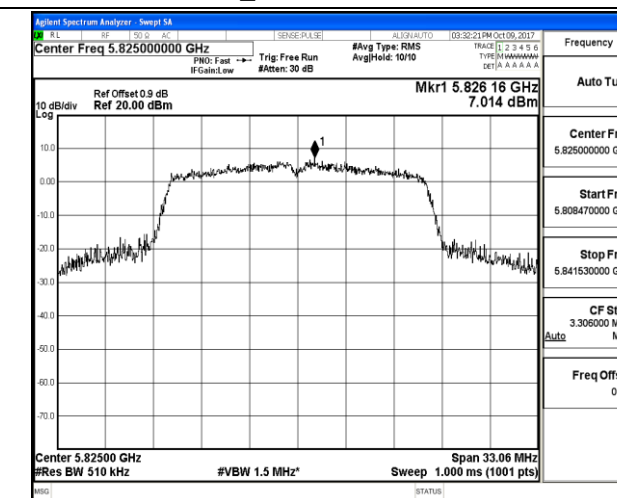
802.11n HT20_High Channel / 5825MHz
