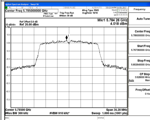
802.11a_Middle Channel / 5785MHz
