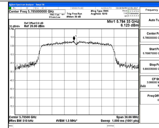
802.11n HT20_Middle Channel / 5785MHz
