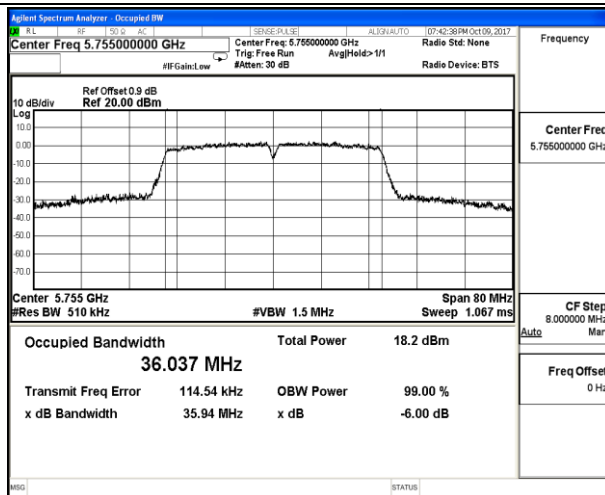
802.11n HT40_Low Channel / 5755MHz
