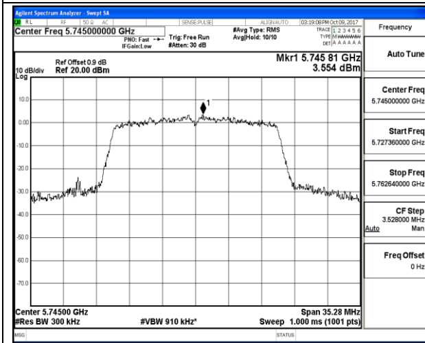
802.11a_Low Channel / 5745MHz
