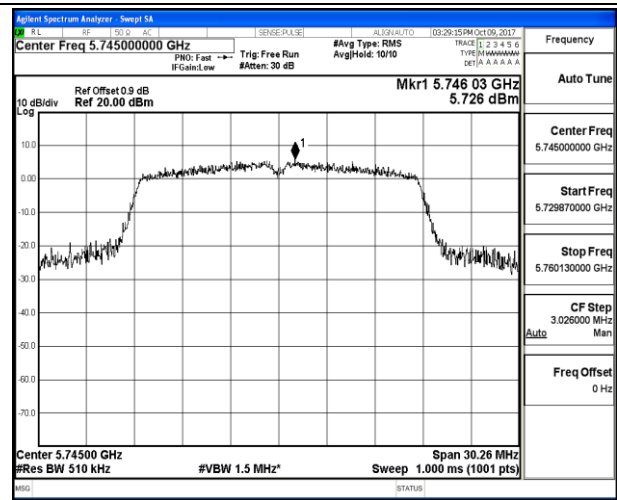
802.11n HT20_Low Channel / 5745MHz
