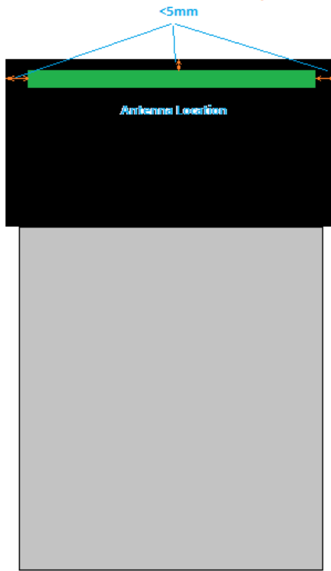
Antenna Location of Horizontal-Up View
