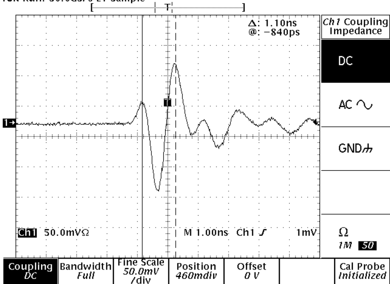
Figure 1. Pulse characteristic of a 500 MHz UWB-unit.
