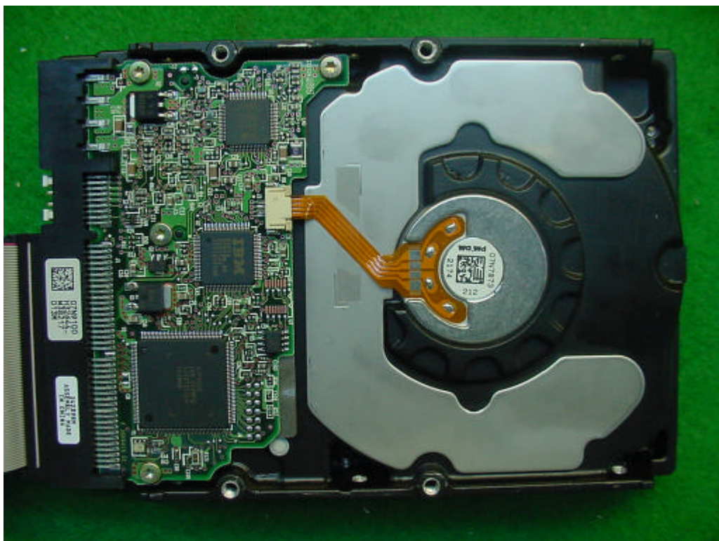
STORAGE (REAR)
