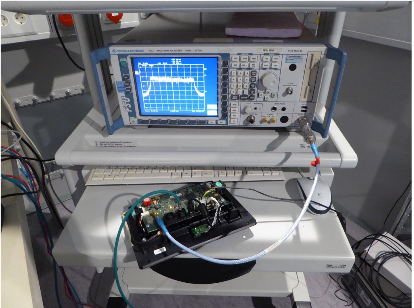
Conducted measurement at antenna port
