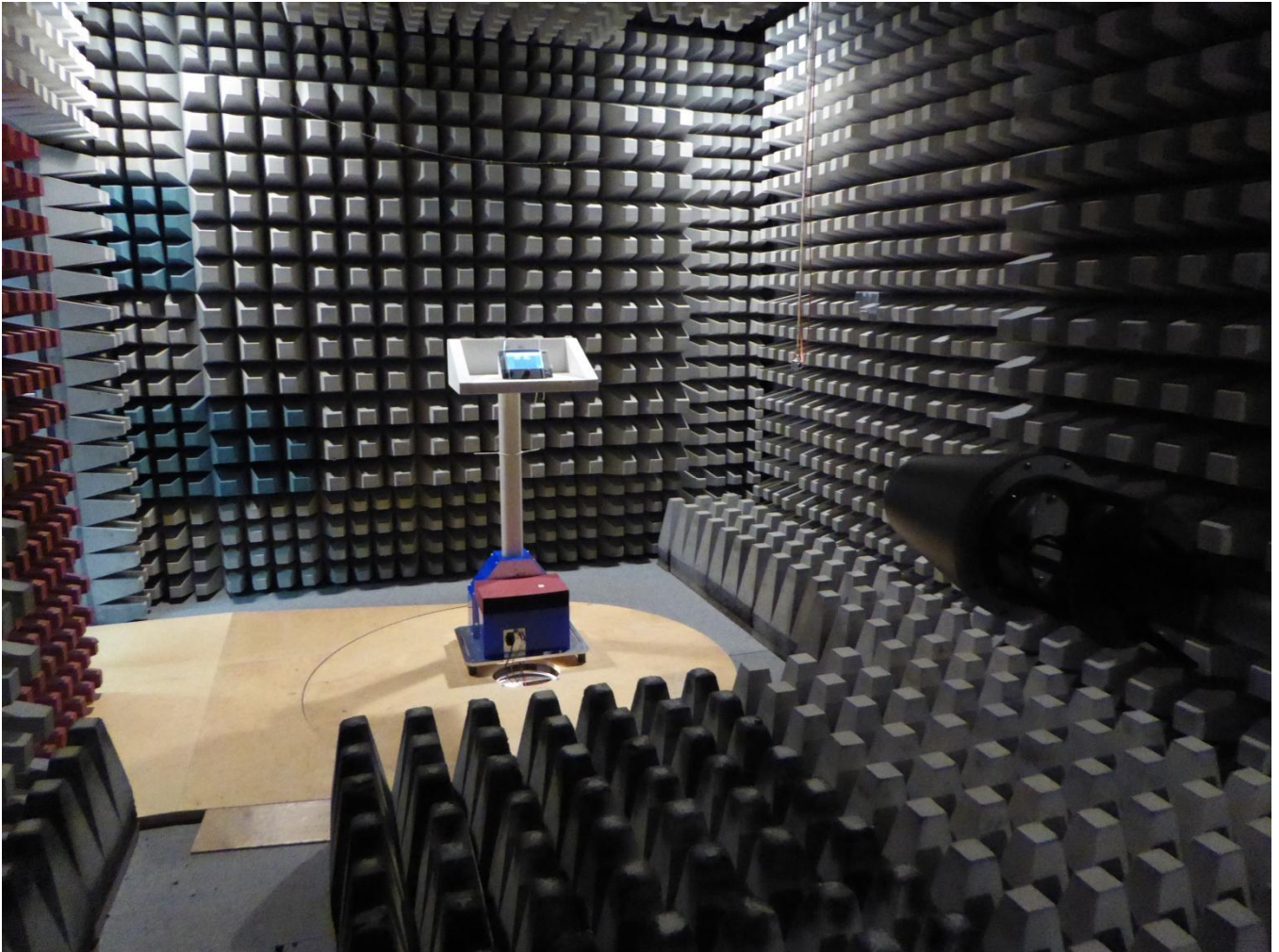
Measurement FAR; 1 - 12 GHz
