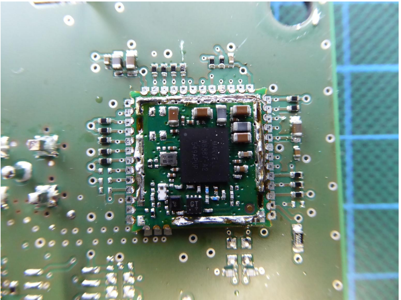
Radio module (WiFi/BLE) shielding removed – detail view
