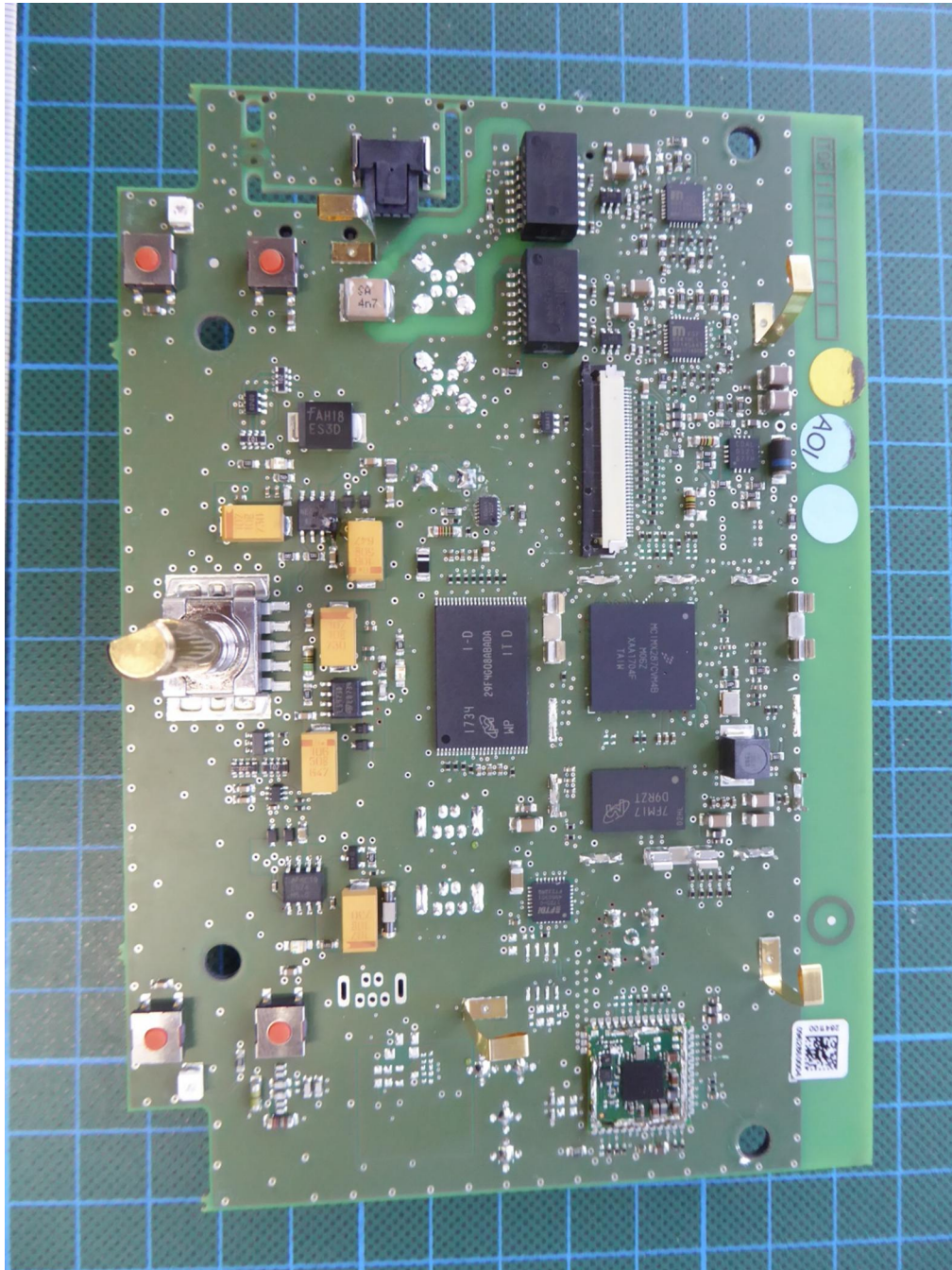
PCB, top view, radio module shielding removed
