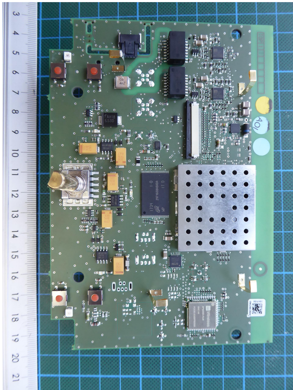
PCB, top view, radio module shielding mounted
