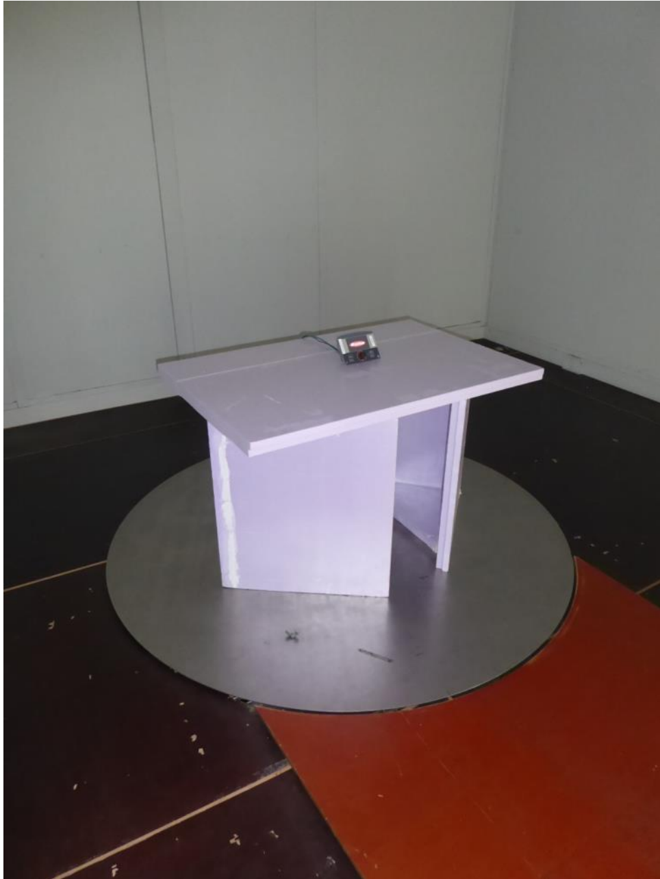
Test setup OATS Final measurement 30 MHz – 1 GHz
