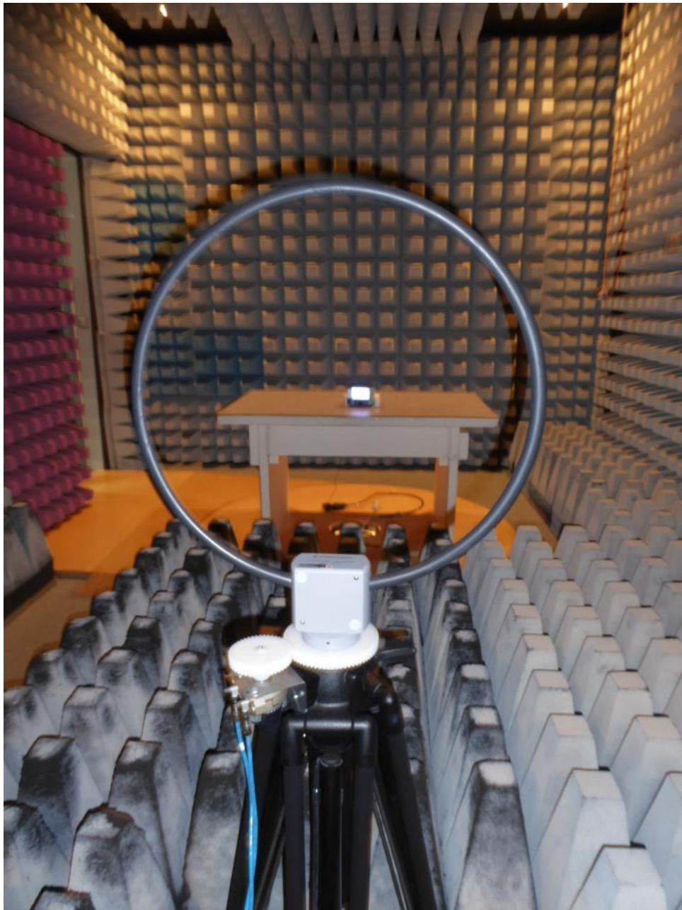
Test setup fully anechoic chamber Preliminary measurement 9 kHz – 30 MHz
